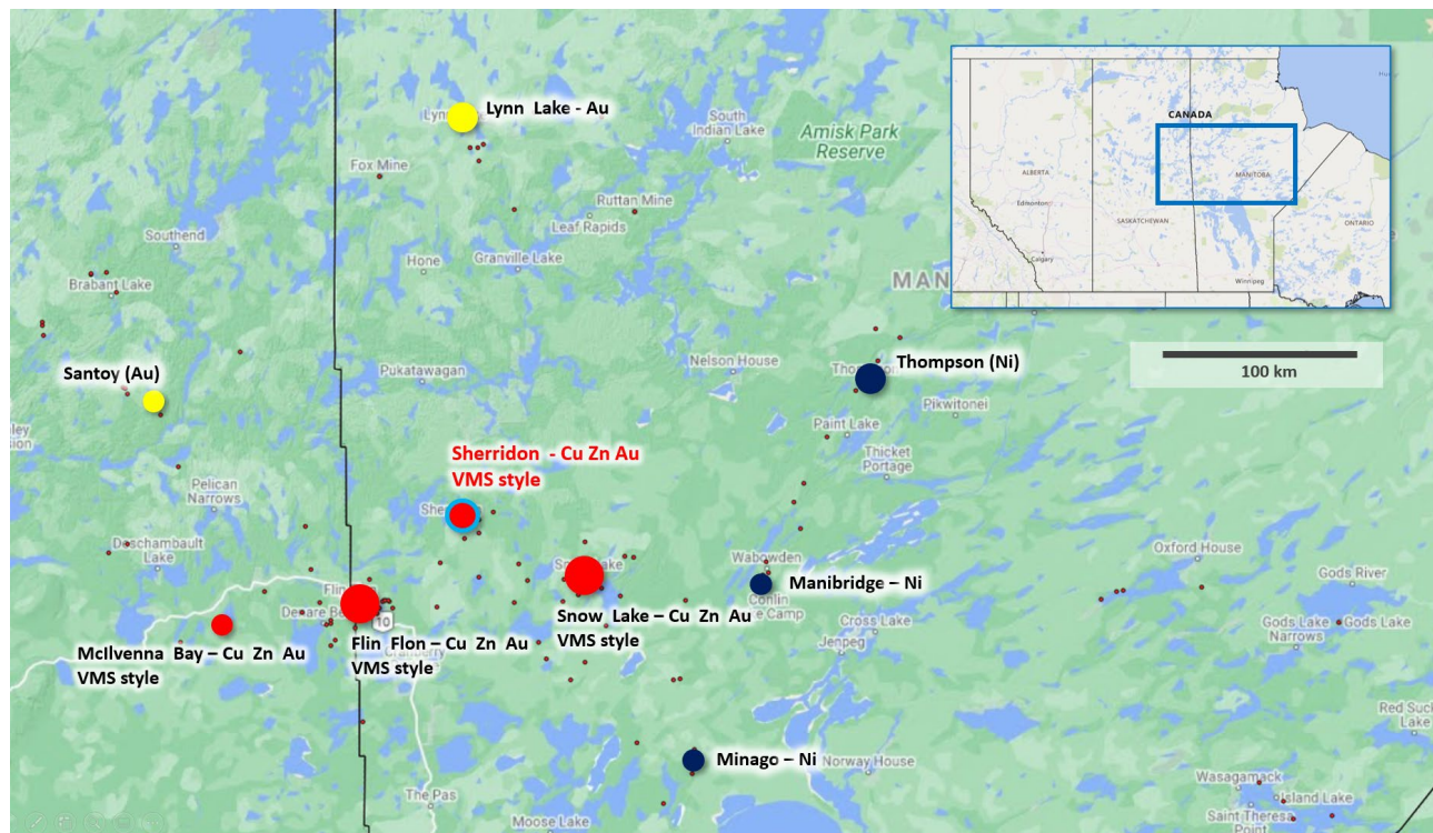
Figure 1: Location map for the Sherridon copper district in central western Manitoba, Canada. Other significant mines, deposits and mineral districts shown.
