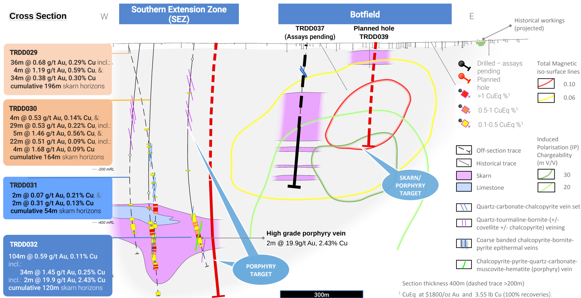
Figure 2: The Botfield prospect is interpreted to be an uplifted block to the adjacent Southern Extension Zone (SEZ) discovery Large magnetic complex coincident with shallow copper-gold and chargeability anomaly is indicative of a large untested skarn &/or porphyry complex
