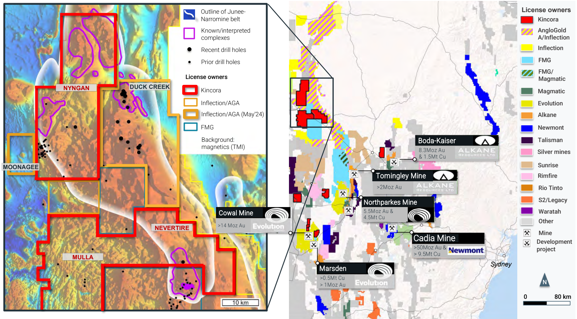
Figure 1: The Macquarie Arc is a proven Tier 1 terrane and Australia's foremost copper porphyry belt hosting a number of world-class mines The Northern Junee-Narromine Belt (NJNB) is an untested district of the Macquarie Arc situated under the post-mineral cover
