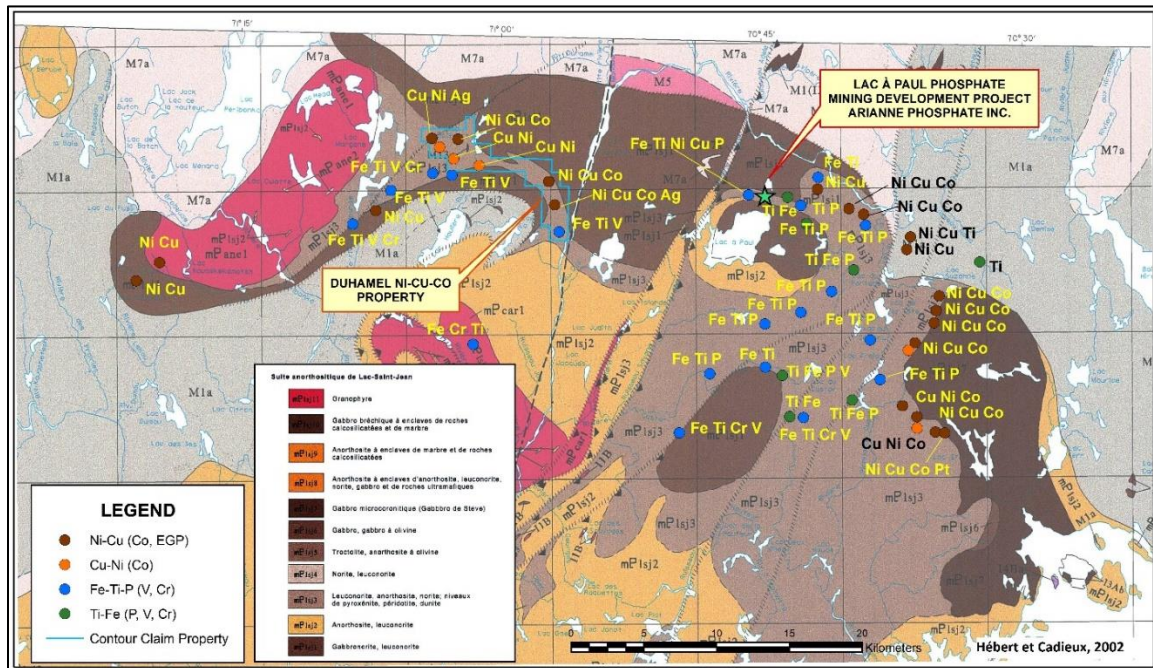
Figure 3. Ni-Cu-Co and Fe-Ti-P-V mineral occurrences on the Chute-des-Passes and Pipmuacan Areas (modified from Hébert et Cadieux, 2002)
