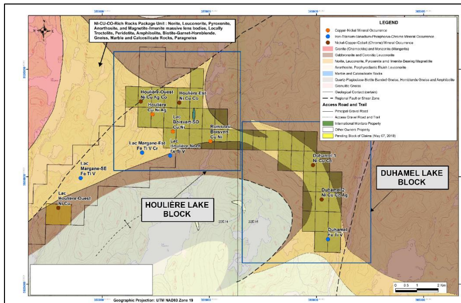
Figure 4. Cu-Ni-Co and Fe-V-Ti-Cr mineral occurrences in Houliere-Duhamel property (Modified from SIGEOM, 2023)
