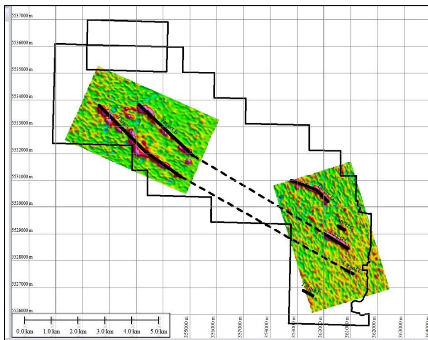
Figure 2. Late-off time TDEM response anomalies on the Duhamel Ni-Cu-Co Property.
