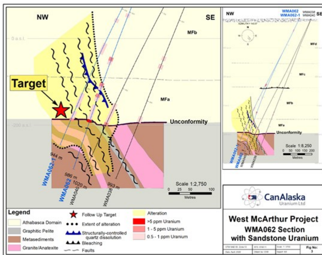
Figure 3 - Uranium geochemistry associated with wide structural zone and alteration halo 1,800 m to the southwest of the "42 Zone"
