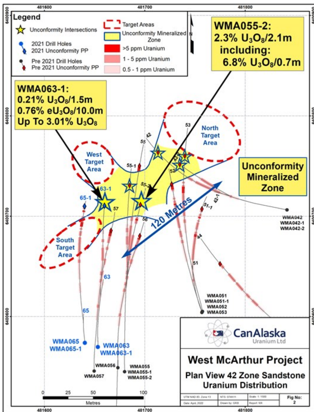
Figure 2 - West McArthur Project Plan View 42 Zone Sandstone Uranium Distribution
