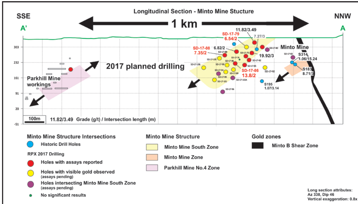
Figure 2. Longitudinal section showing drilling intersections in the Minto Mine Structure between the former Minto and Parkhill mines
