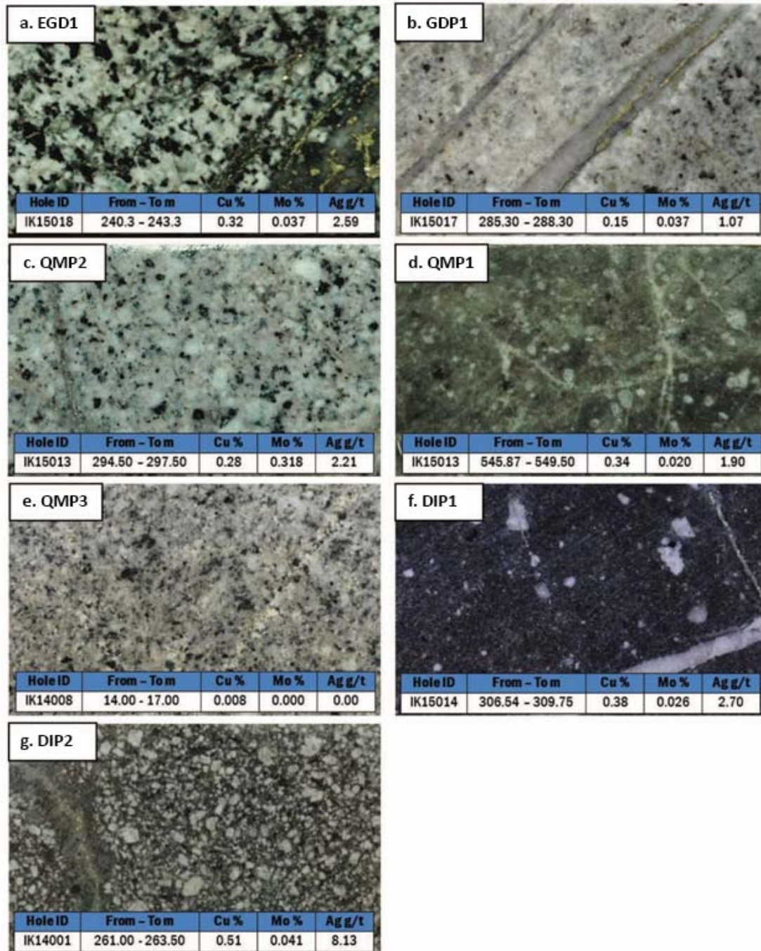
Figure 7-5: Lithological Plates From the IKE Deposit. a. Biotite-bearing Hornblende Granodiorite (EGD1); b. Porphyritic, Hornblende-Bearing, Biotite Granite to Granodiorite (GDP1); c. Porphyritic Hornblende-Bearing, Biotite Quartz-Monzonite to Granodiorite (QMP2); d. Porphyritic Biotite Monzodiorite to Diorite (QMP1); e. Porphyritic Hornblende-Bearing, Biotite Quartz-Monzonite (QMP3); f. Porphyritic Diorite (DIP1); g. Hornblende Diorite Porphyry (DIP2)QMP3 is a porphyritic hornblende-bearing biotite quartz-monzonite and is texturally similar to QMP2 but can be distinguished by its finer grain size and seriate texture (Figure 7-5e). Phenocrysts comprise up to 6% rounded quartz phenocrysts 1-2 mm in size, up to 35% euhedral, lath-like plagioclase phenocrysts 1-3 mm in size, up to 5% euhedral biotite 1-3 mm in size, and trace 1 mm prismatic hornblende. The grain size of the groundmass is typically < 1 mm.
