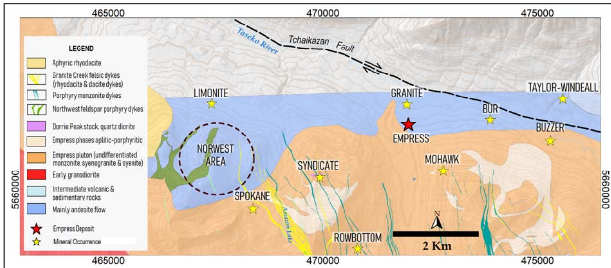
Figure 7-7: Amarc GECAP Surface Geology.
