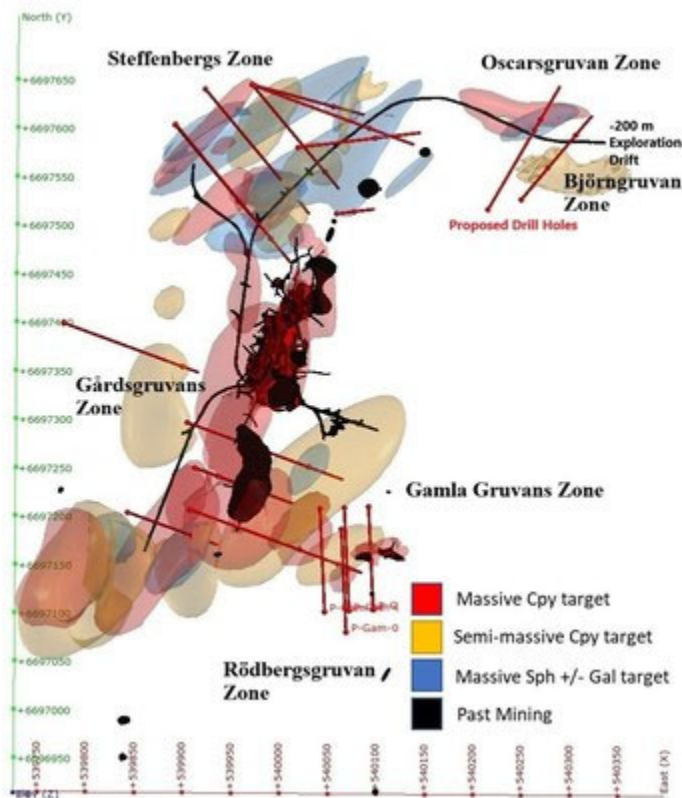
Figure 1: Plan View of Mineralized Zones at Tomtebo Mine (CNW Group/District Metals Corp.)
