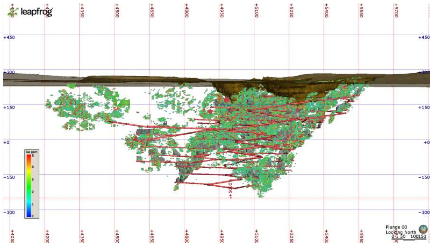
FIGURE 1 - LONG SECTION OF BLOCK MODEL – CUT OFF 1.5G/T
