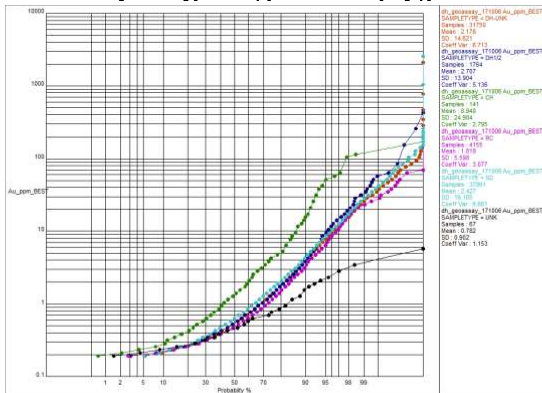
Figure 3. Log probability plot different sampling types
