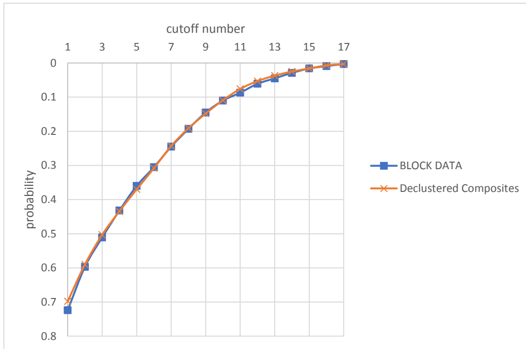
Figure 4. CCDF Validation Curves Medium Grade Group
