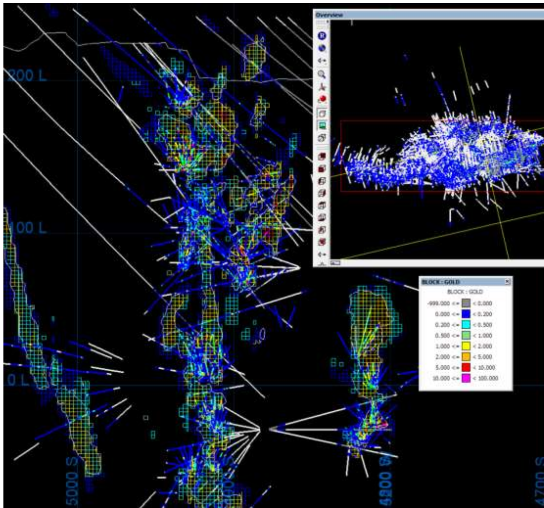
Figure 5. Typical sectional view displaying localised Au grades
