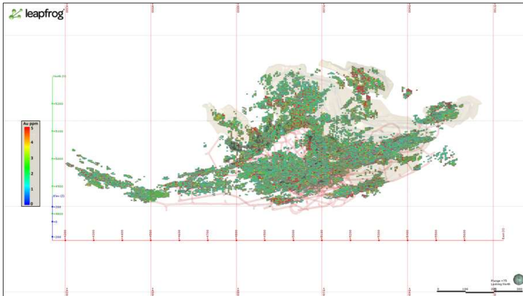
FIGURE 2 – PLAN VIEW OF BLOCK MODEL – CUT OFF 1.5G/T
