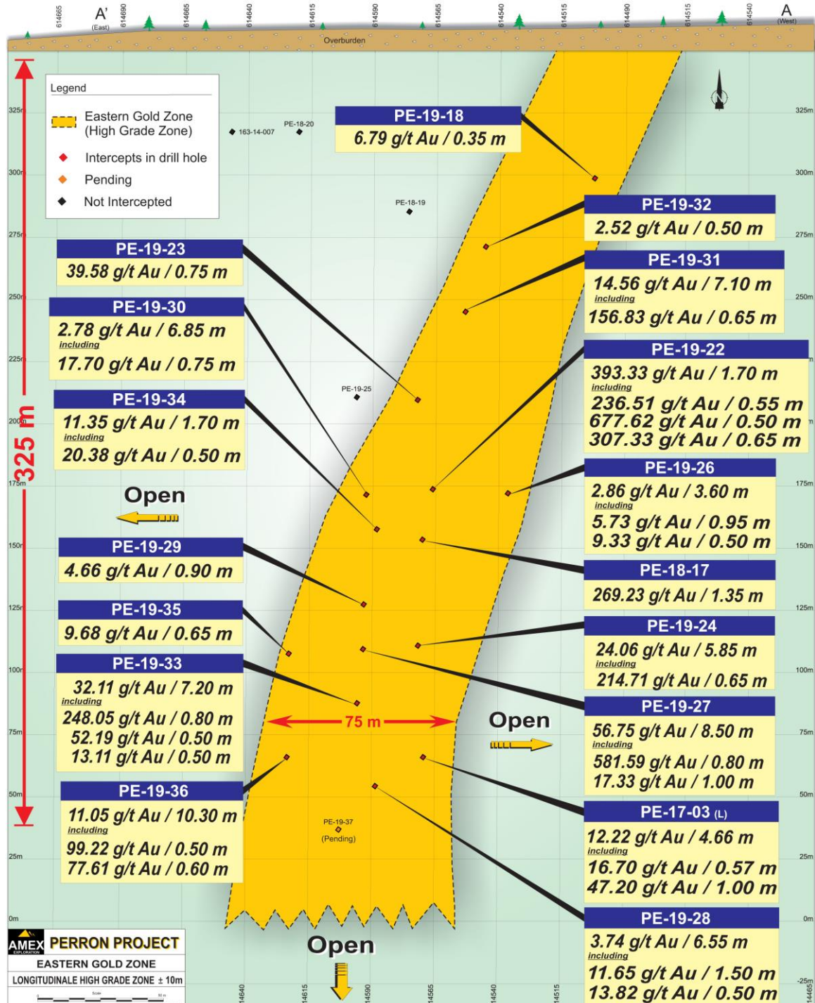
FIGURE 2: Longitudinal of the High Grade Zone
