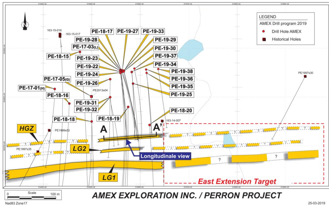
FIGURE 1: Plan Map of Drilled Hole Locations EASTERN GOLD ZONE DRILL PROGRAM 2019
