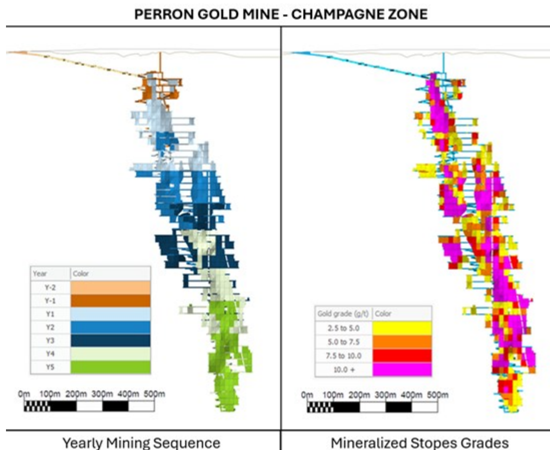
Figure 1: Mine Plan Design looking north.
