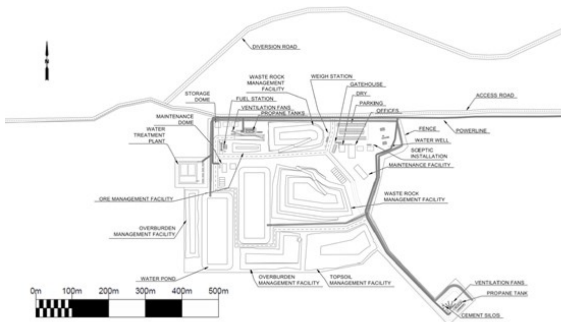
Figure 2: Suggested Infrastructure Arrangement
