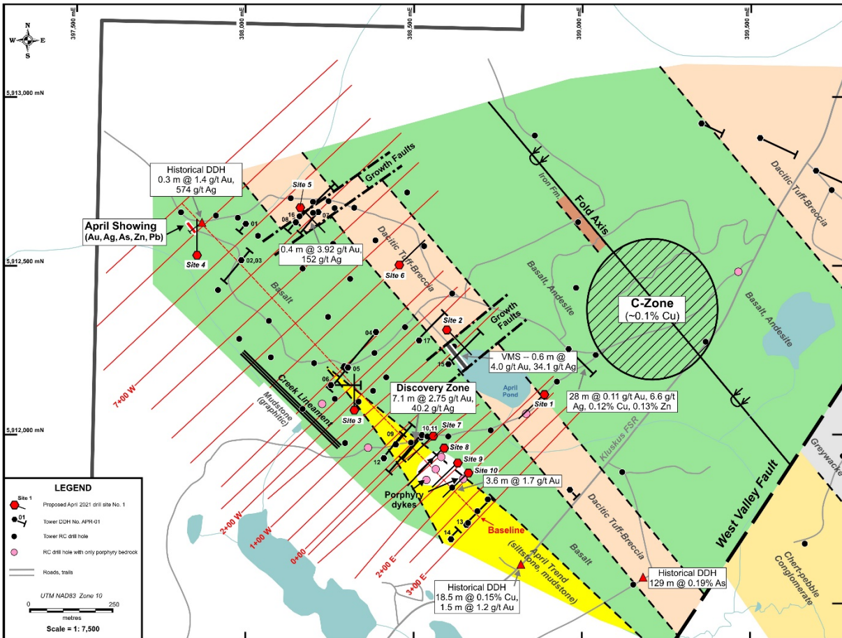
Figure 2 – Proposed sites and geological targets of the first ten drill holes of the planned eighteen-hole drill program. The first six sites are scout holes to guide the placement of some of the remaining holes. Sites 7 to 10 are designed to extend the Discovery Zone along strike and to depth.
