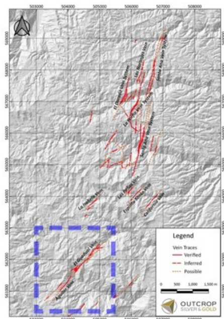
Map 2. Twelve kilometres strike of mapped veins zones at Santa Ana permitted for drilling. Reconnaissance mapping and prospecting suggest Aguilar could be part of a 1.5-kilometre-wide vein corridor, similar to the Royal Santa Ana veins to north, (CNW Group/Outcrop Silver & Gold Corporation)
