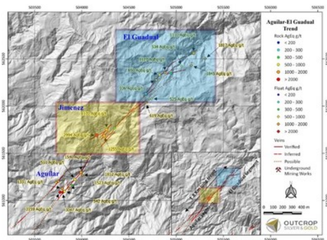
Map 1. The Aguilar-El Guadual trend can be traced for 1.8 kilometres in outcrop and float. This area is highlighted on Map 2, (CNW Group/Outcrop Silver & Gold Corporation)
