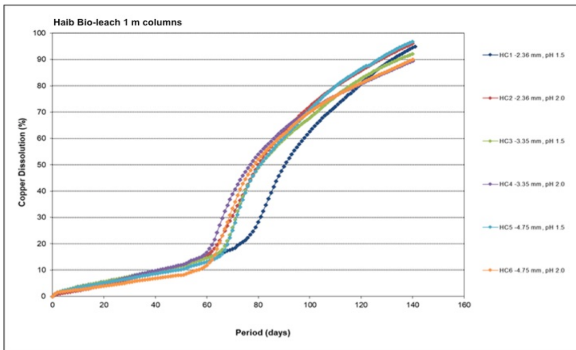
Figure 1. Columns copper dissolution profiles
