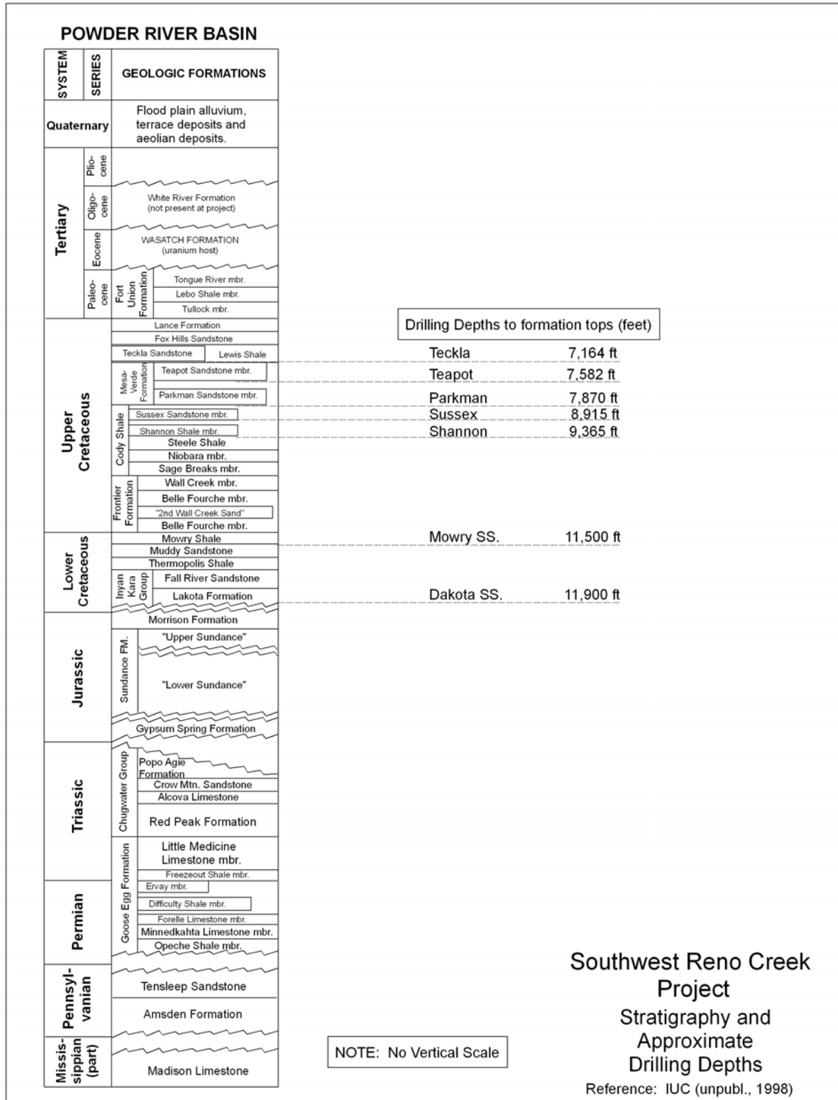
Figure 7-1 Southwest Reno Creek Property: Powder River Basin Stratigraphic Column
