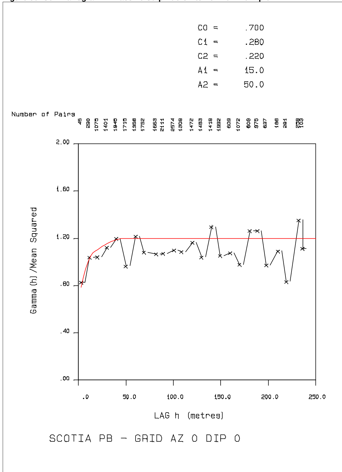
Figure 30: Semivariogram In Massive Sulphide Units for Pb Az 0 Dip 0
