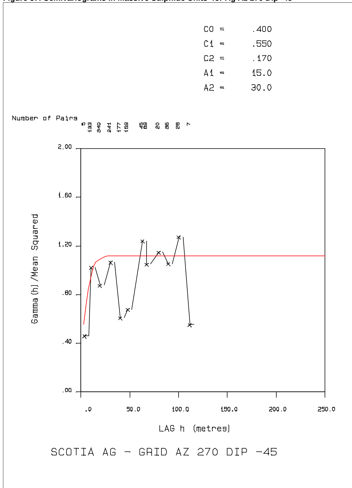
Figure 37: Semivariograms In Massive Sulphide Units for Ag Az 270 Dip -45
