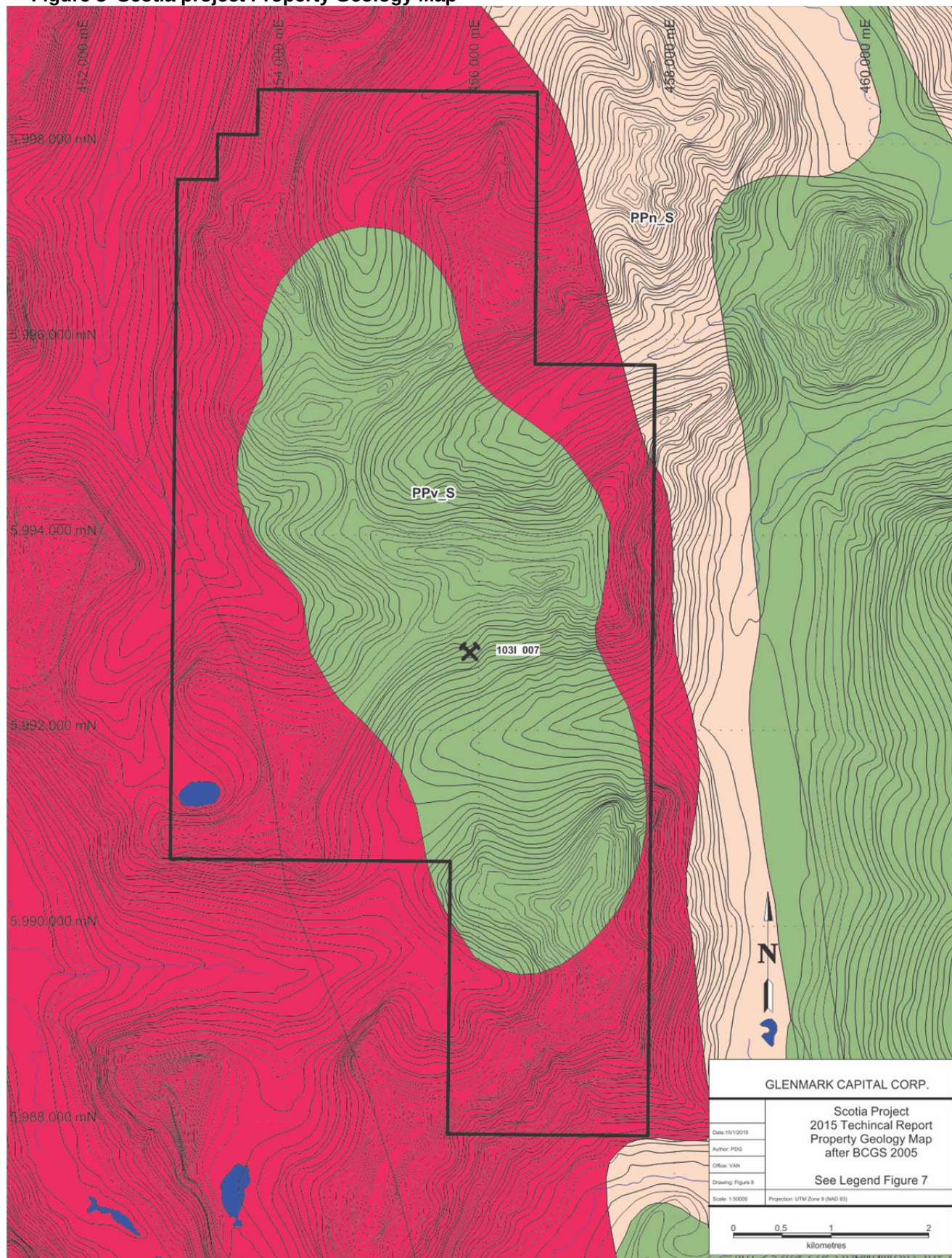
Figure 8 Scotia project Property Geology Map
