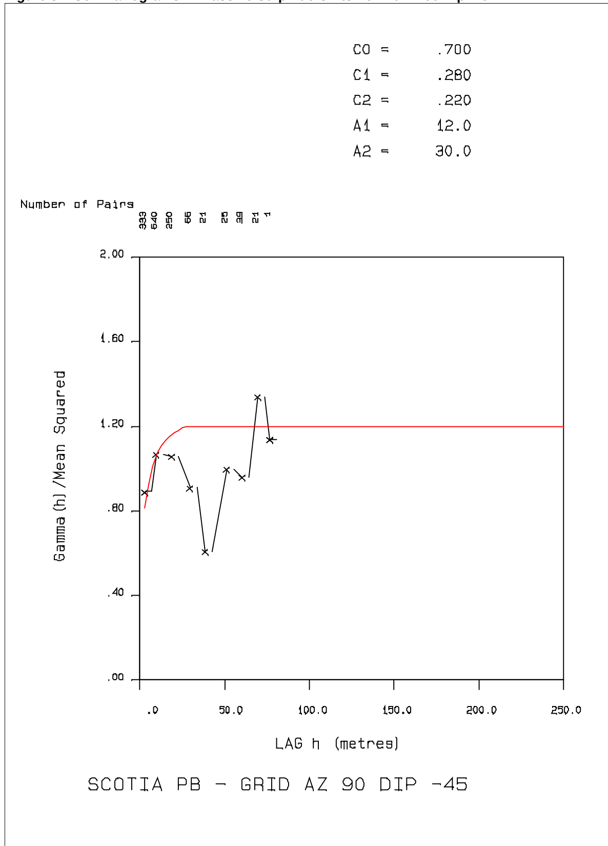
Figure 32: Semivariograms In Massive Sulphide Units for Pb Az 90 Dip -45
