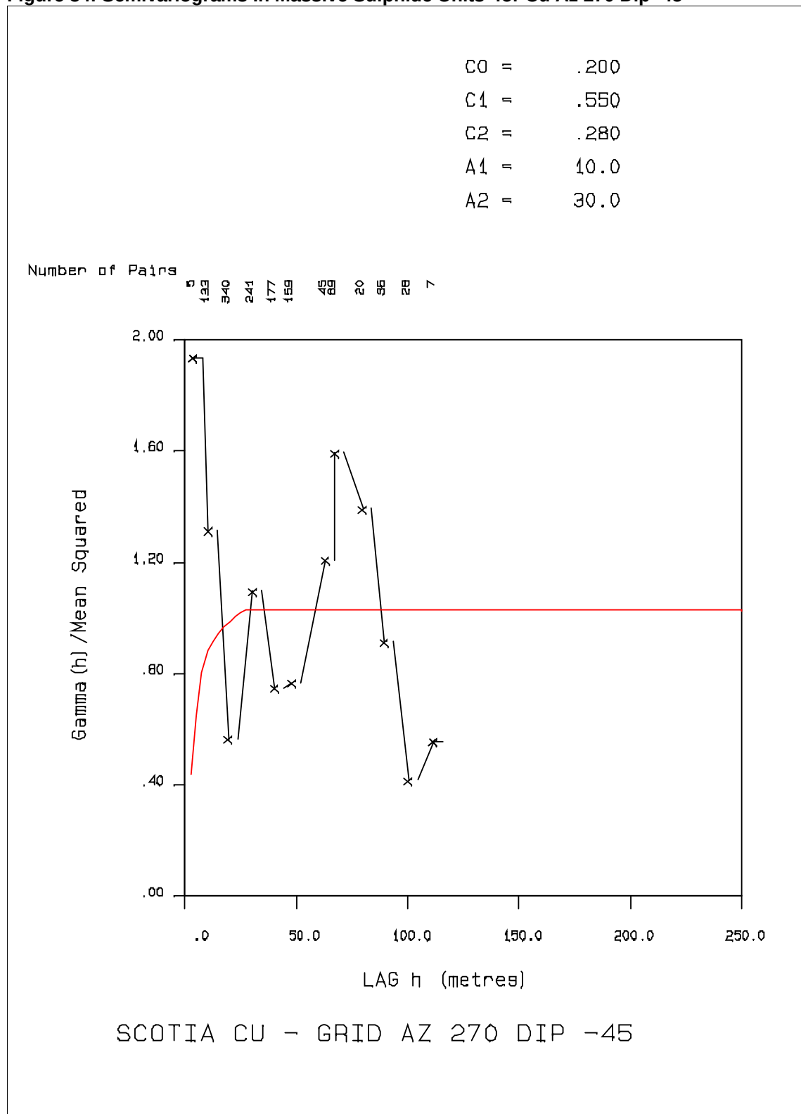
Figure 34: Semivariograms In Massive Sulphide Units for Cu Az 270 Dip -45
