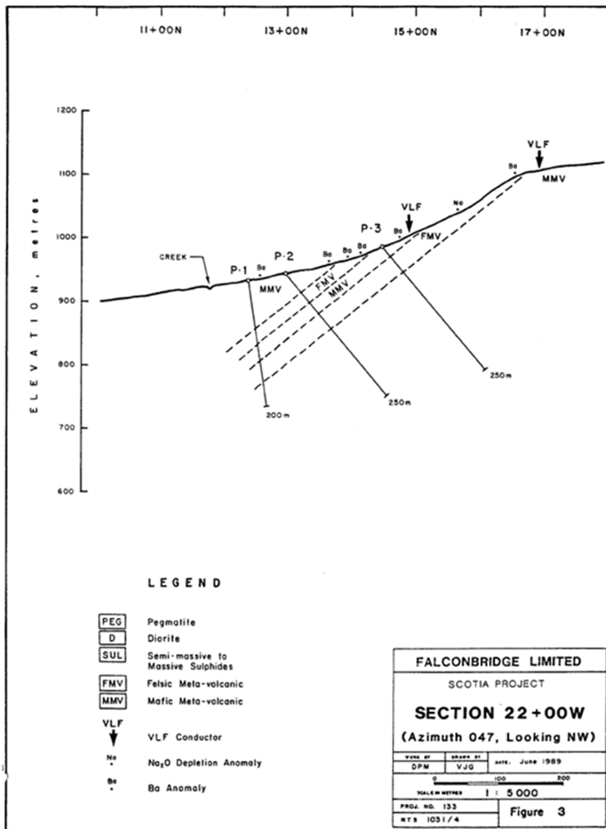
Figure 5 Section 22+00W
