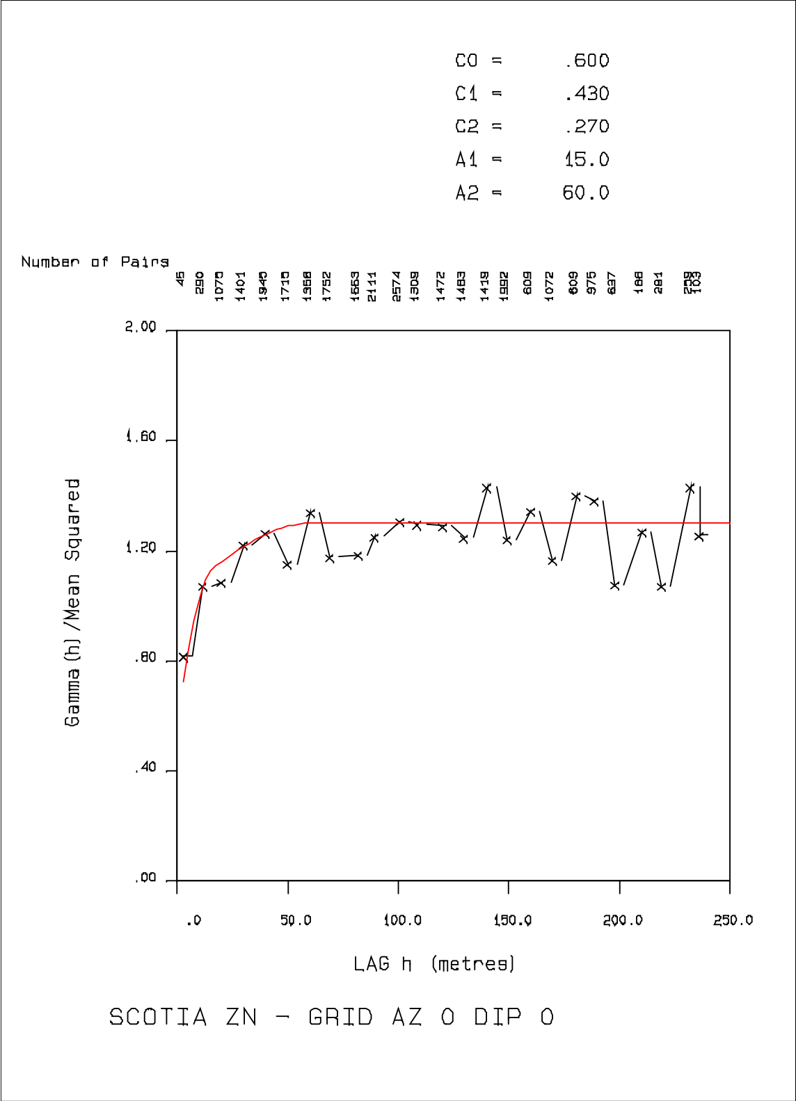
Figure 27: Semivariogram In Massive Sulphide Units for Zn Az 0 Dip 0
