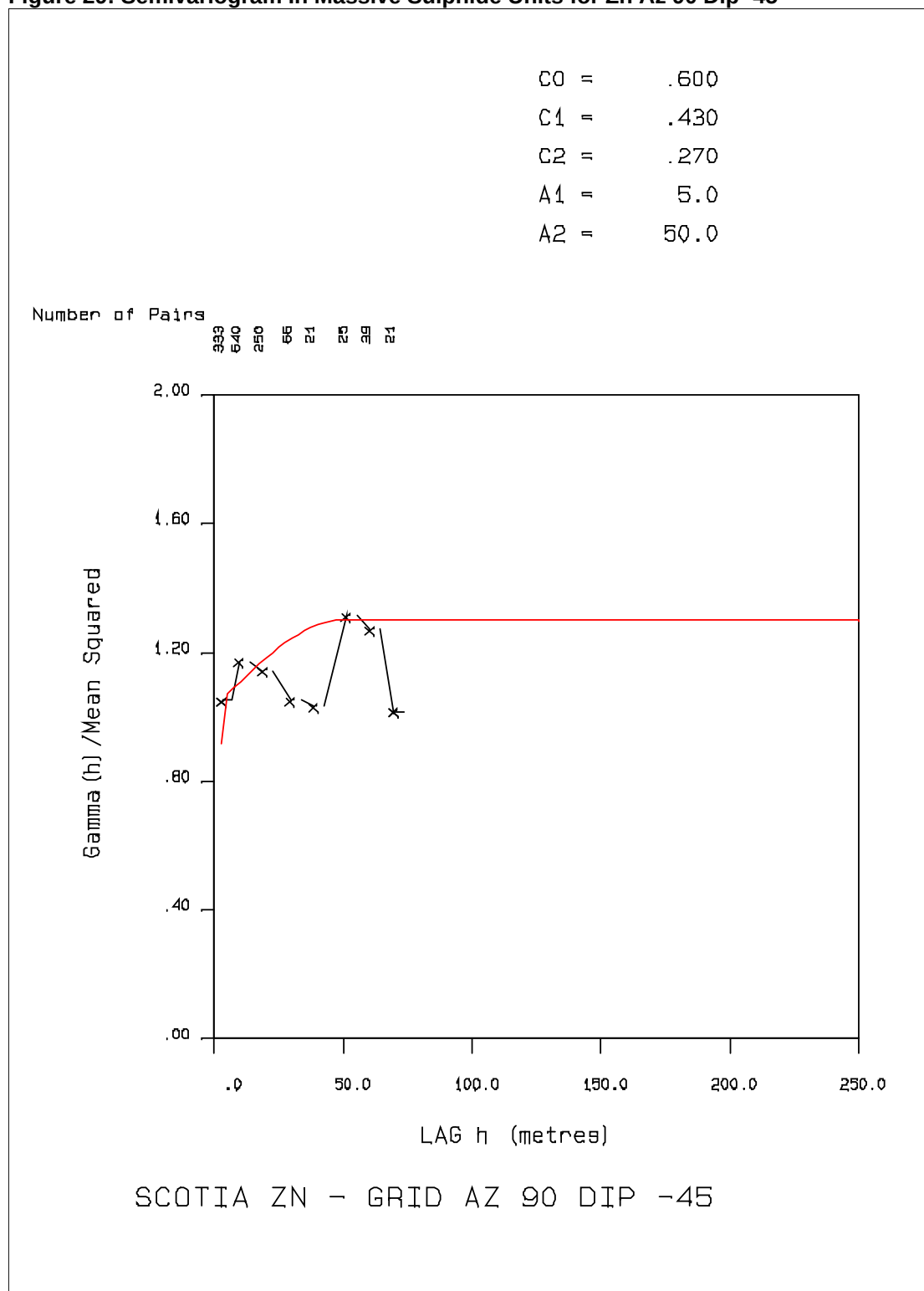
Figure 29: Semivariogram In Massive Sulphide Units for Zn Az 90 Dip -45
