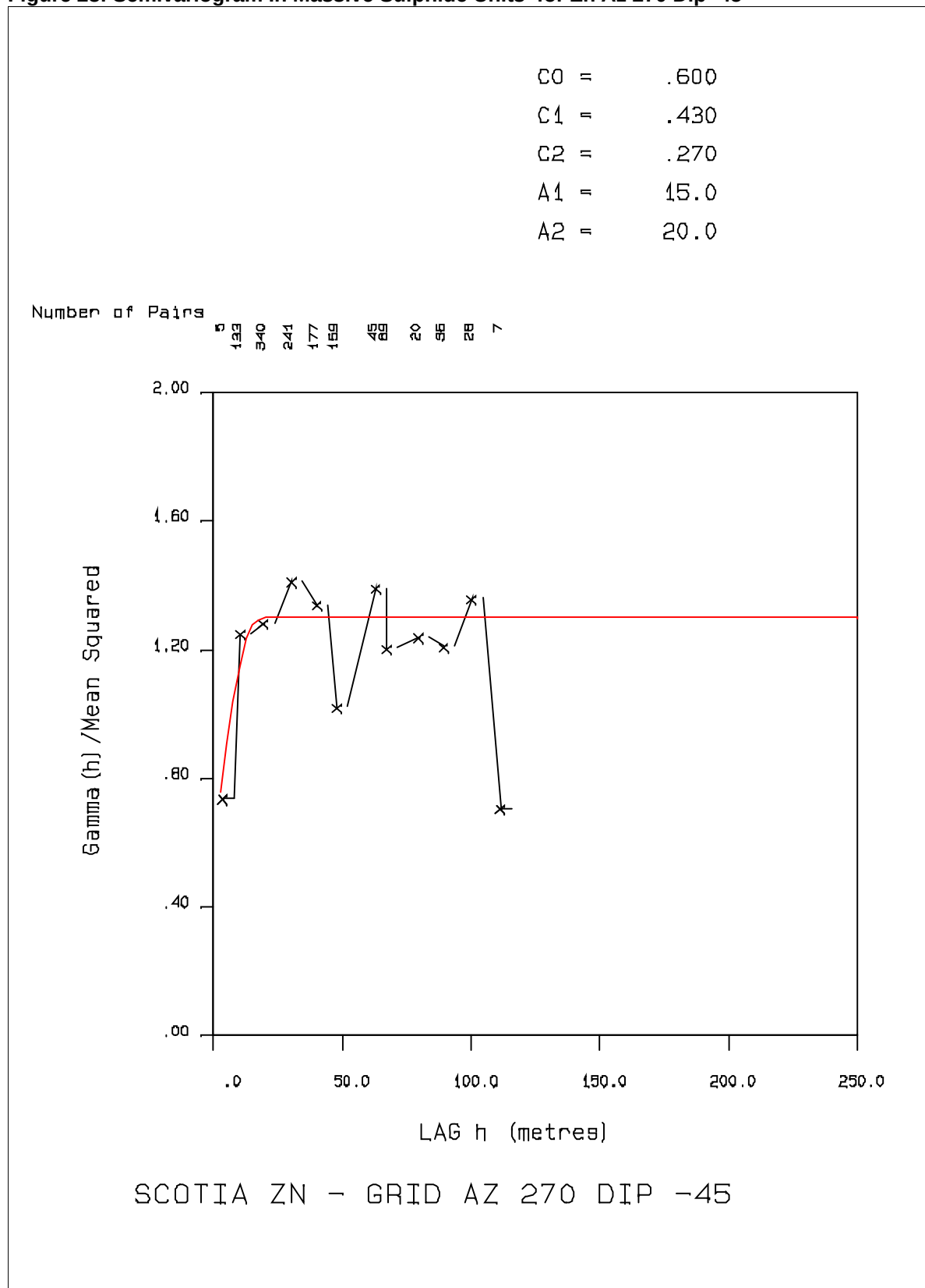
Figure 28: Semivariogram In Massive Sulphide Units for Zn Az 270 Dip -45
