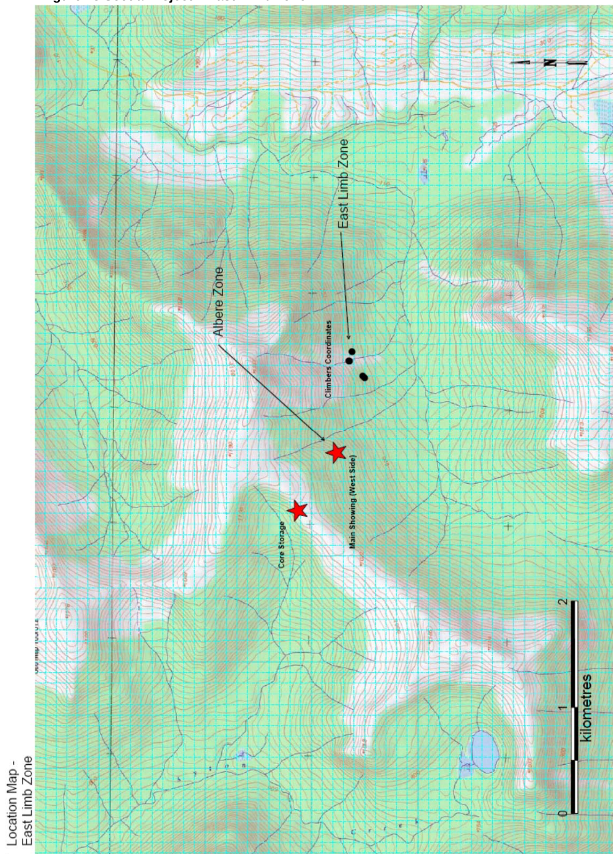
Figure 13 Scotia Project – East Limb Zone
