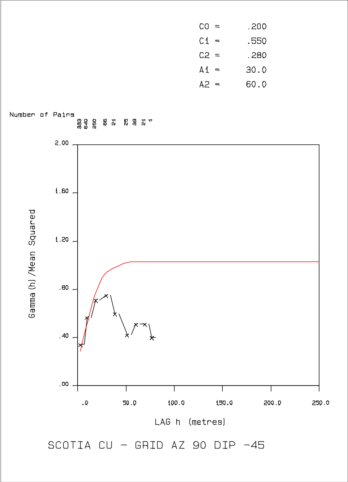
Figure 35: Semivariograms In Massive Sulphide Units for Cu Az 90 Dip -45
