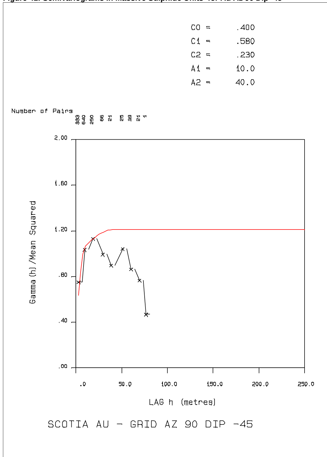
Figure 41: Semivariograms In Massive Sulphide Units for Au Az 90 Dip -45
