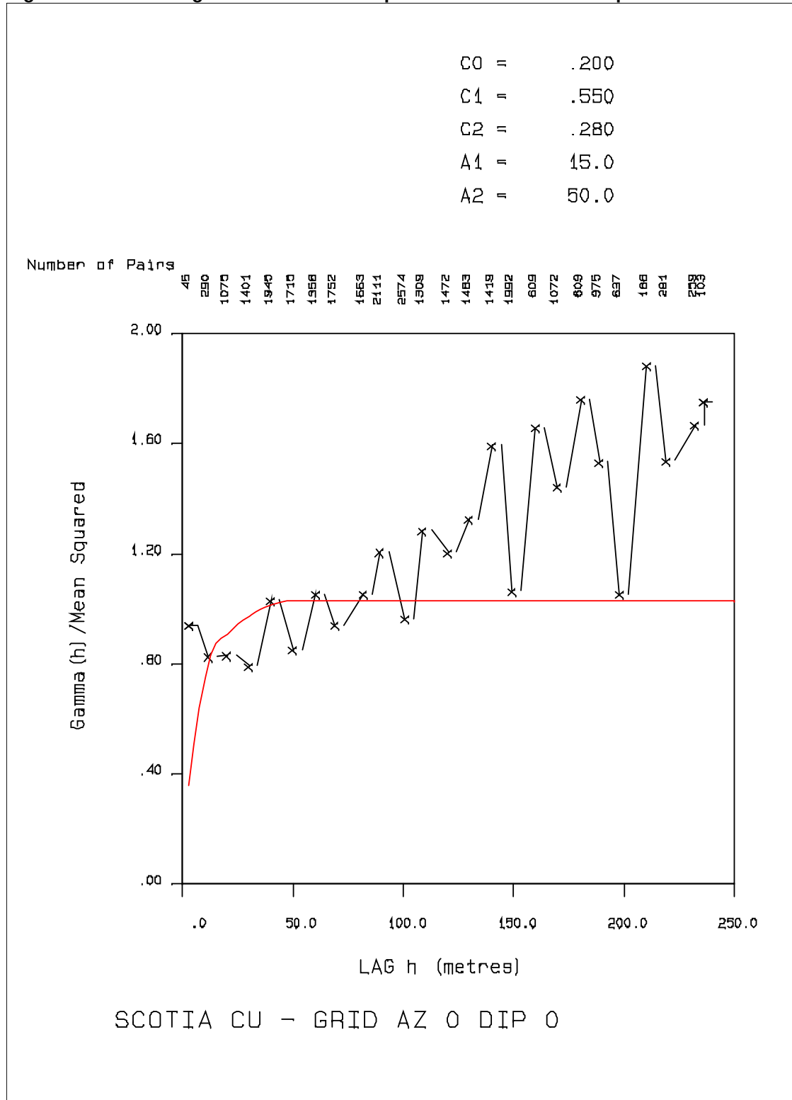
Figure 33: Semivariograms In Massive Sulphide Units for Cu Az 0 Dip 0
