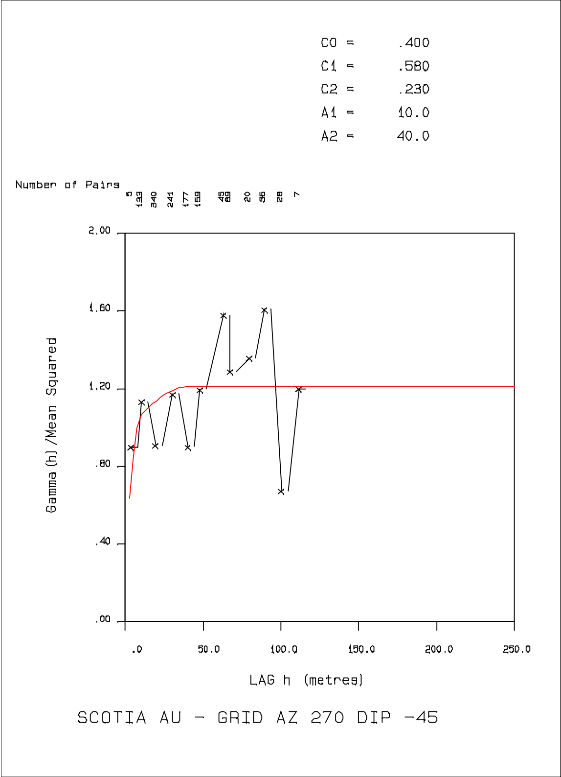
Figure 40: Semivariograms In Massive Sulphide Units for Au Az. 270 Dip -45
