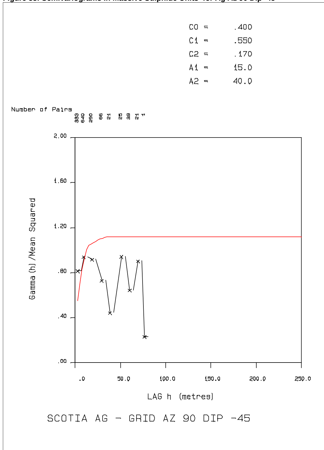
Figure 38: Semivariograms In Massive Sulphide Units for Ag Az 90 Dip -45
