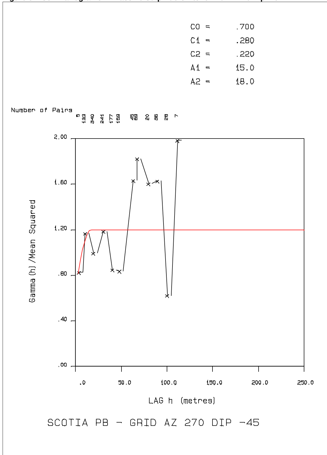
Figure 31: Semivariograms In Massive Sulphide Units for Pb Az 270 Dip -45
