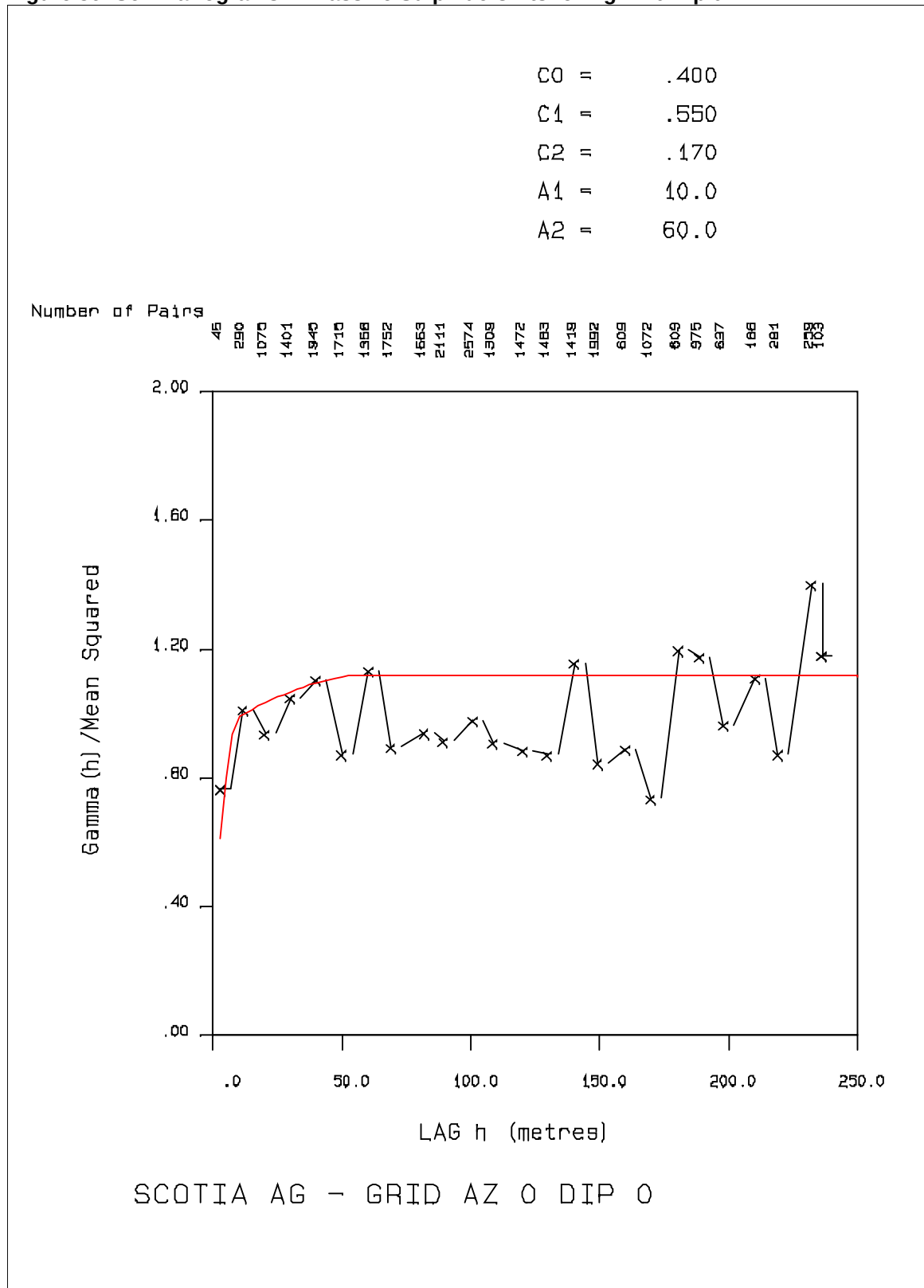
Figure 36: Semivariograms In Massive Sulphide Units for Ag Az 0 Dip 0
