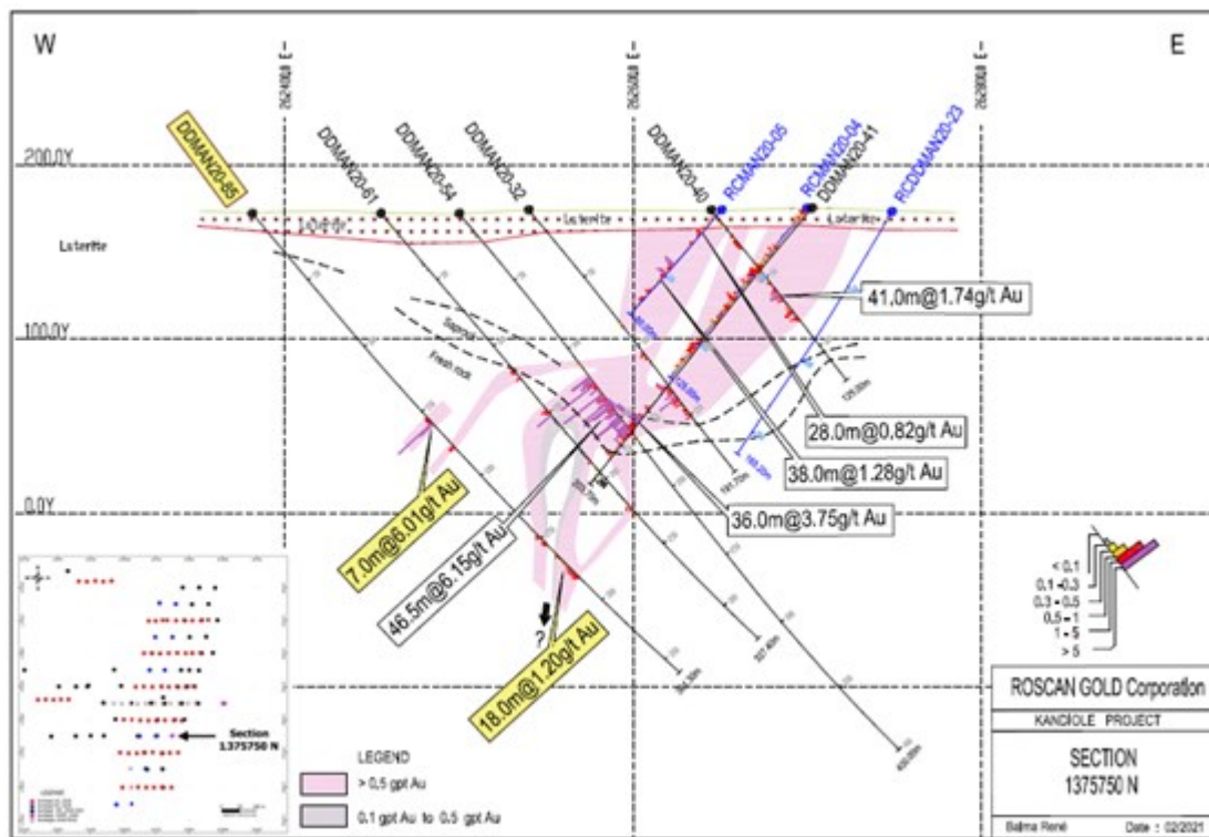
Figure 2: Cross Section Depicting the Extension to Vertical Depth to 220m - DDMAN-20-85
