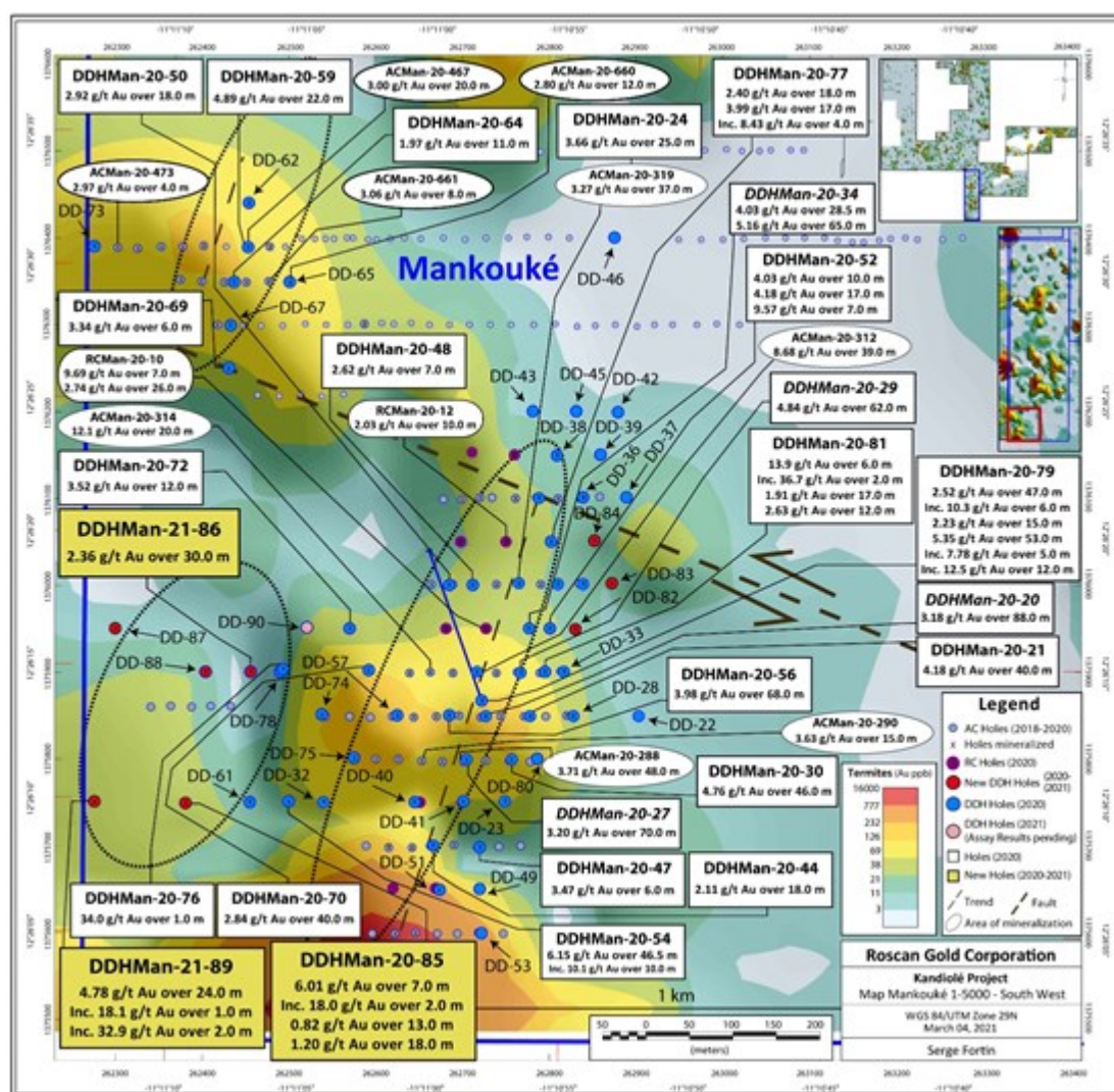
Figure 1: Plan View of the Southern Mankouke Drilling
