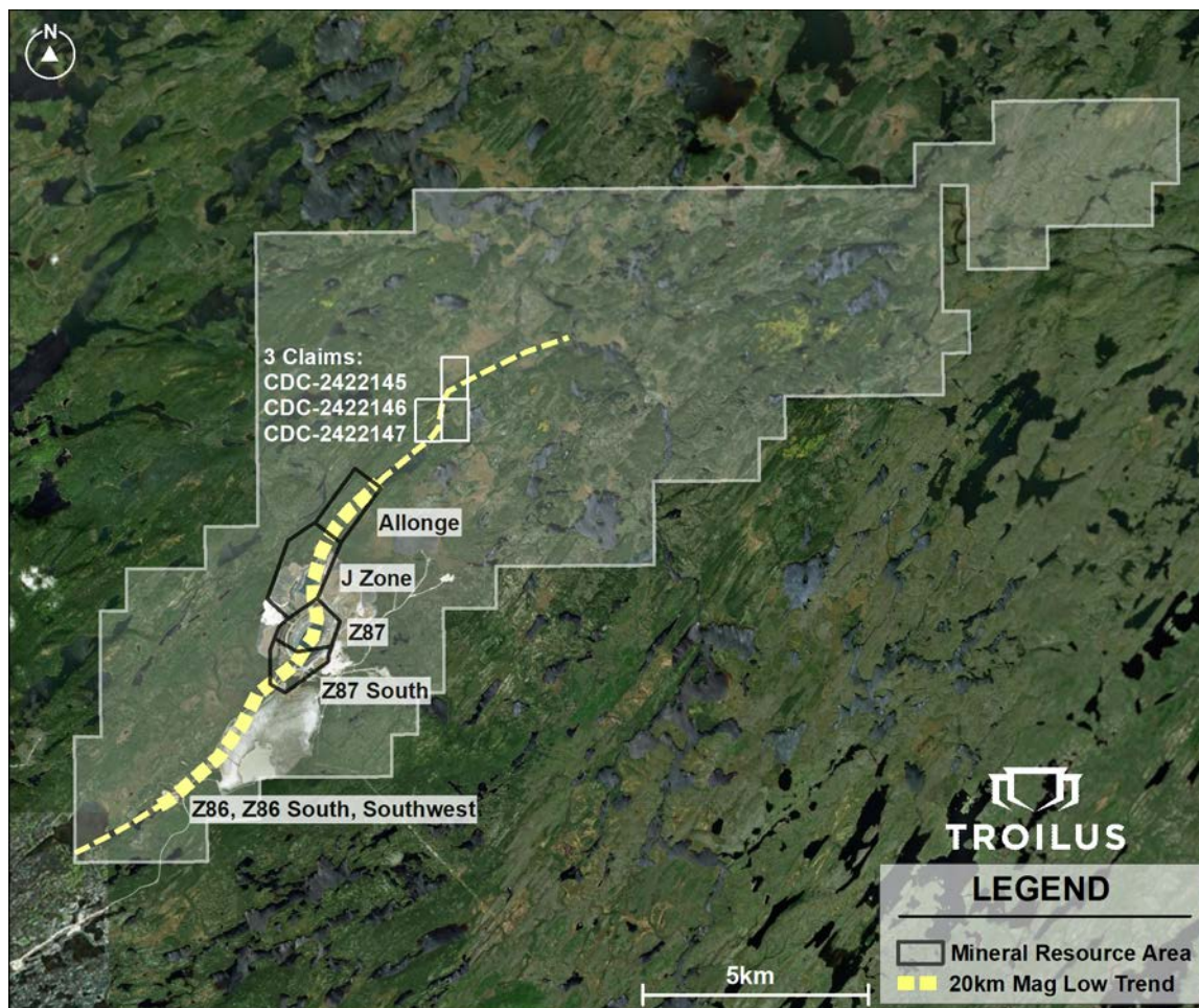
Figure 1: Plan view of Troilus Property Showing new Claims Acquired to the north west of Zone Allonge
