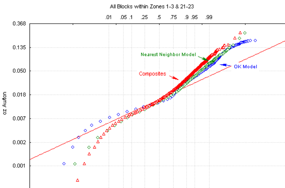
Figure 14.6 Distribution of Block Models and Composites
