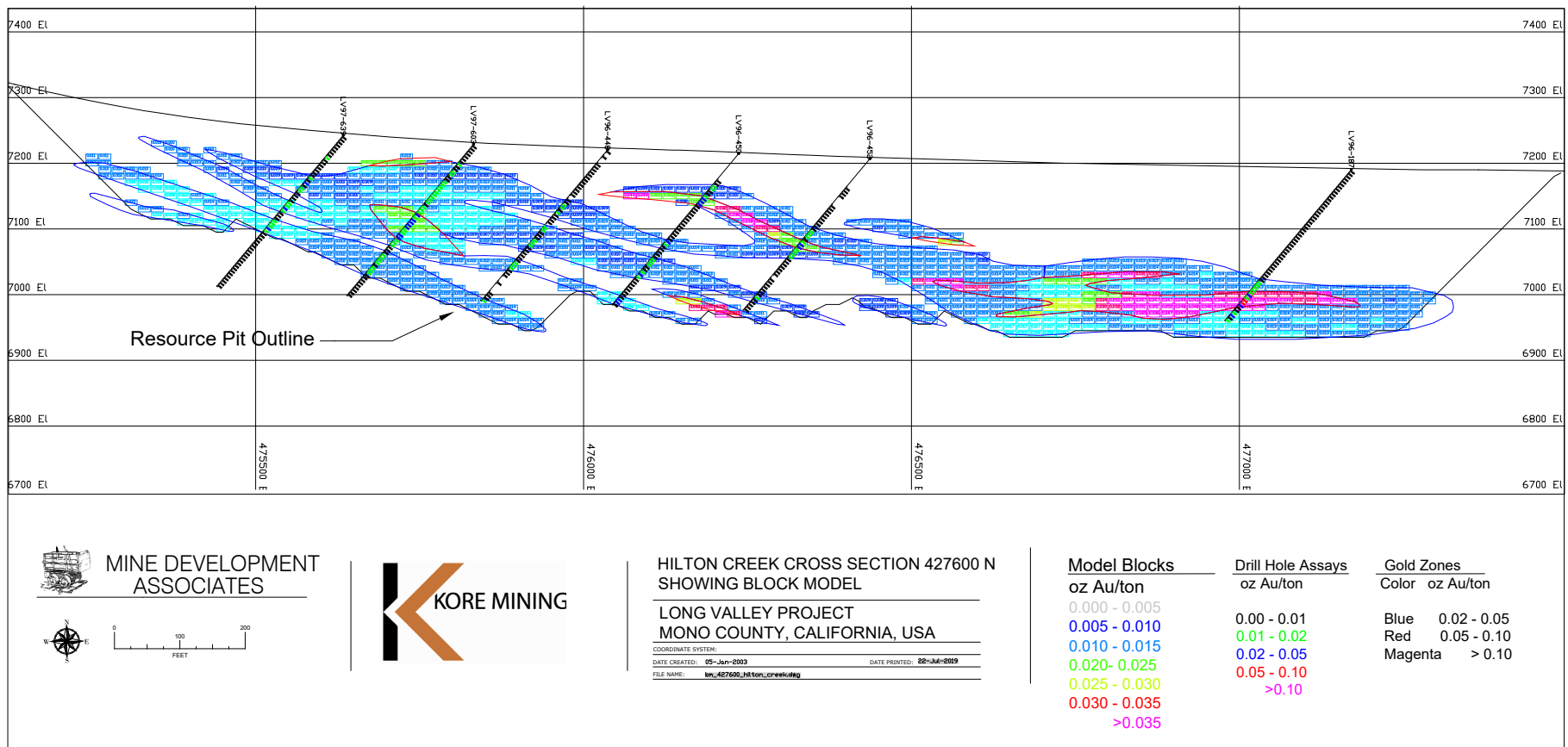
Figure 14.7 Hilton Creek Block Model Section, Looking North
