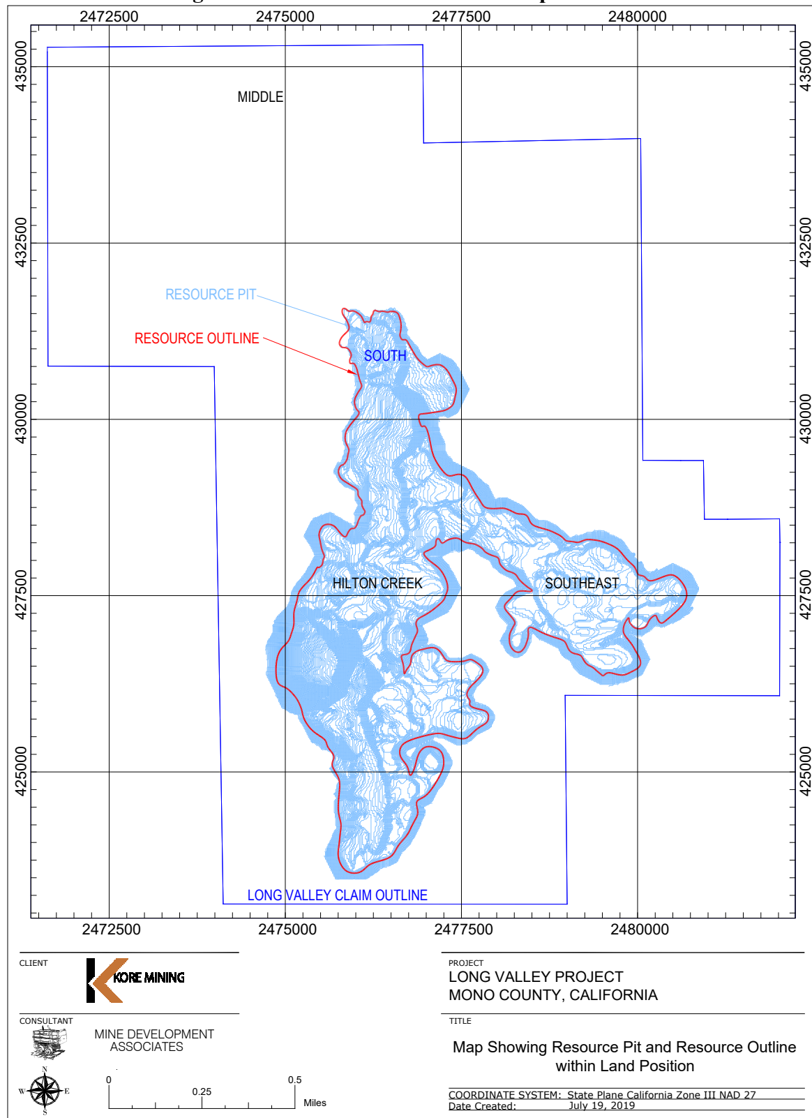
Figure 14.10 Resource Outline with Optimized Pit
