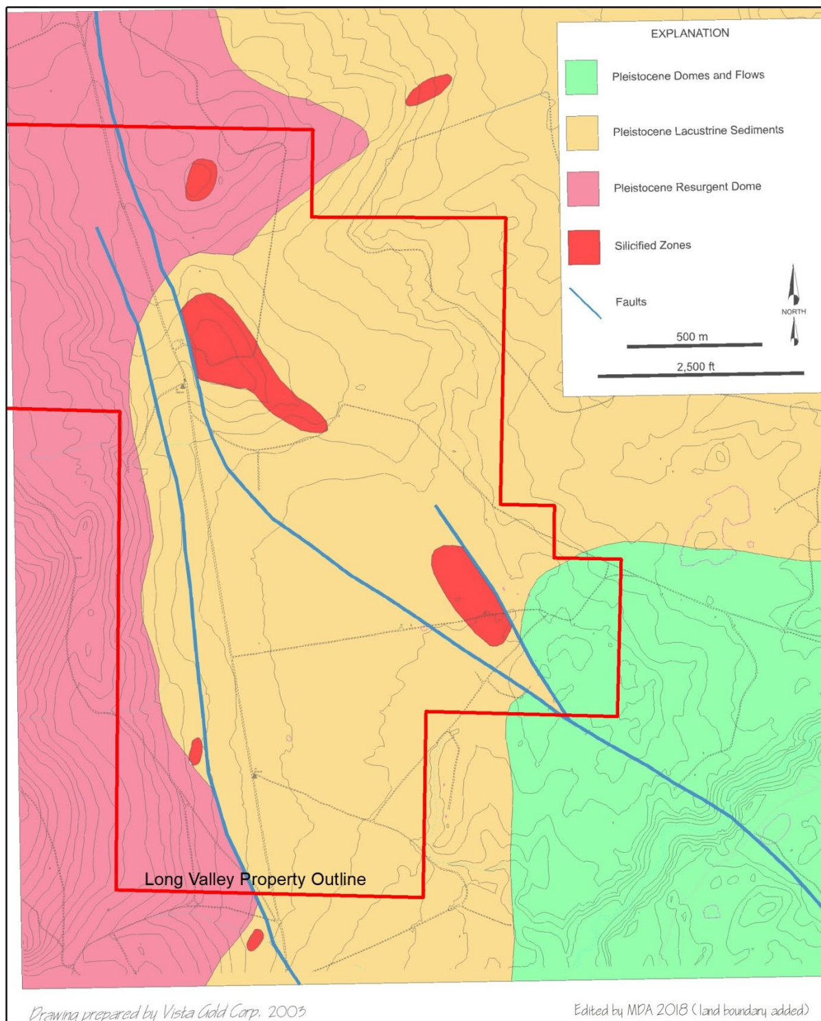
Figure 7.2 Deposit Geology
