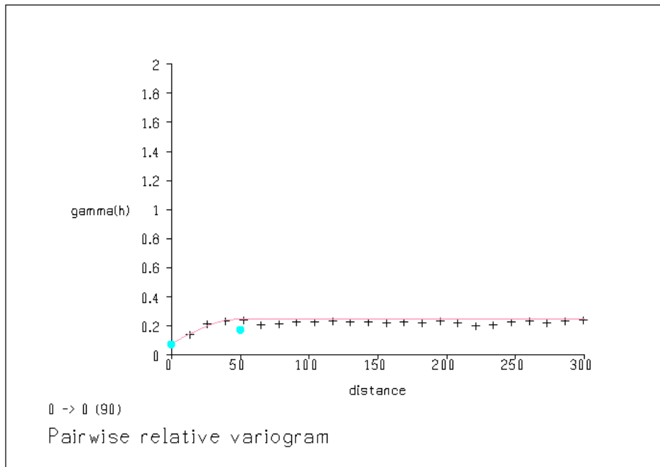
Figure 14.5 Southeast Zone Variogram (Omni-Directional)
