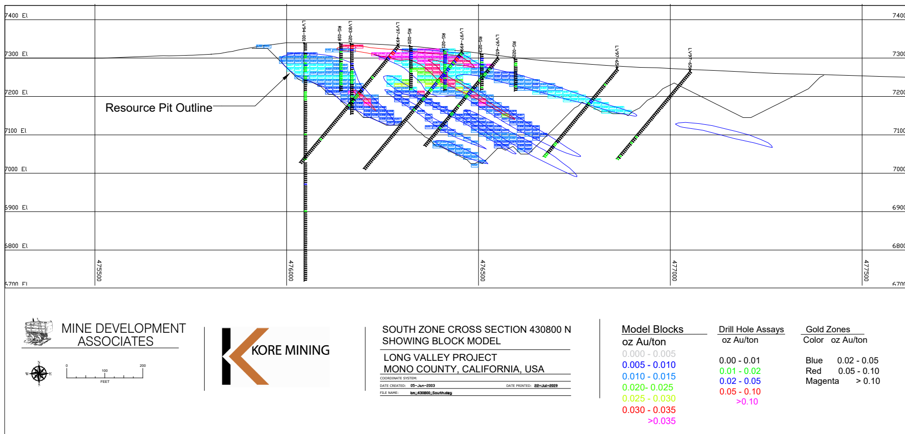
Figure 14.9 South Zone Block Model Cross Section, Looking North
