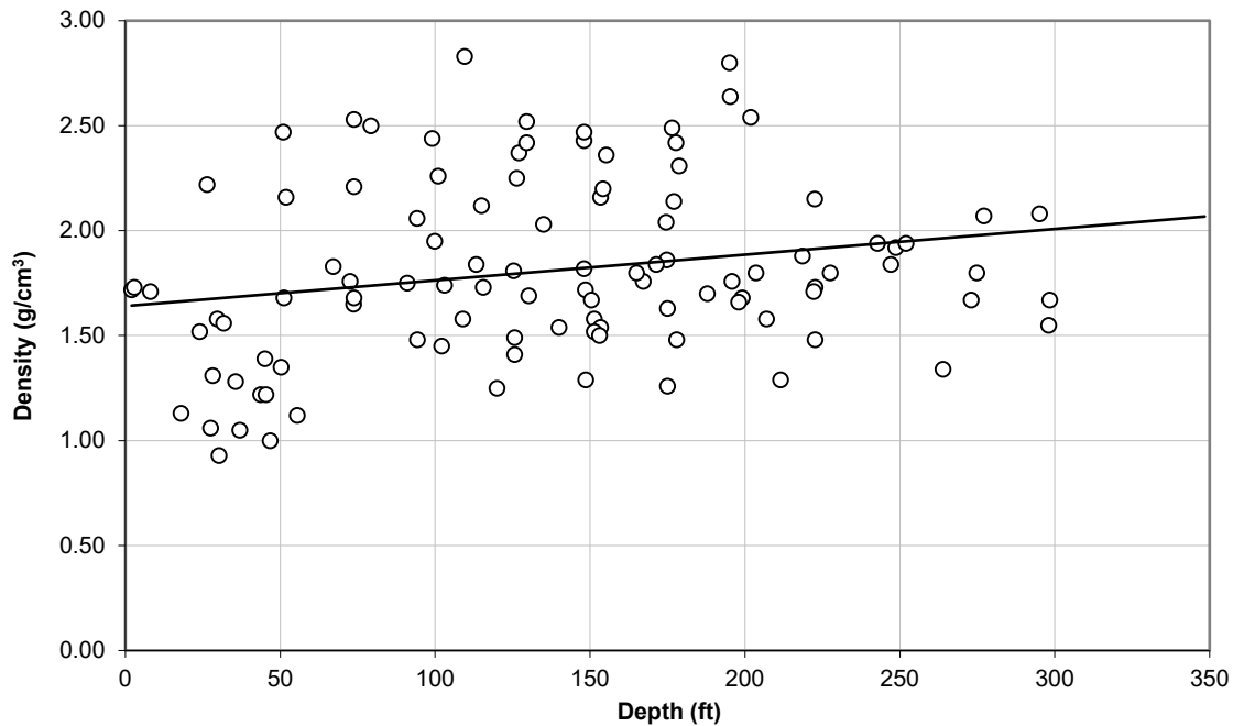
Figure 14.1 Density vs Depth
