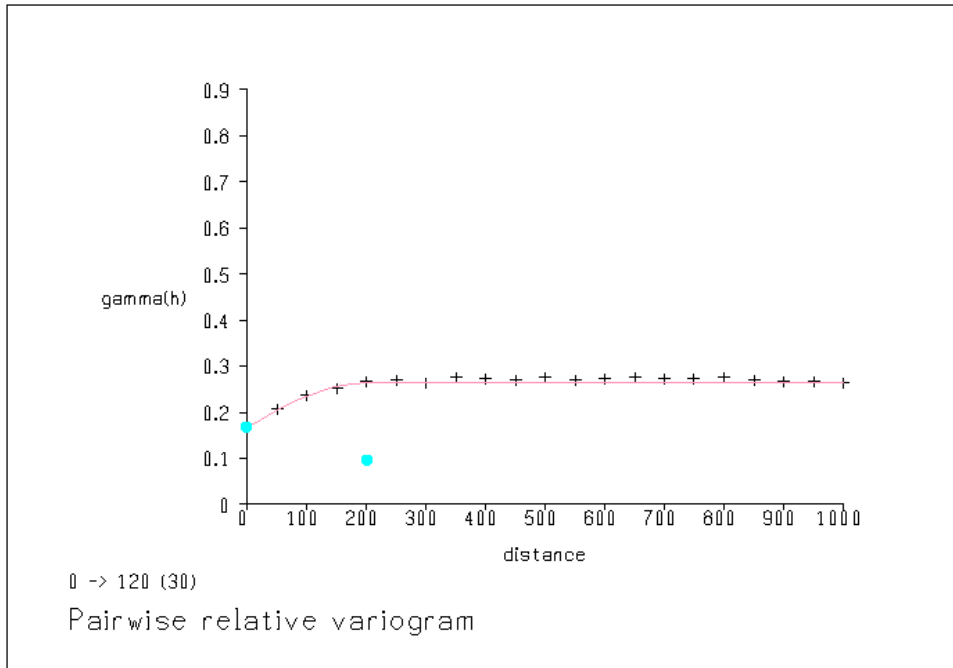
Figure 14.4 Hilton Creek / South Zone Variogram (Major Axis)
