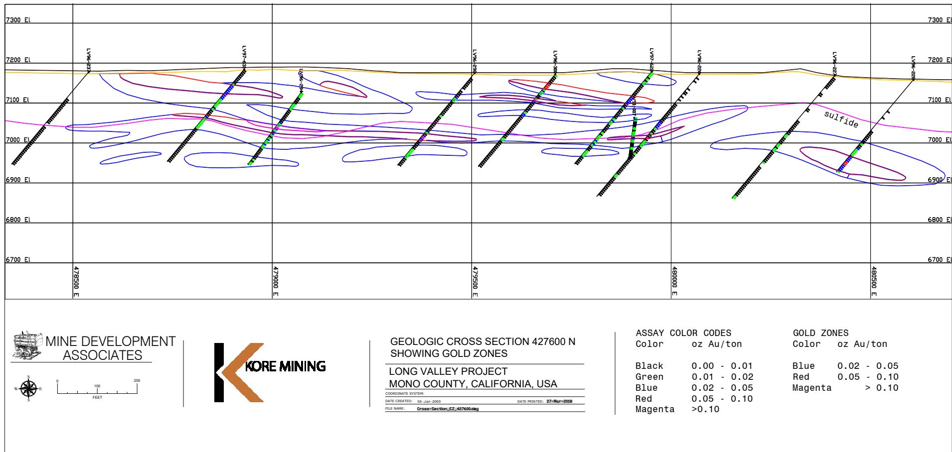
Figure 7.5 Southeast Zone Cross Section
