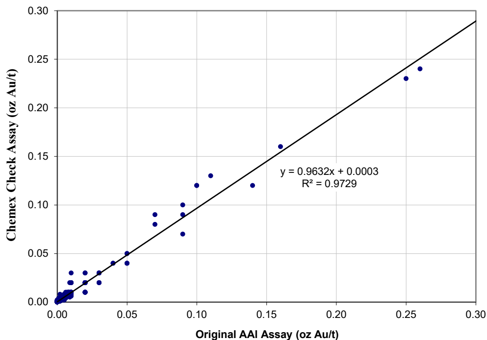
Figure 11.4 Check Assays on Coarse Rejects
