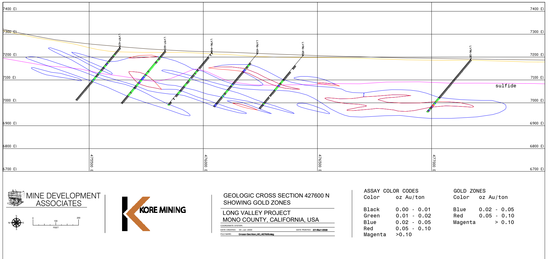
Figure 7.4 Hilton Creek Cross Section
