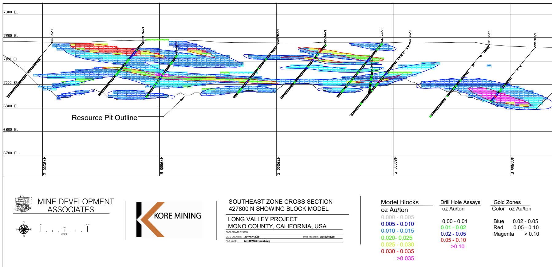
Figure 14.8 Southeast Zone Block Model Cross Section, Looking North
