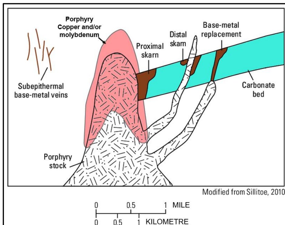
Figure 22: Simplified drawing of a skarn-porphyry system (by the USGS, after Sillitoe, 2010).
