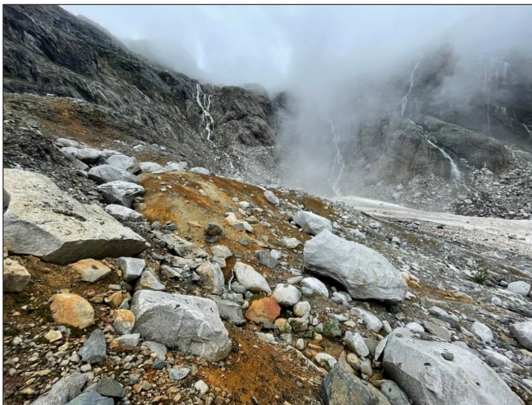
Photo 16: TOE Zone recent exposures: rusty glacial till in foreground, rusty, pyritic outcrops in back left corner. Looking south, ~400 m south of original TOE Zone outcrop
