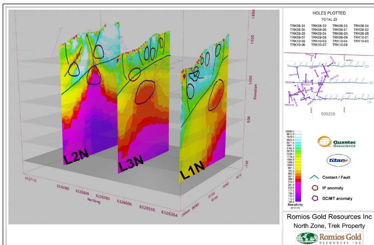
Figure 26: Geosoft 3D view of the Trek North MT model with interpretation and DDH (Prepared by Quantec Geoscience, presented in Chadwick (2011))
