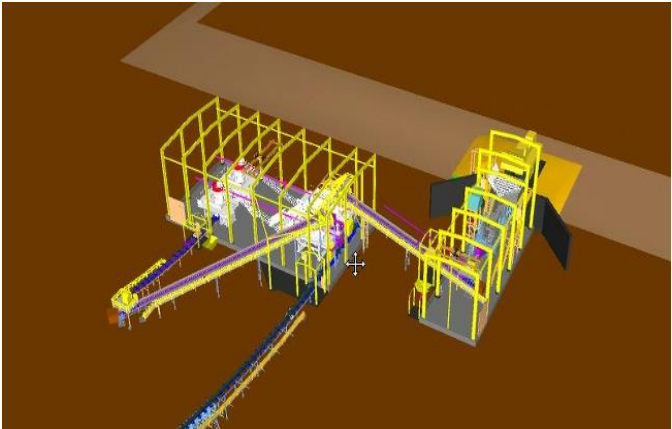
Crushing Plant
