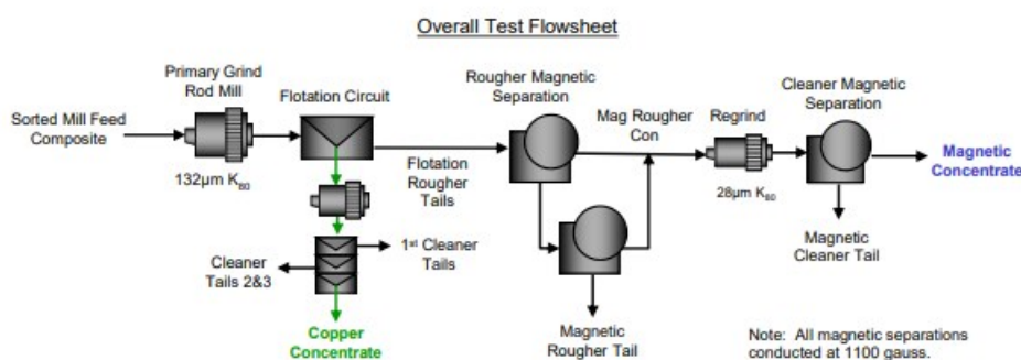
Figure 2: Overall metallurgical test flowsheet
