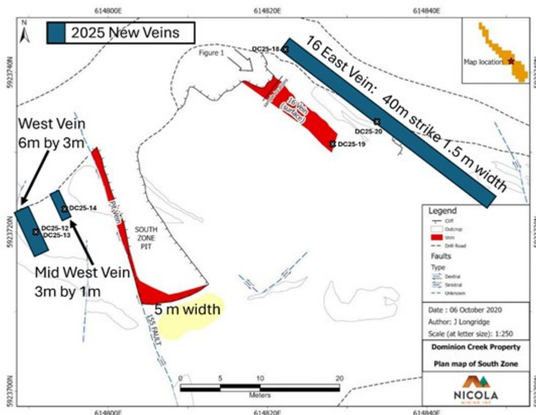
Figure 2. Current Map of Dominion Gold Project (modified from 2020 to include new veins and sample locations; note that DC-25-18 was waste pile sample)
