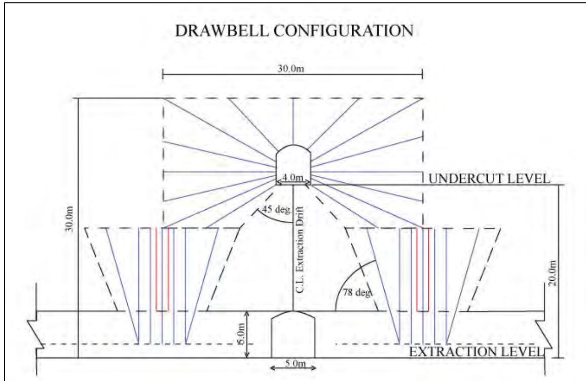
Figure 1-6 Drawbell Configuration
