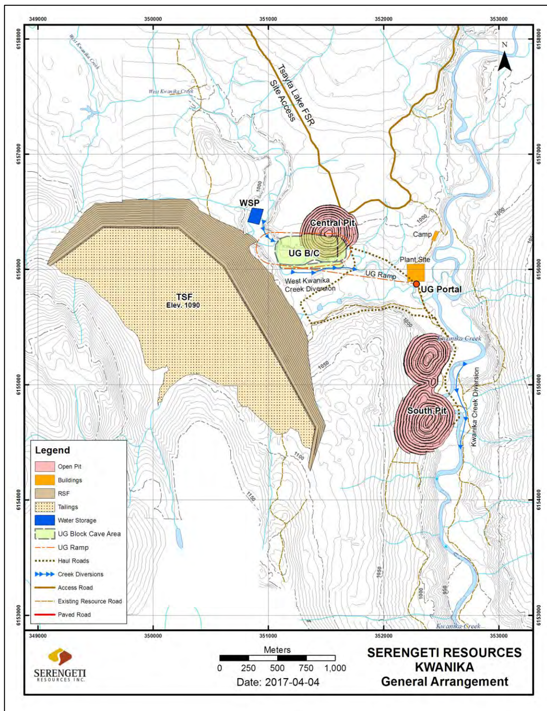
Figure 1-1 General Arrangement
