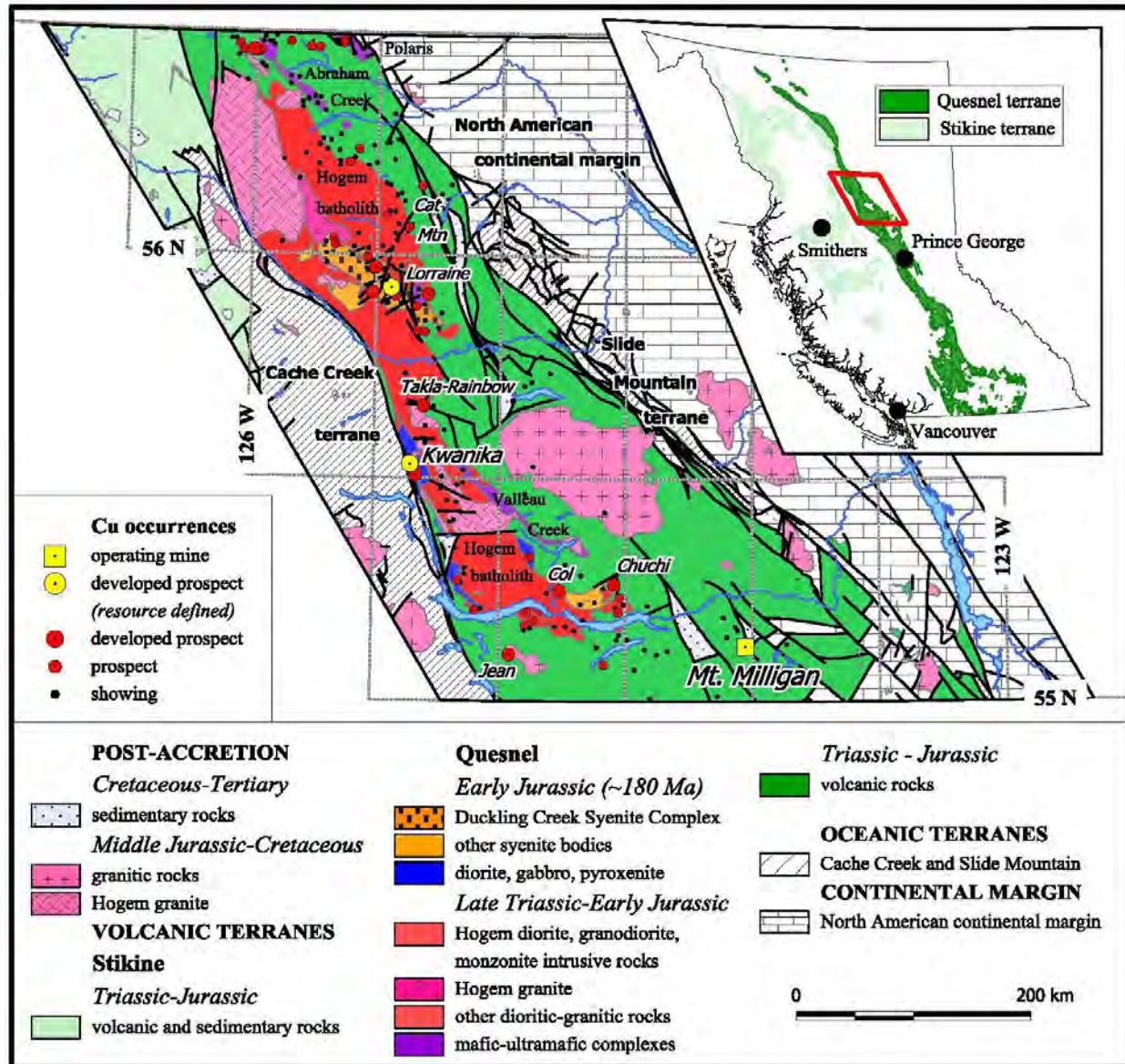
Figure 7-1 Regional Geology
