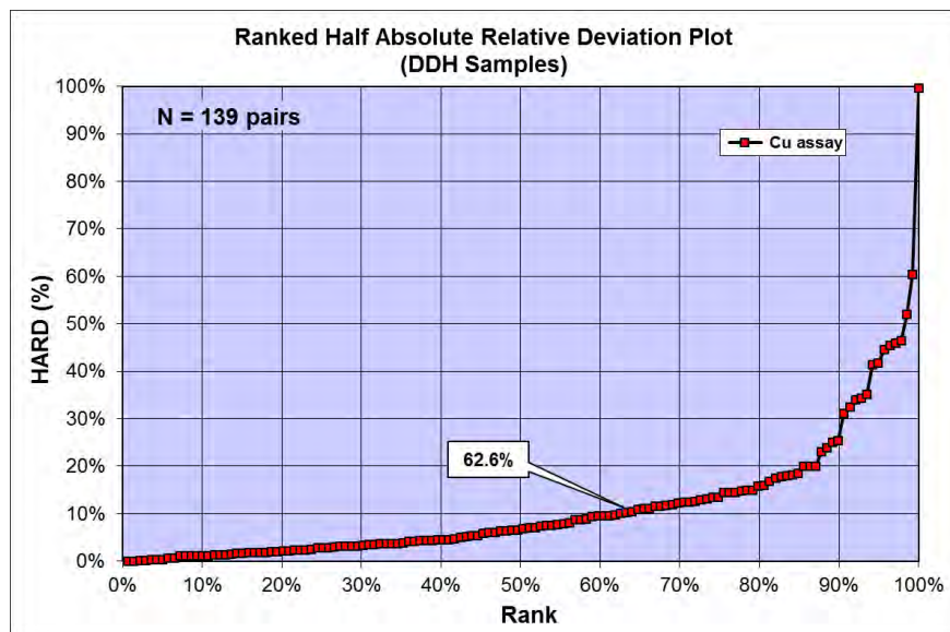
Figure 12-14 Copper Field Duplicates Plotted as Relative Deviation
