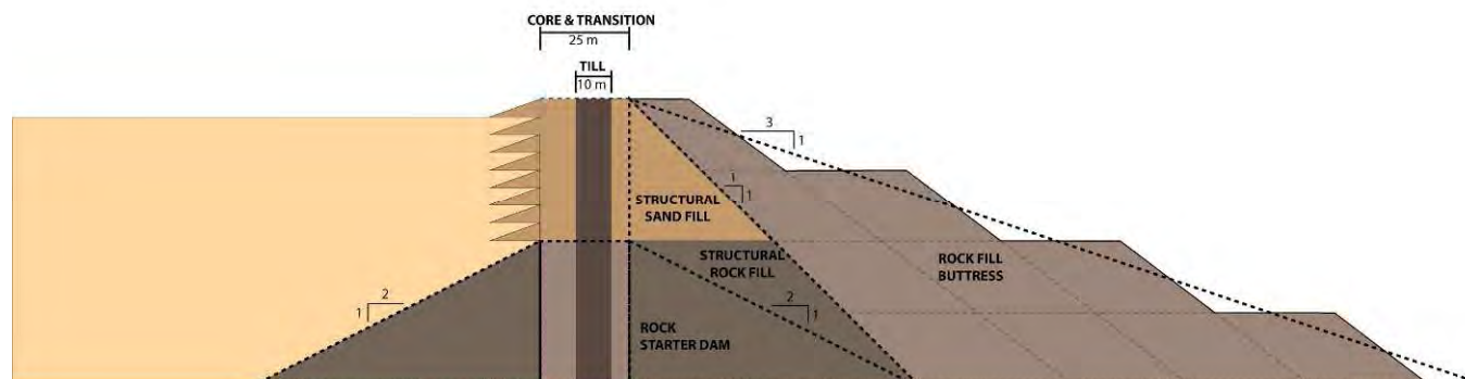
Basic template used for costing Rock fill buttress (Rock Storage Facility)
