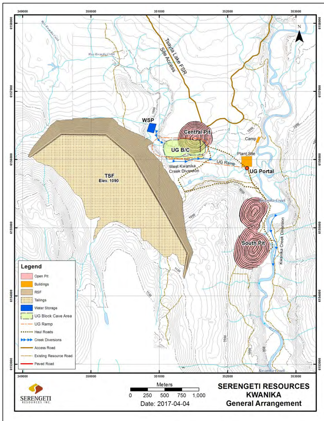
Figure 18-1 General Site Layout and Site Infrastructure
