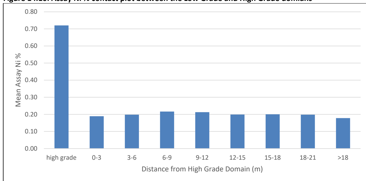
Figure 14.16: Assay Ni % contact plot between the Low Grade and High Grade domains
