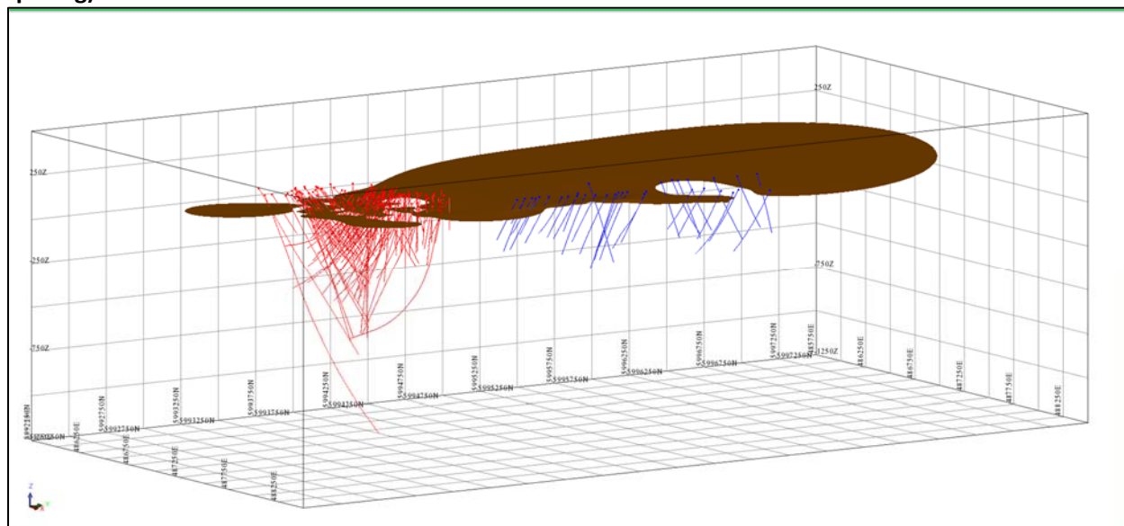
Figure 14.5: Isometric view to the Northwest of the Deposit area regolith solid model (250 m grid spacing)
