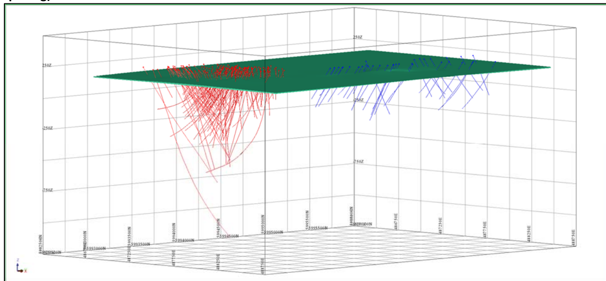
Figure 14.4: Isometric view to the Northwest of the Deposit area sandstone solid model (250 m grid spacing)
