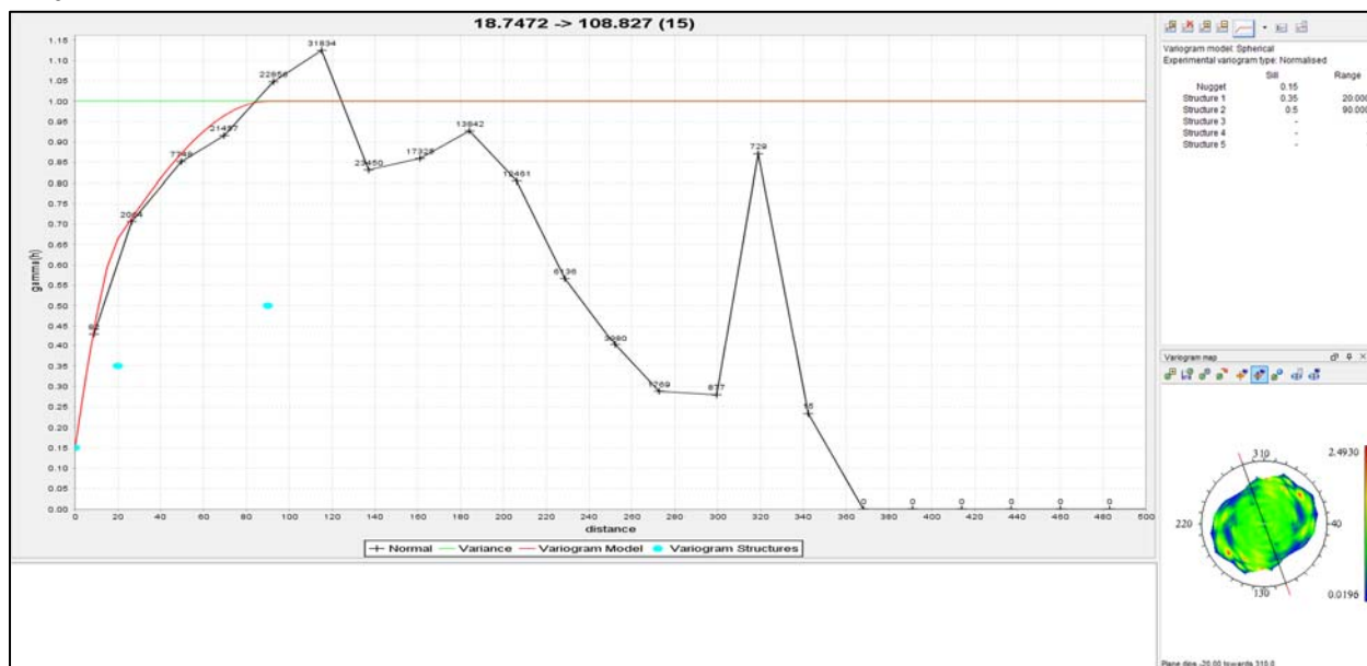
Figure 14.19: Nickel variogram model for the semi-major axis of continuity for the Nose Zone west limb
