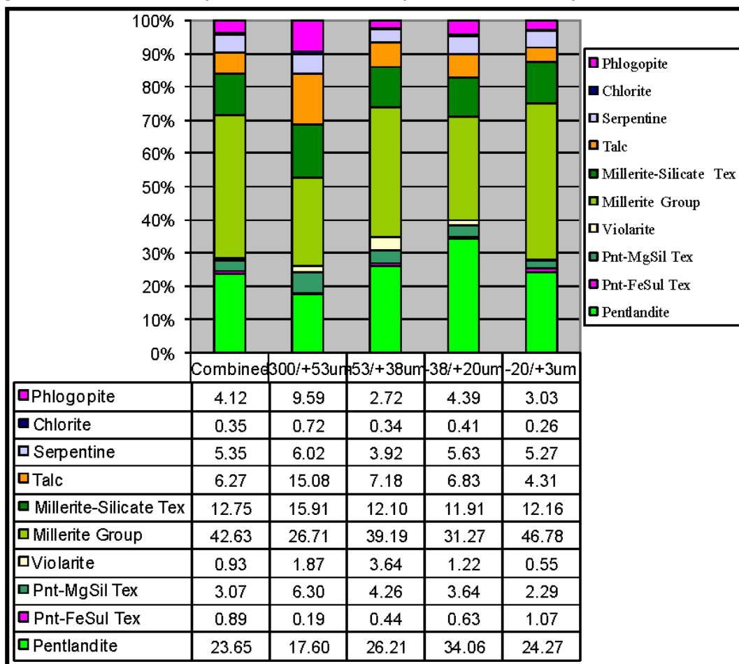
Figure 13.2: Elemental deportment of nickel in Open Pit Master Composite No. 2
