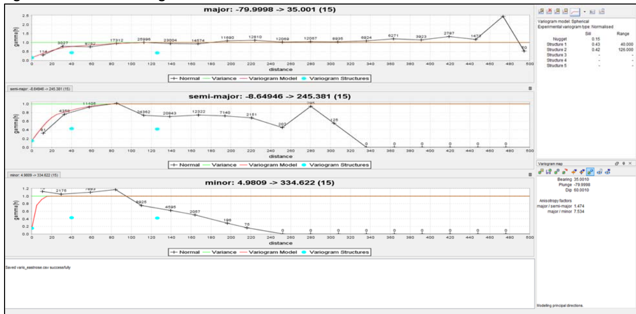
Figure 14.23: Nickel variogram model Nose Zone east limb
