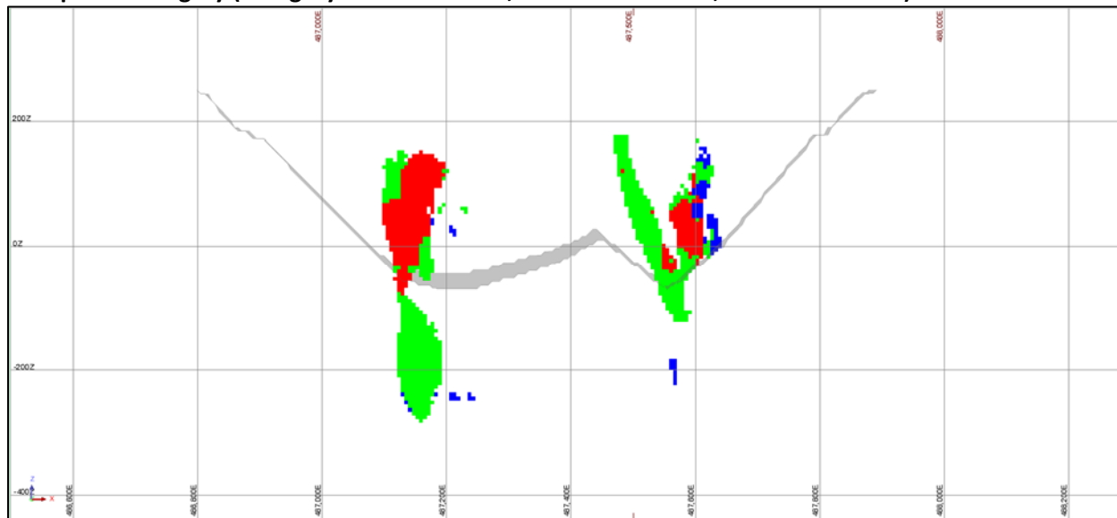
Figure 14.38: Section 5993500N (looking North) of the Minago Project mineral resource categorization with pit shell in grey (Category: Blue - Inferred, Green – Indicated, Red – Measured)
