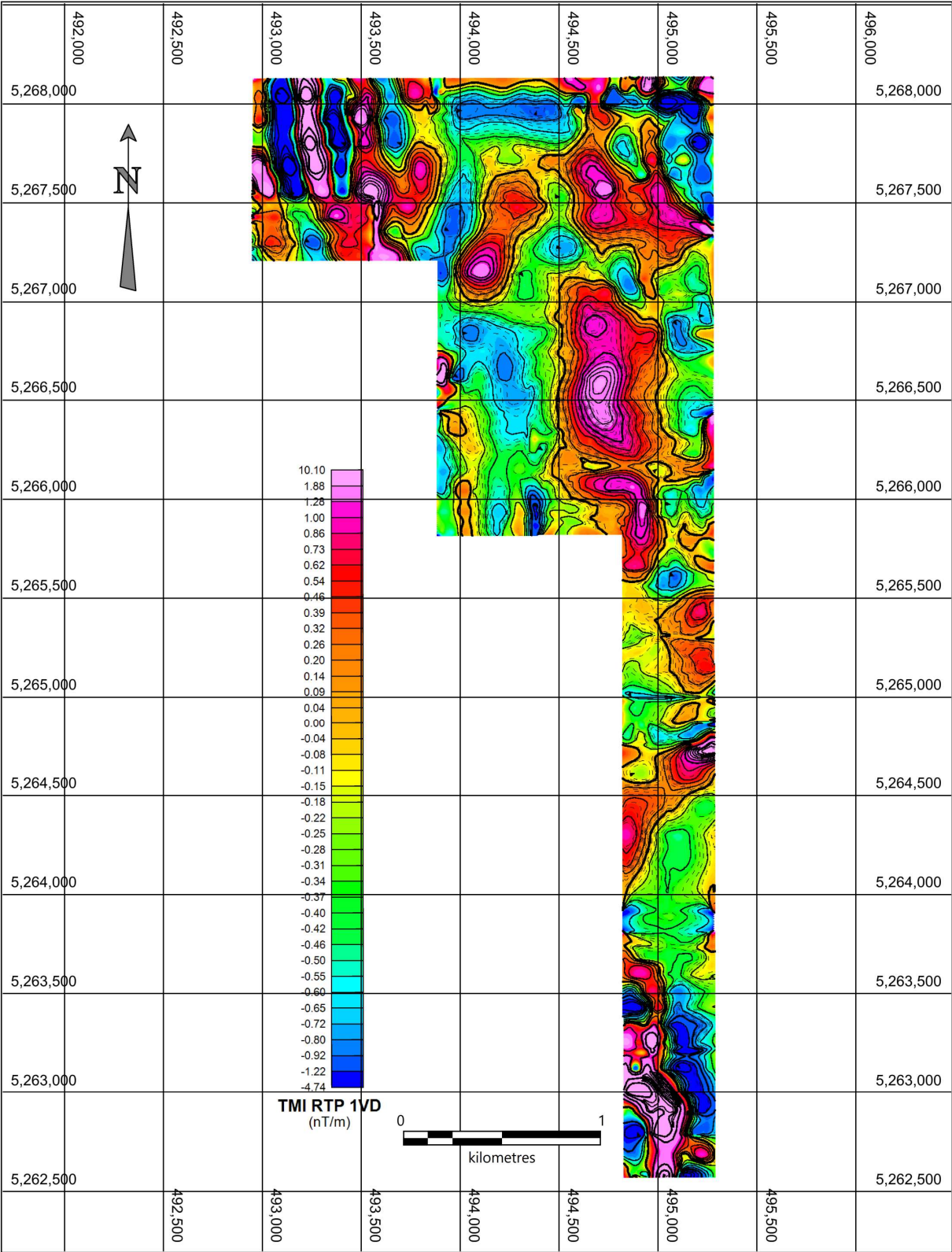
Figure 6. Initial Interpretation (1st Vertical Derivative) of Drone Magnetics
