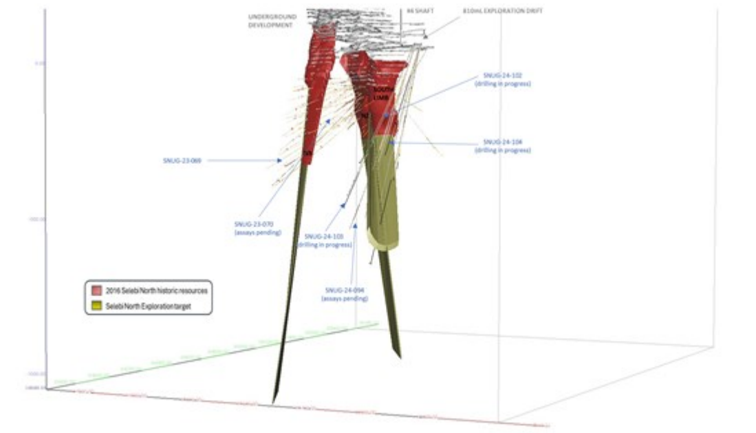
Figure 2: Selebi North: Location of Reported Drill Holes with Underground Infrastructure, Historic Resources and Exploration Targets
