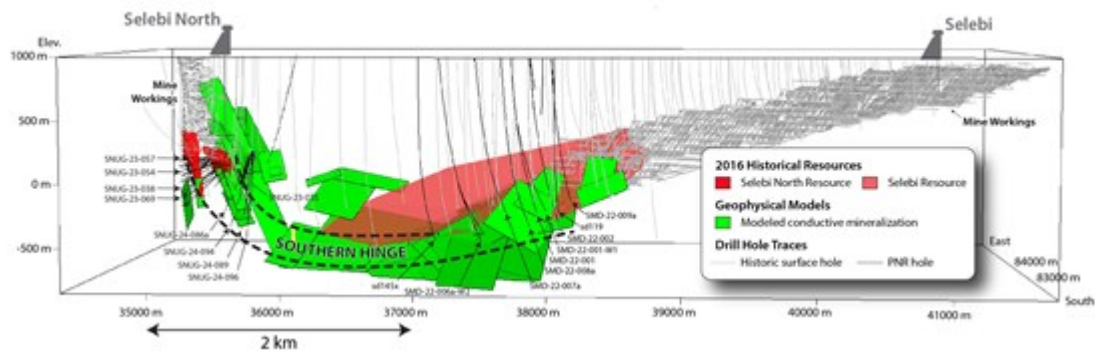
Figure 4: Long Section showing "southern hinge zone" with PNR 2022 Surface and 2023-2024 underground drillholes
