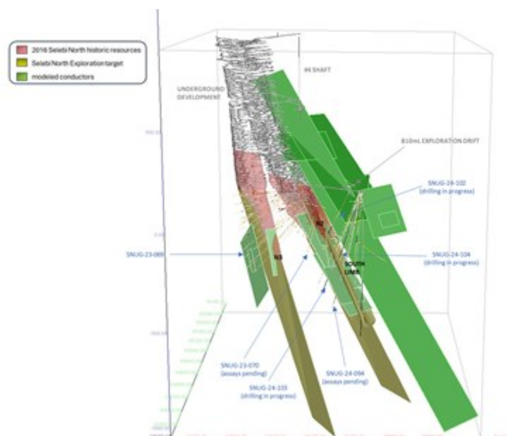
Figure 1: Selebi North: Location of Reported Drill Holes with Underground Infrastructure, Historic Resources, Exploration Targets and modeled BHEM plates.
