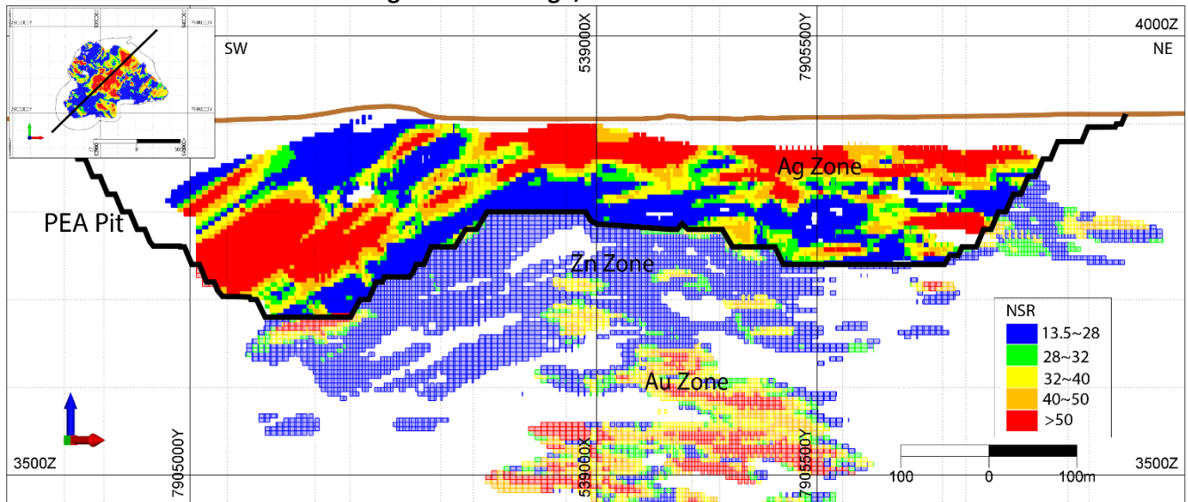
Figure 1: Pit Design, SW-NE Section View
