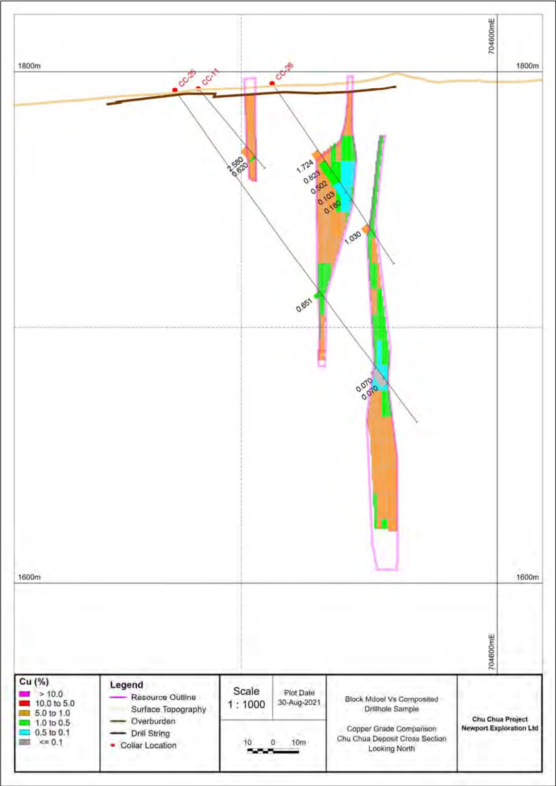
Figure 14.8. Cross-section showing Cu Block Model Grades (%) versus Cu Sample Grades
