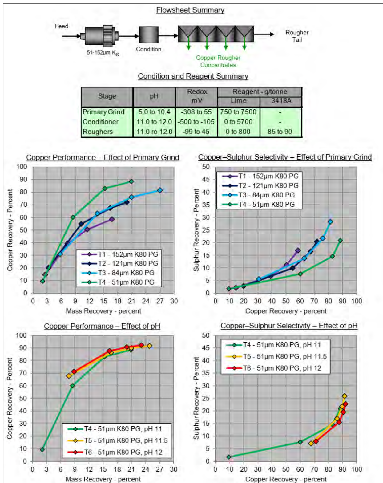
Figure 13.3. Rougher flotation response, flow-sheet summary (after Roulston and Mehrfert, 2014).
