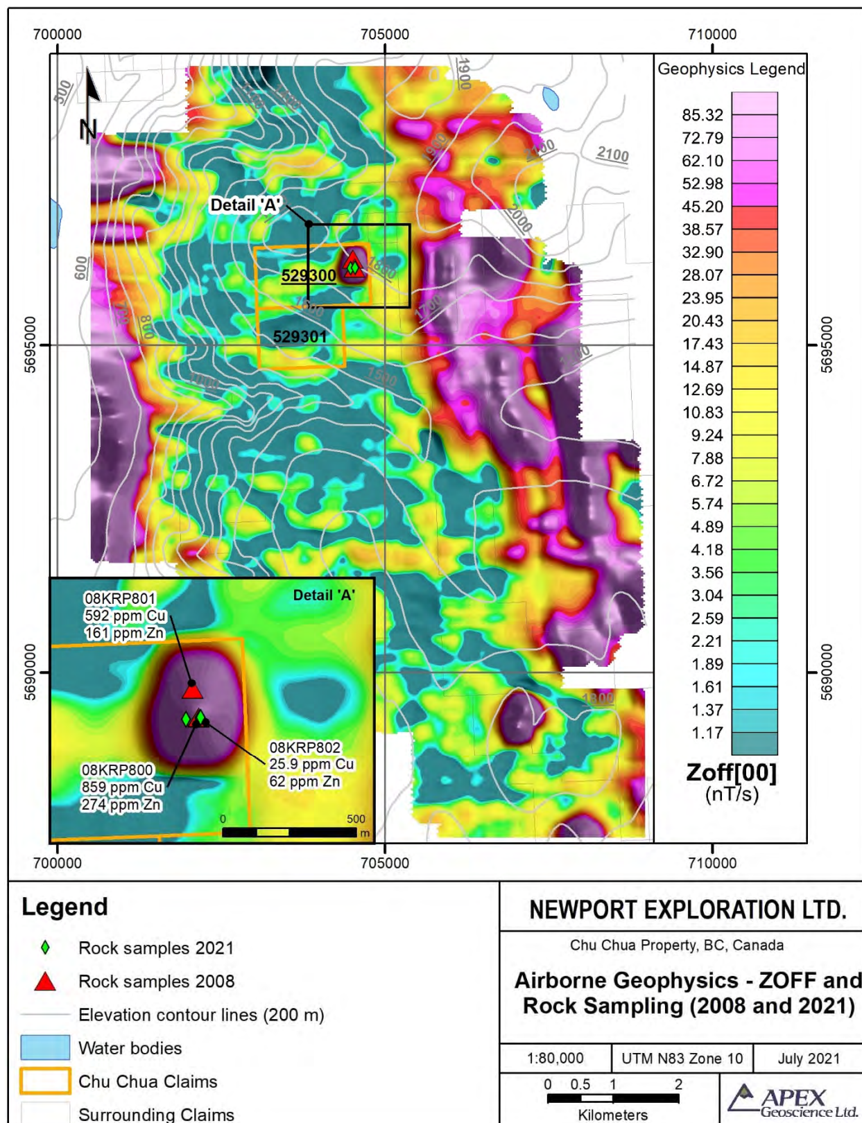
Figure 6.2. 2008 AeroTEM III Airborne Geophysical Survey (Zoff).
