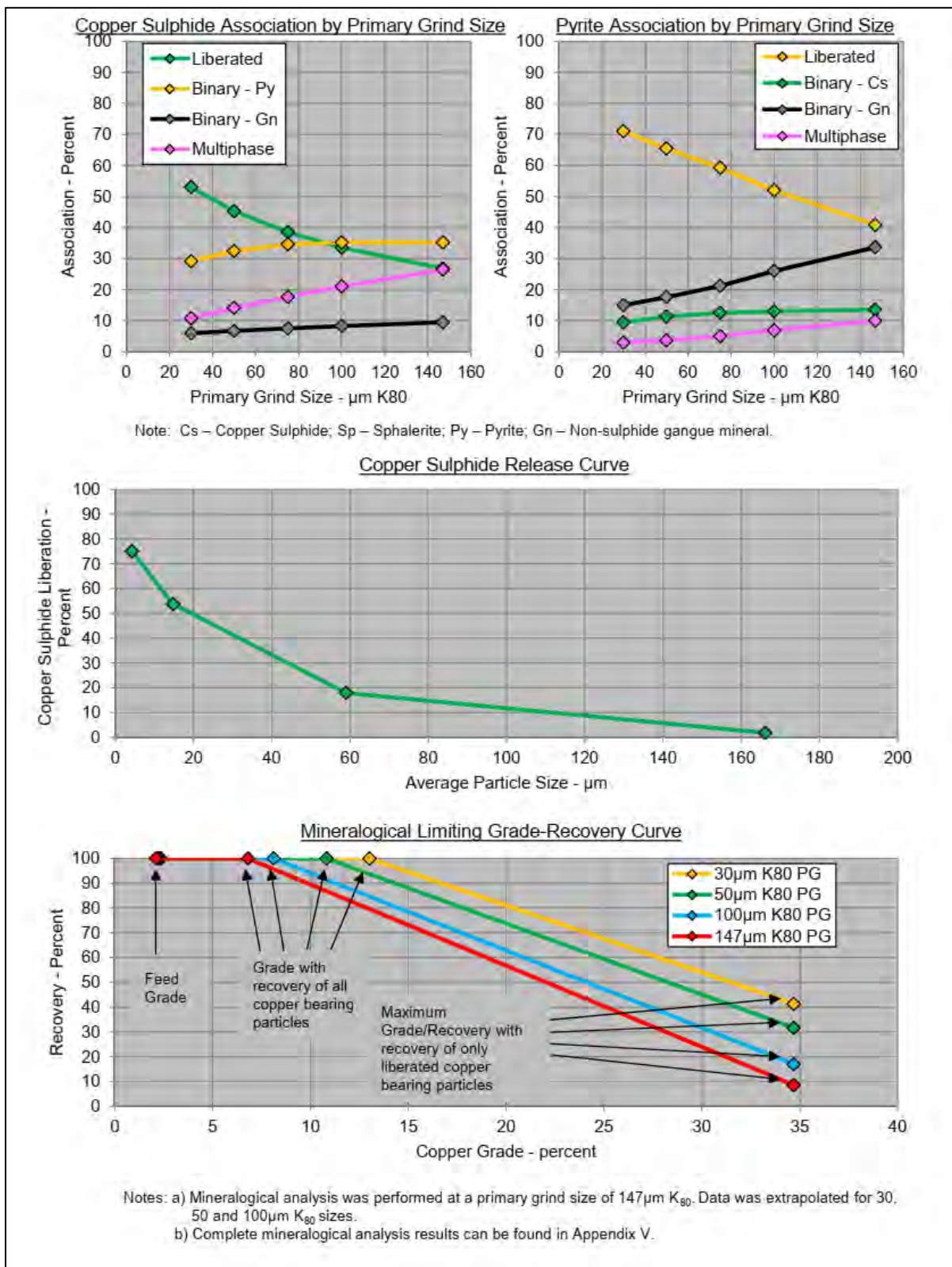
Figure 13.1. Mineral Fragmentation (after Roulston and Mehrfert, 2014).
