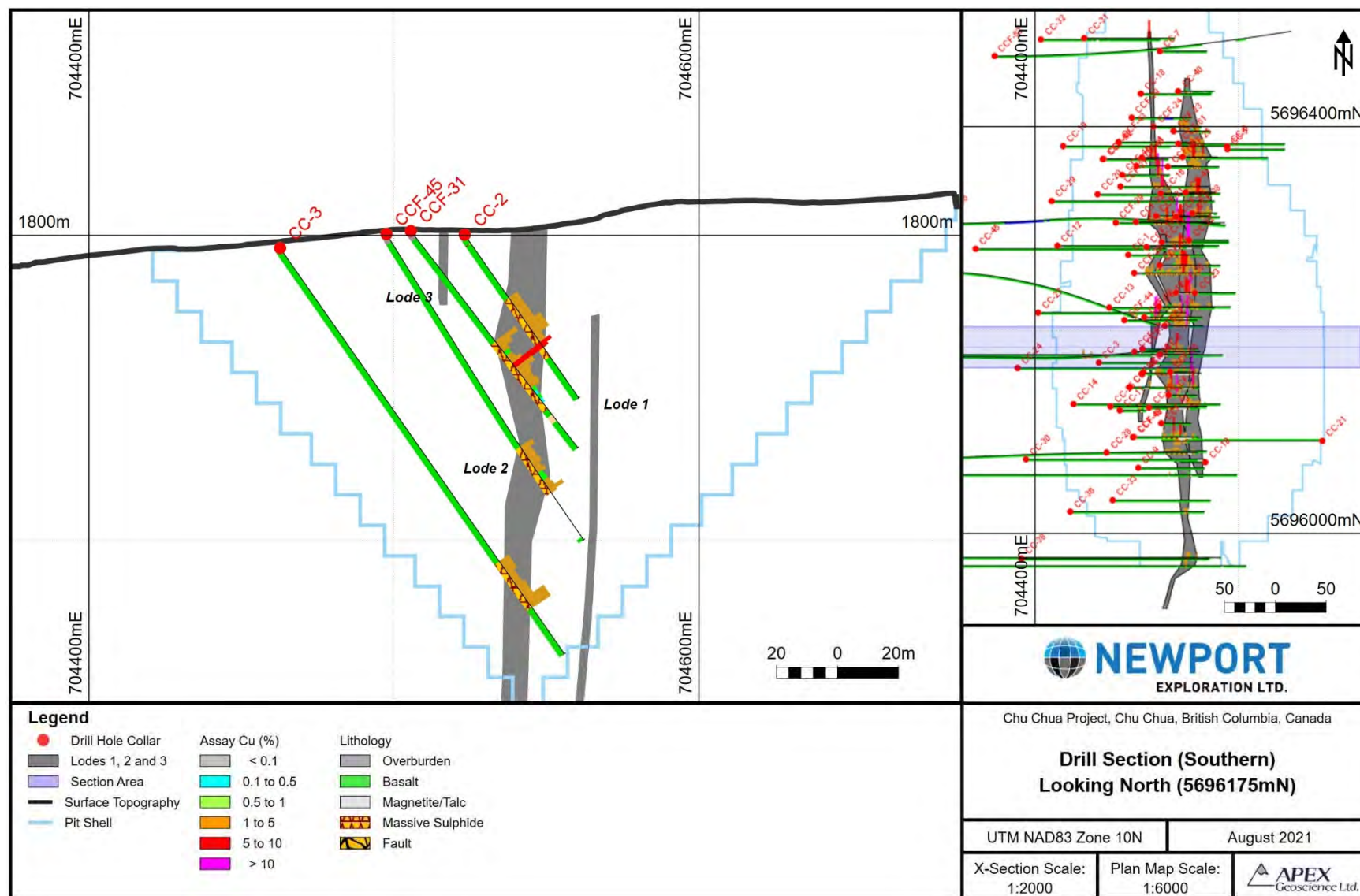
Figure 10.1. East-West Southern section 5696175mN looking North
