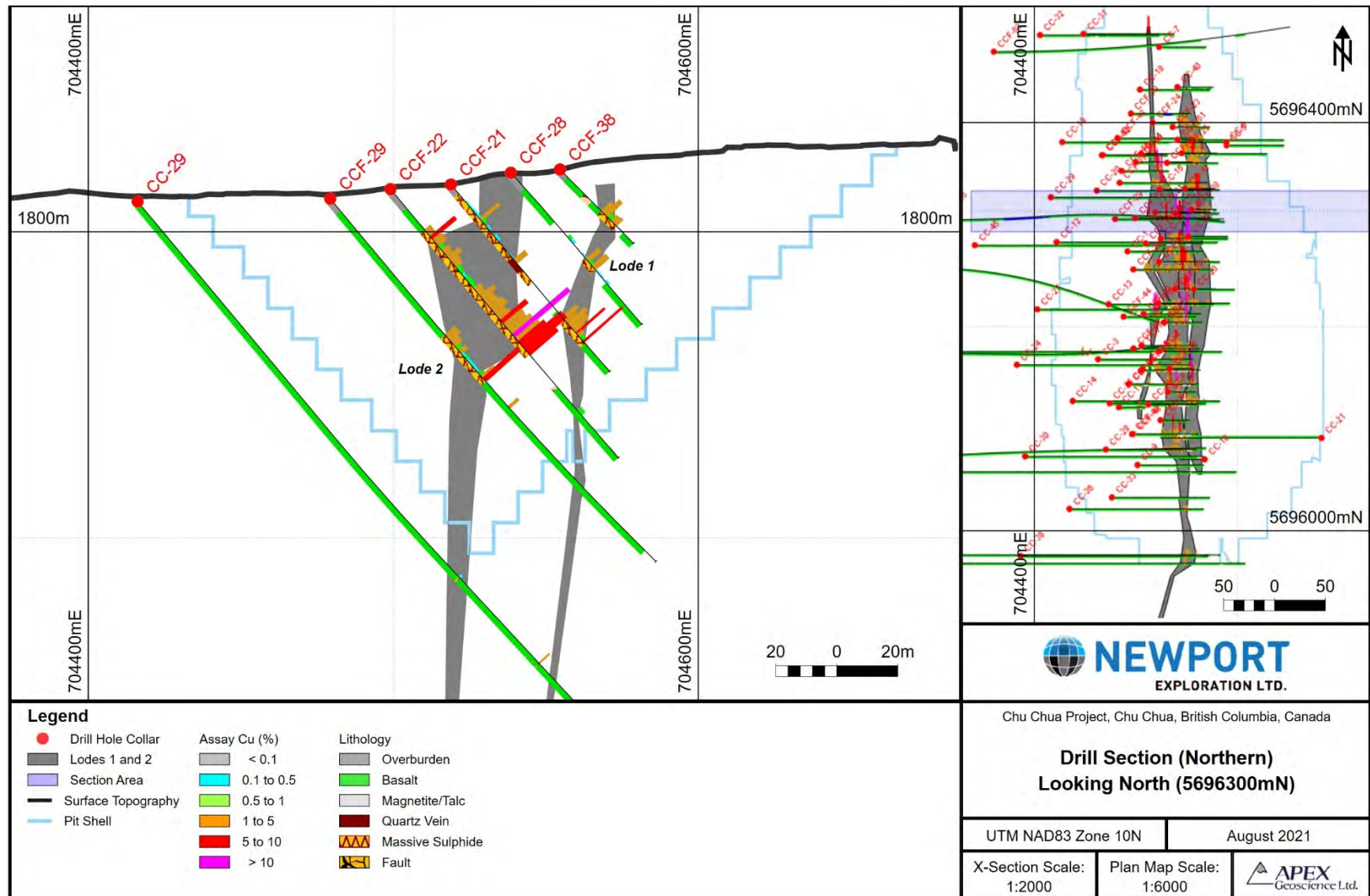
Figure 10.3. East-West Northern section 569300mN looking North
