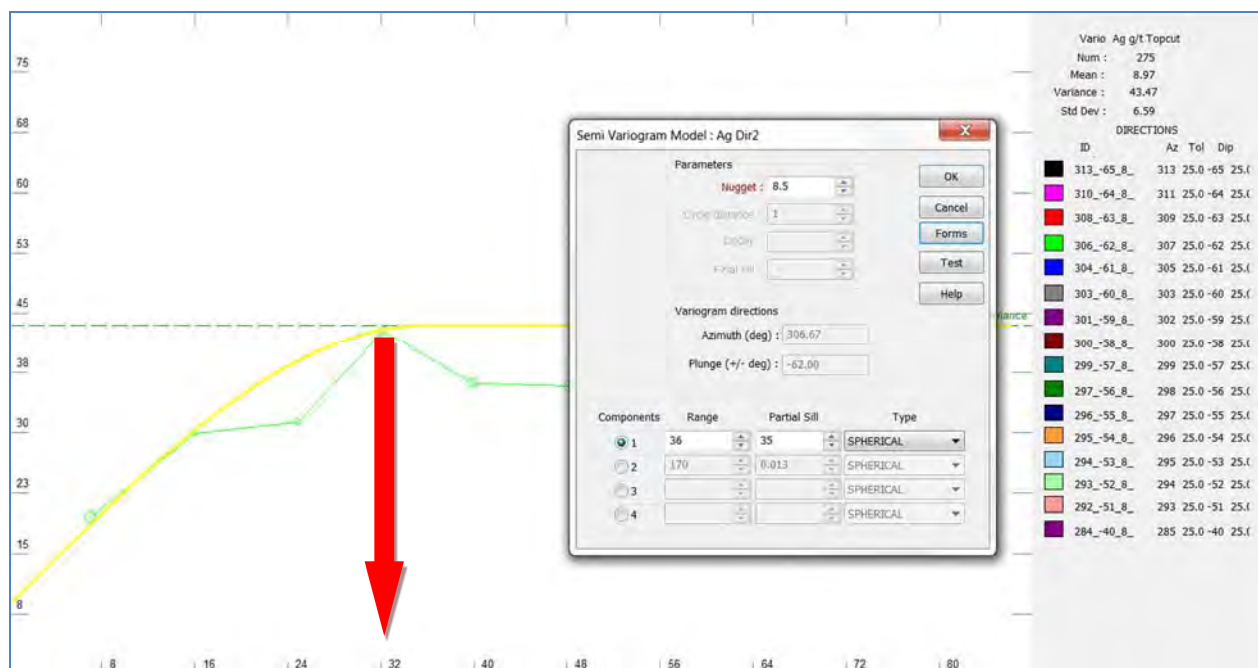
Directional Variogram. Second Direction. Suggested range 36m.
