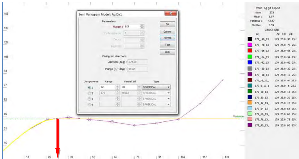
Directional variogram. Strike of 179° and 18° plunge. Suggested range of 32m.
