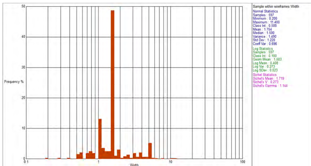
Figure 14.6. Histogram of Sample Length for the Chu Chua Domain Prior to Compositing
