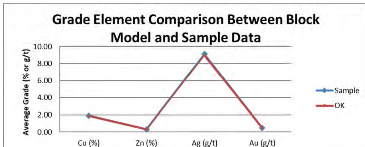
Figure 14.7. Average Grade Element Comparison Between Input Sample and OK Block Model Data
