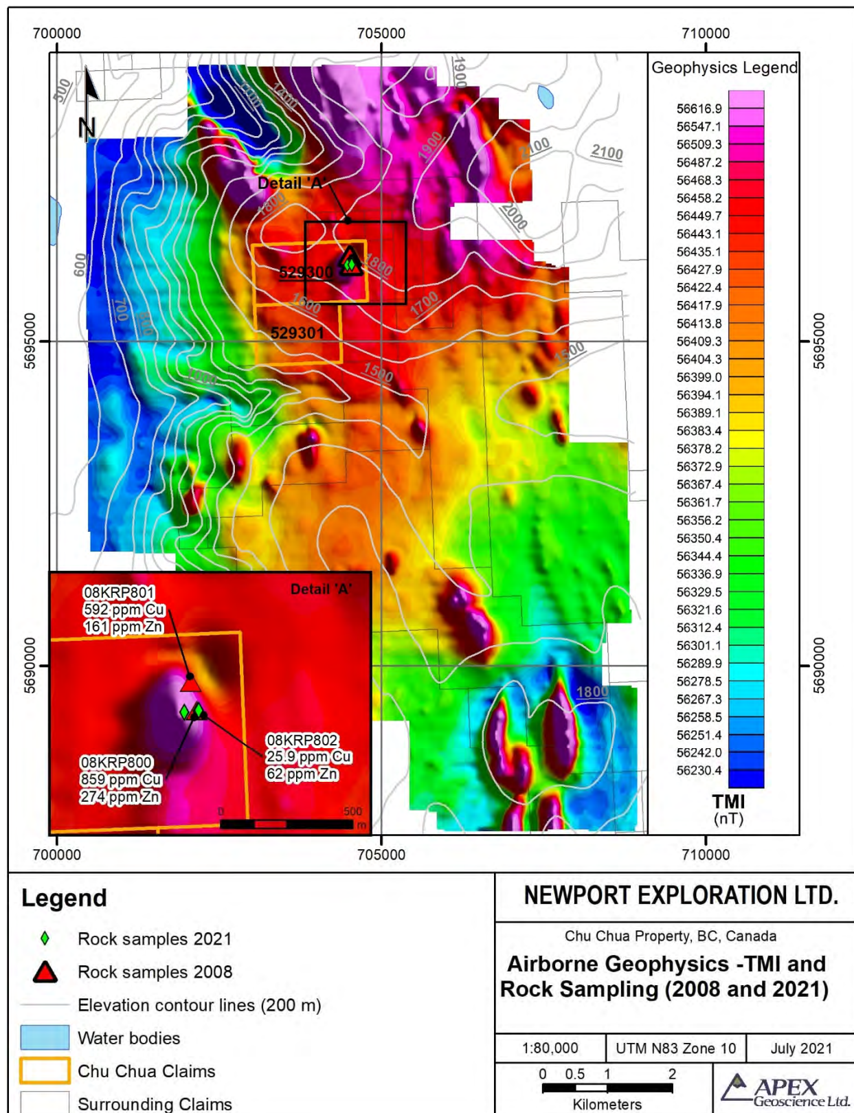
Figure 6.3. 2008 AeroTEM III Airborne Geophysical Survey (TMI)
