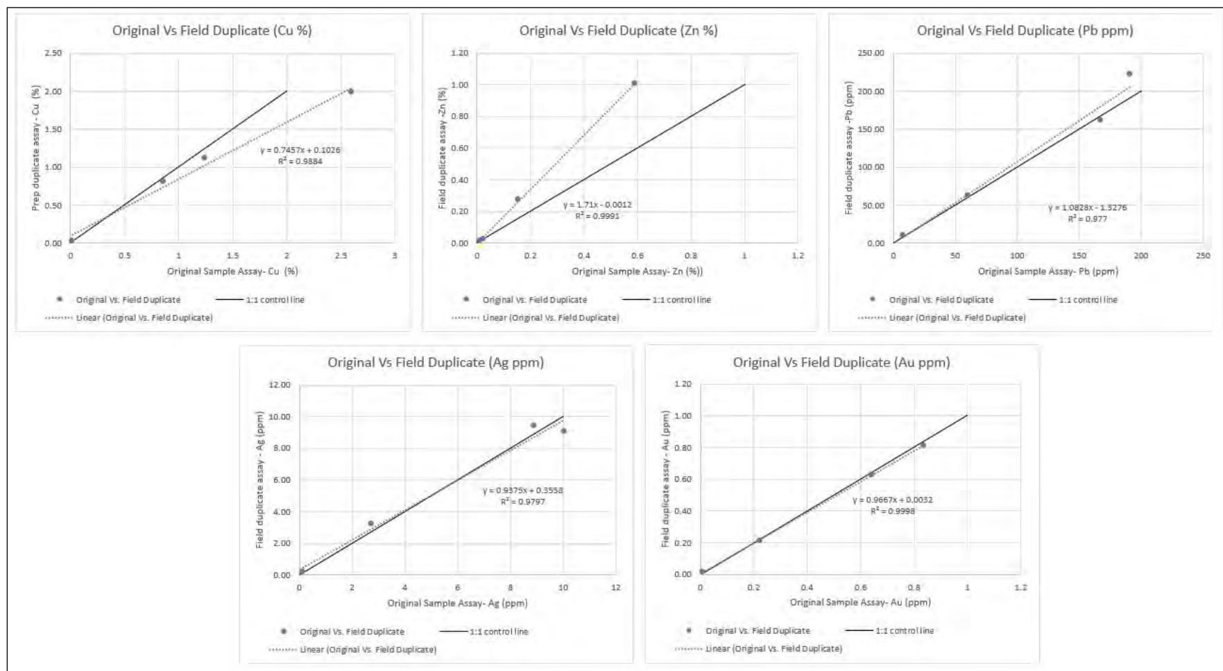
Figure 11.3. Original drill re-sample assays versus duplicate
