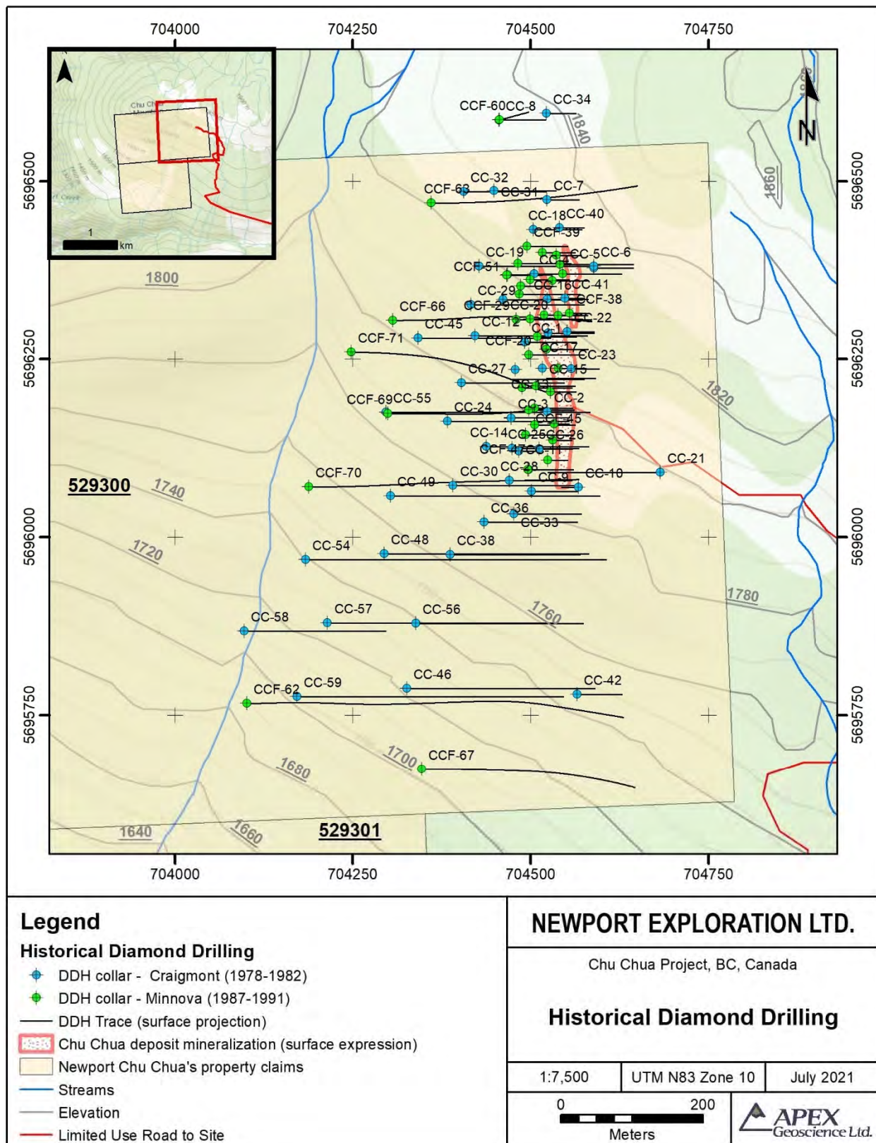
Figure 6.1. Historical Diamond Drilling of Chu Chua Deposit.
