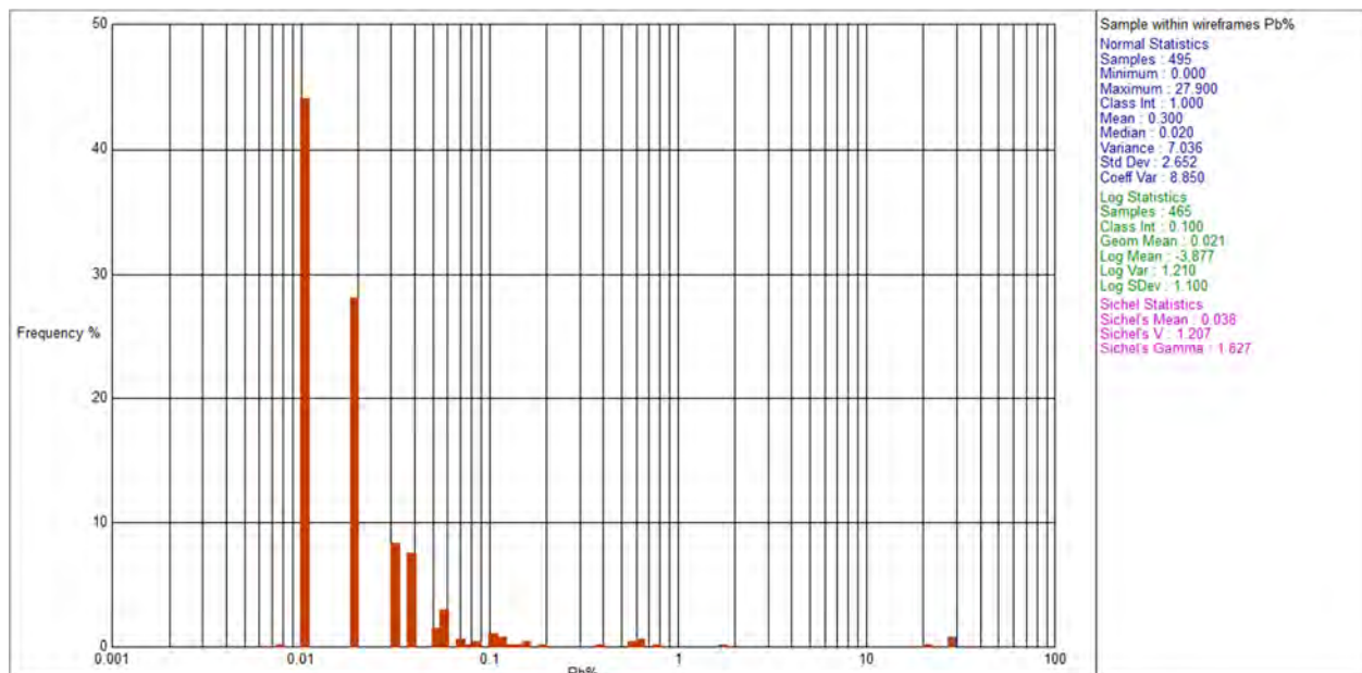
Figure 14.2. Histogram of Pb Assay Data Within Chu Chua Mineralized Zone
