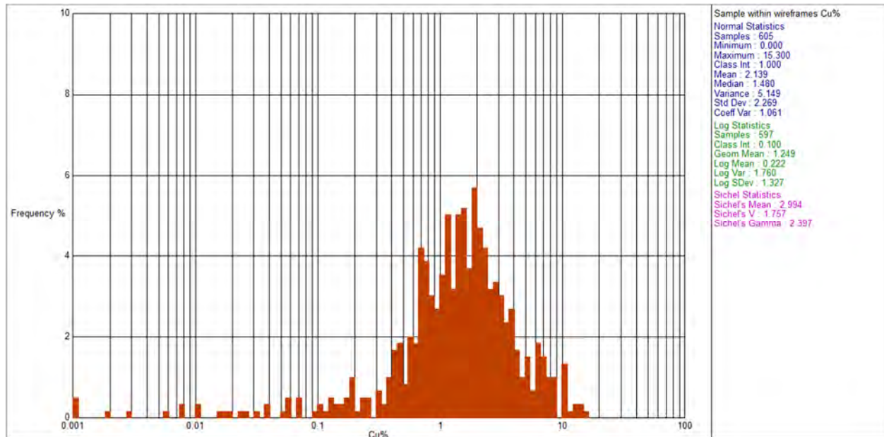
Figure 14.1. Histogram of Cu Assay Data Within Chu Chua Mineralized Zone
