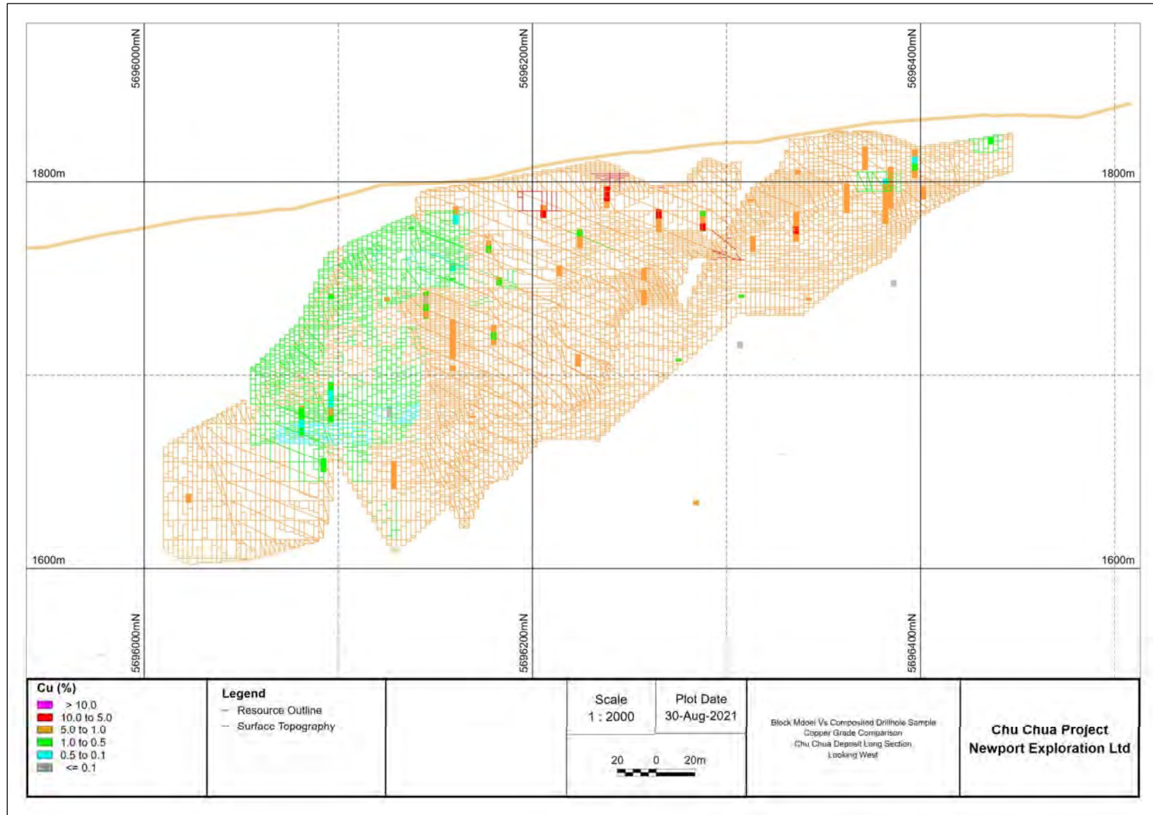
Figure 14.9. Long section showing Cu Block Model Grades (%) versus drill hole Cu Sample Grades.
