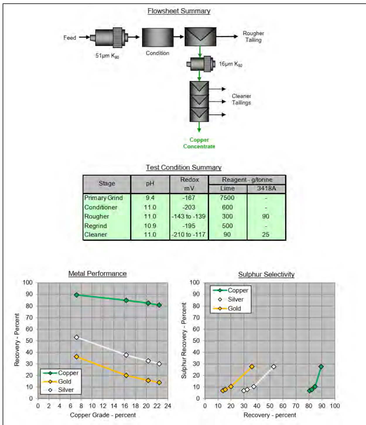
Figure 13.4. Cleaner flotation response, flow-sheet summary (after Roulston and Mehrfert, 2014).
