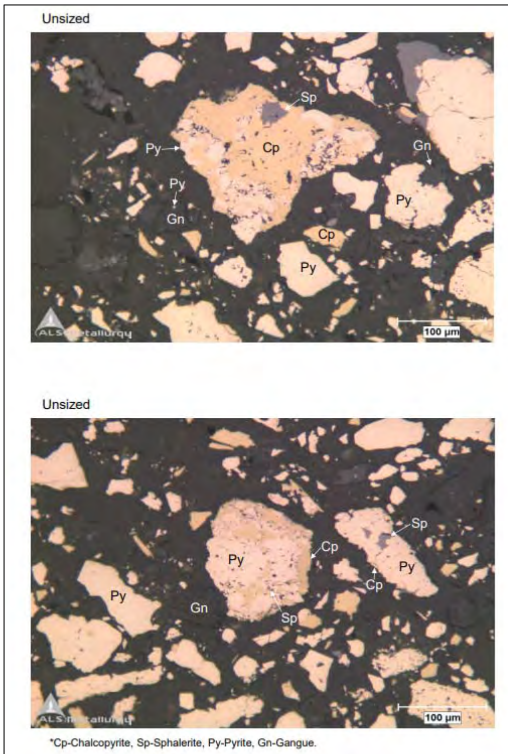
Figure 13.2. Sample photomicrograph 1 (after Roulston and Mehrfert, 2014).
