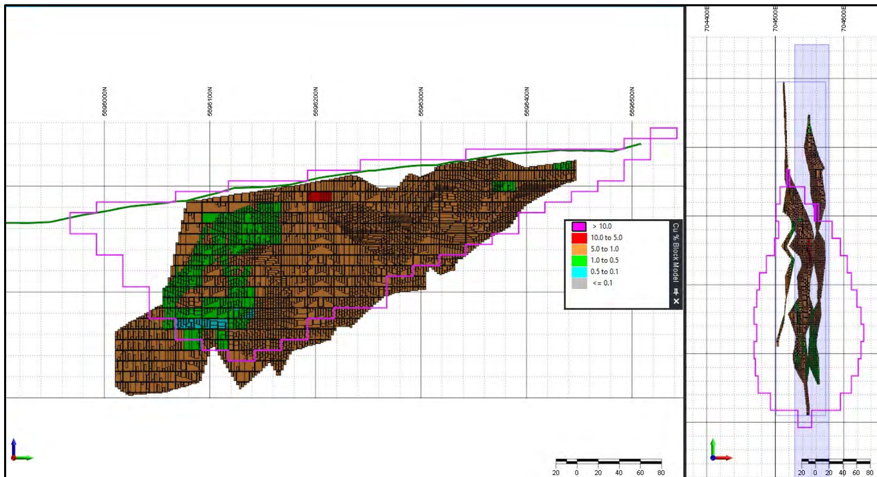
Figure 14.9 Long section of USD 4$/lb CU Lerchs-Grossman pit constraining MRE to reasonable economic extraction. LG Pit outline is shown with Magenta Line.
