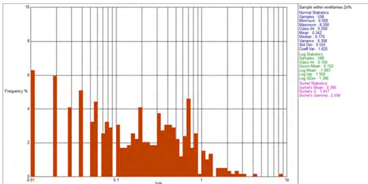
Figure 14.3. Histogram of Zn Assay Data Within Chu Chua Mineralized Zone
