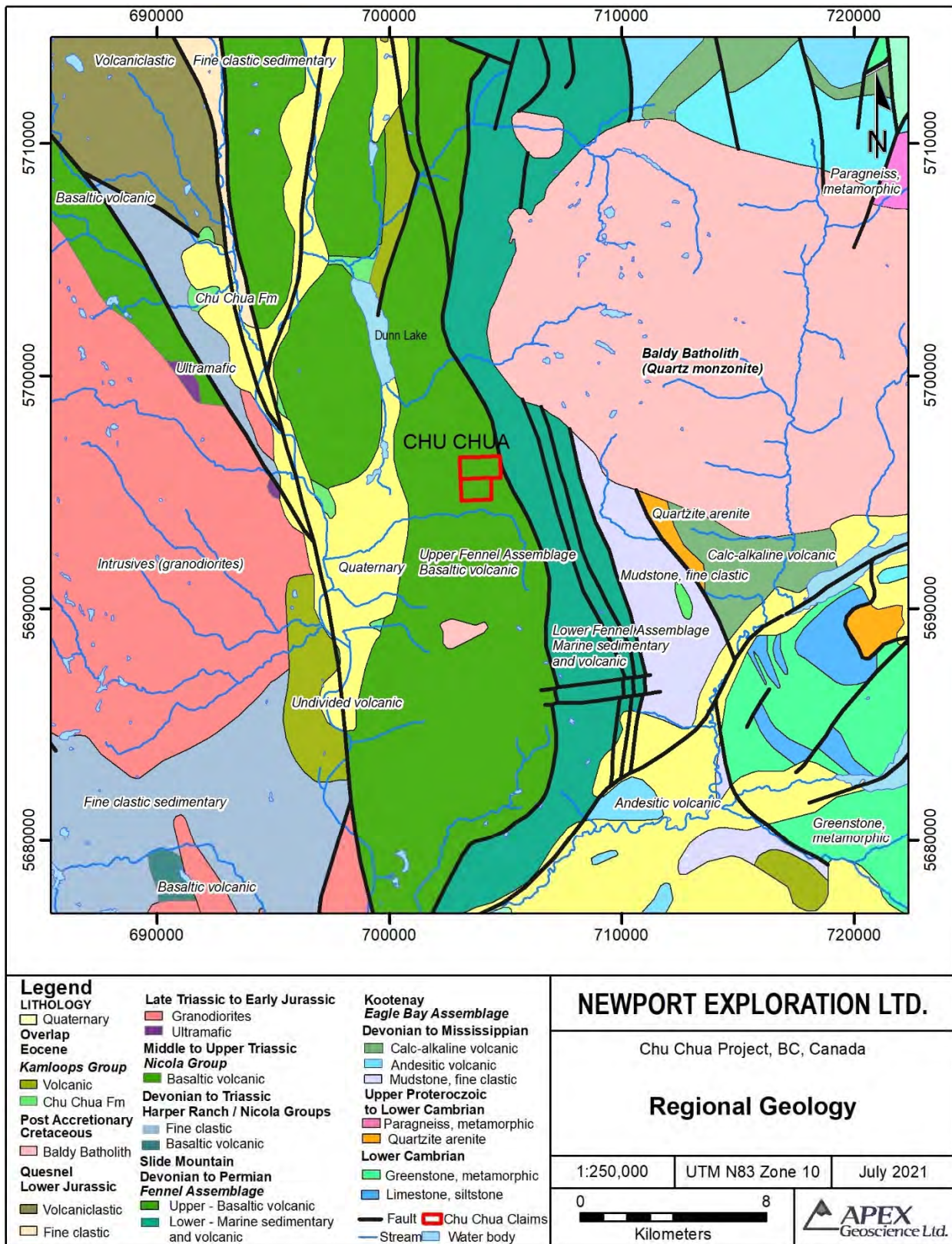
Figure 7.1. Regional Geology
