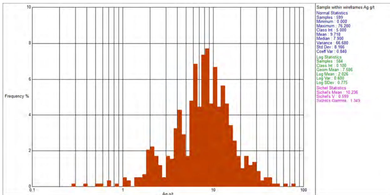
Figure 14.4. Histogram of Ag Assay Data Within Chu Chua Mineralized Zone
