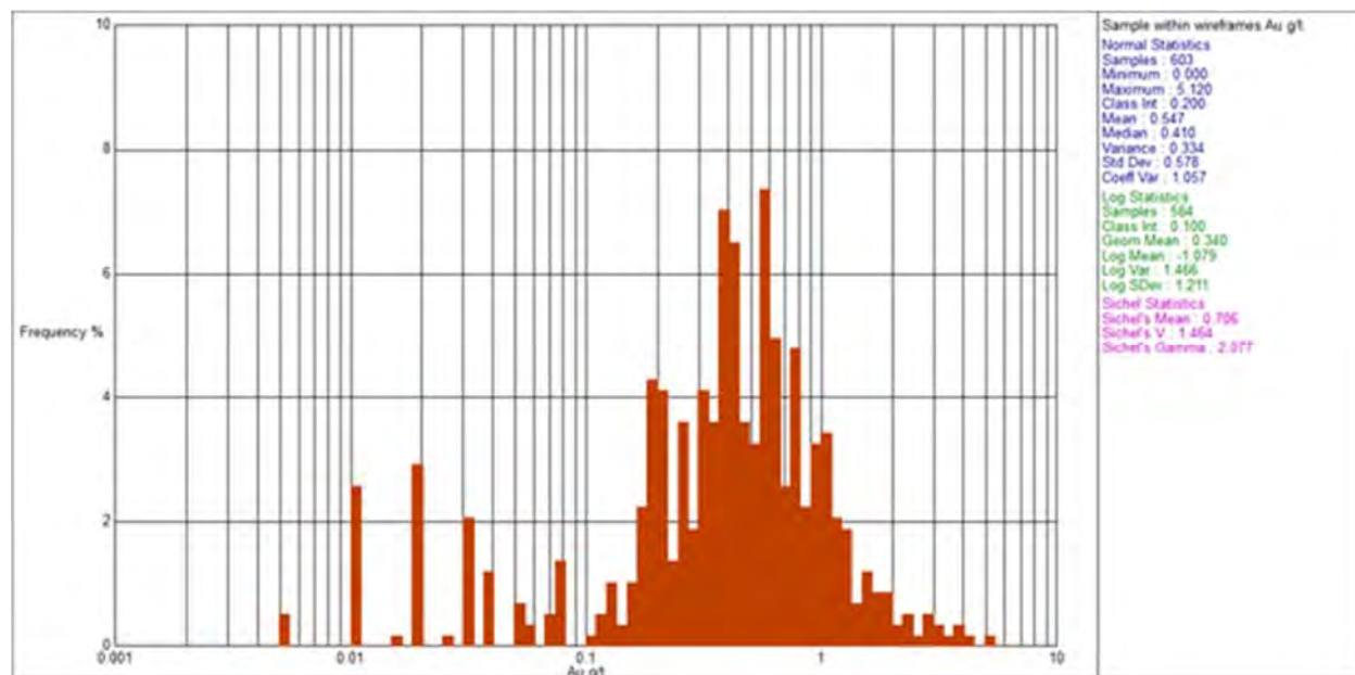
Figure 14.5. Histogram of Au Assay Data Within Chu Chua Mineralized Zone
