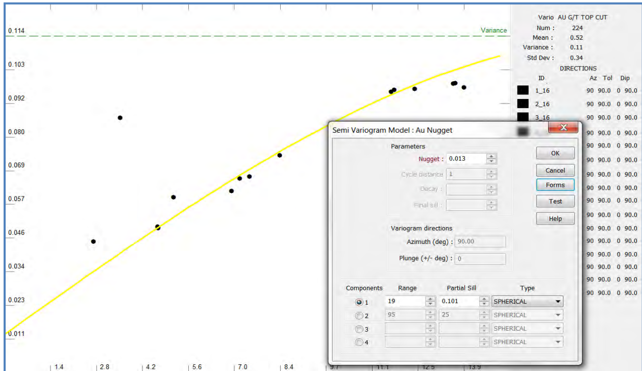
Down hole variogram. Nugget of 12.5%
