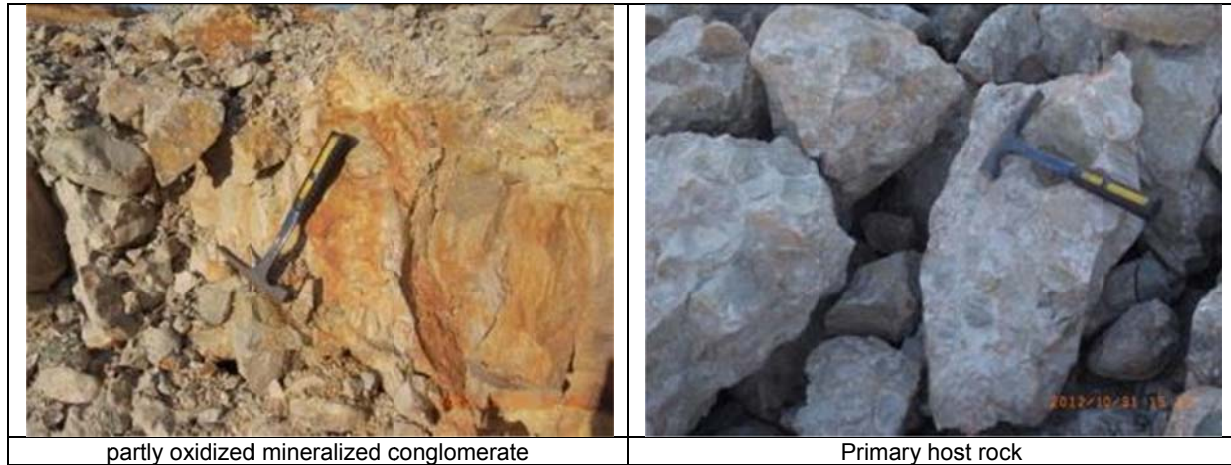
Figure 6-5: Typical Gold Mineralization Host Rocks at Songjiagou Property
