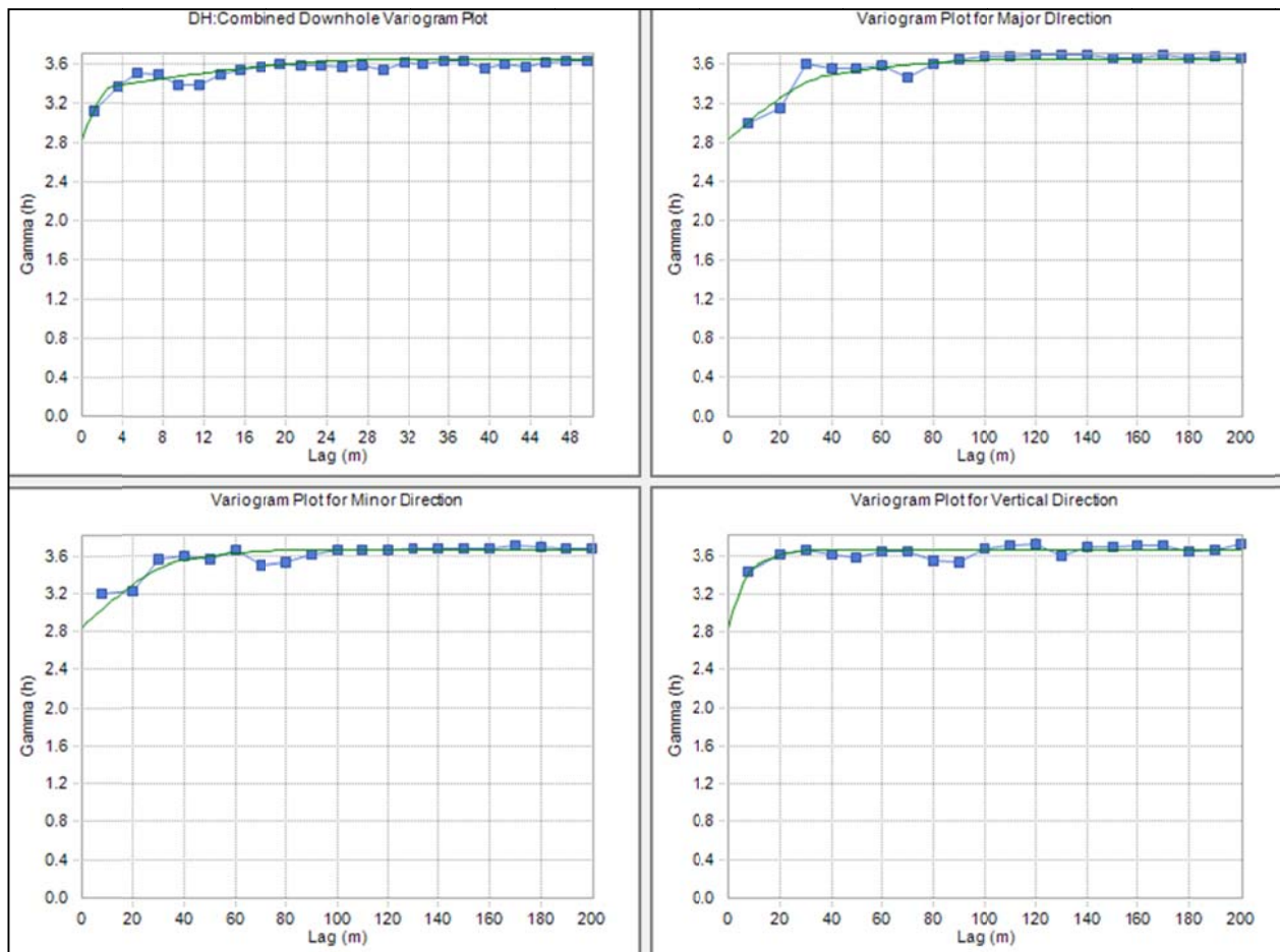
Variogram
