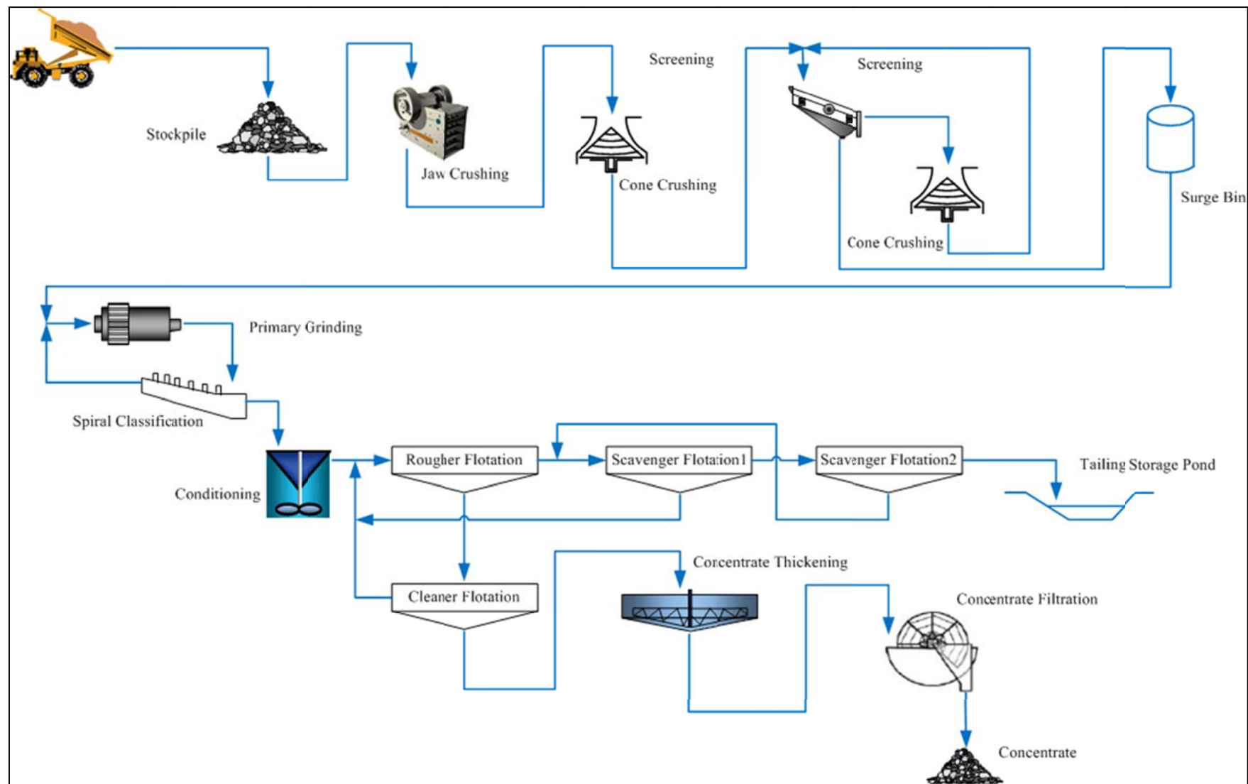
Figure 16-2: Flowsheet Adopted in 6,000 tpd Plant
