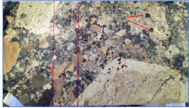
(a) (left): Polymictic Breccia illustrating higher amount of matrix (about 20% volume of breccia) with a strong black rock flour component. Note felsic clast in upper right quadrant with irregular borders indicative of juvenile material. From AP-12-162 at 135 m depth. (b) (right): Polymictic Breccia illustrating lesser amount of matrix (about 10% volume of breccia) with more igneous component. From AP-23-291 at 134 m depth.
