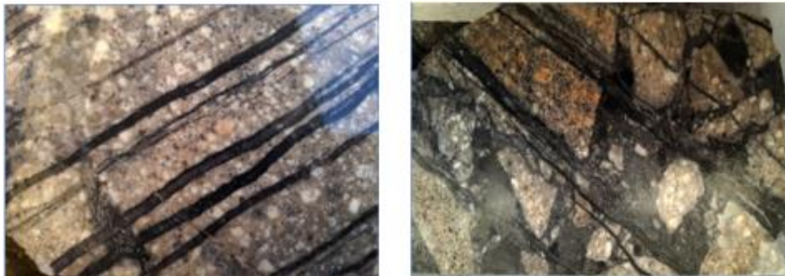
(a) (left): Sheeted 1 to 3 mm wide V2 micro-veinlets cutting the feldspar porphyry in AP-23-297 at 228 m depth. (b) (right): Sheeted 1 to 3 mm wide V2 micro-veinlets cutting the Polymictic Breccia in AP-23-297 at 222 m depth.
