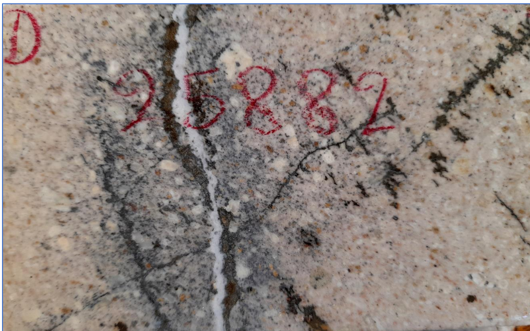
Figure 7-40: Sulphide-rich Bedding Planes (Photo 33)
