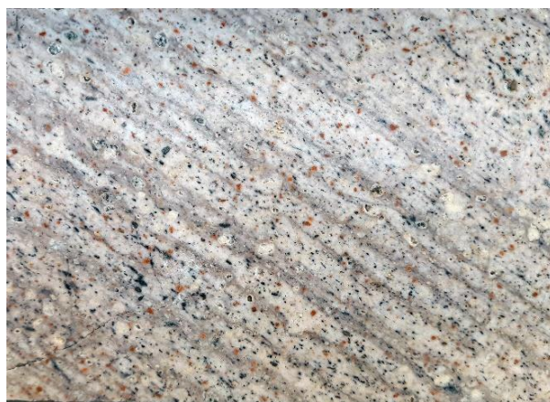
Flow banded rhyolite from AP-23-298 at 44 m depth.
