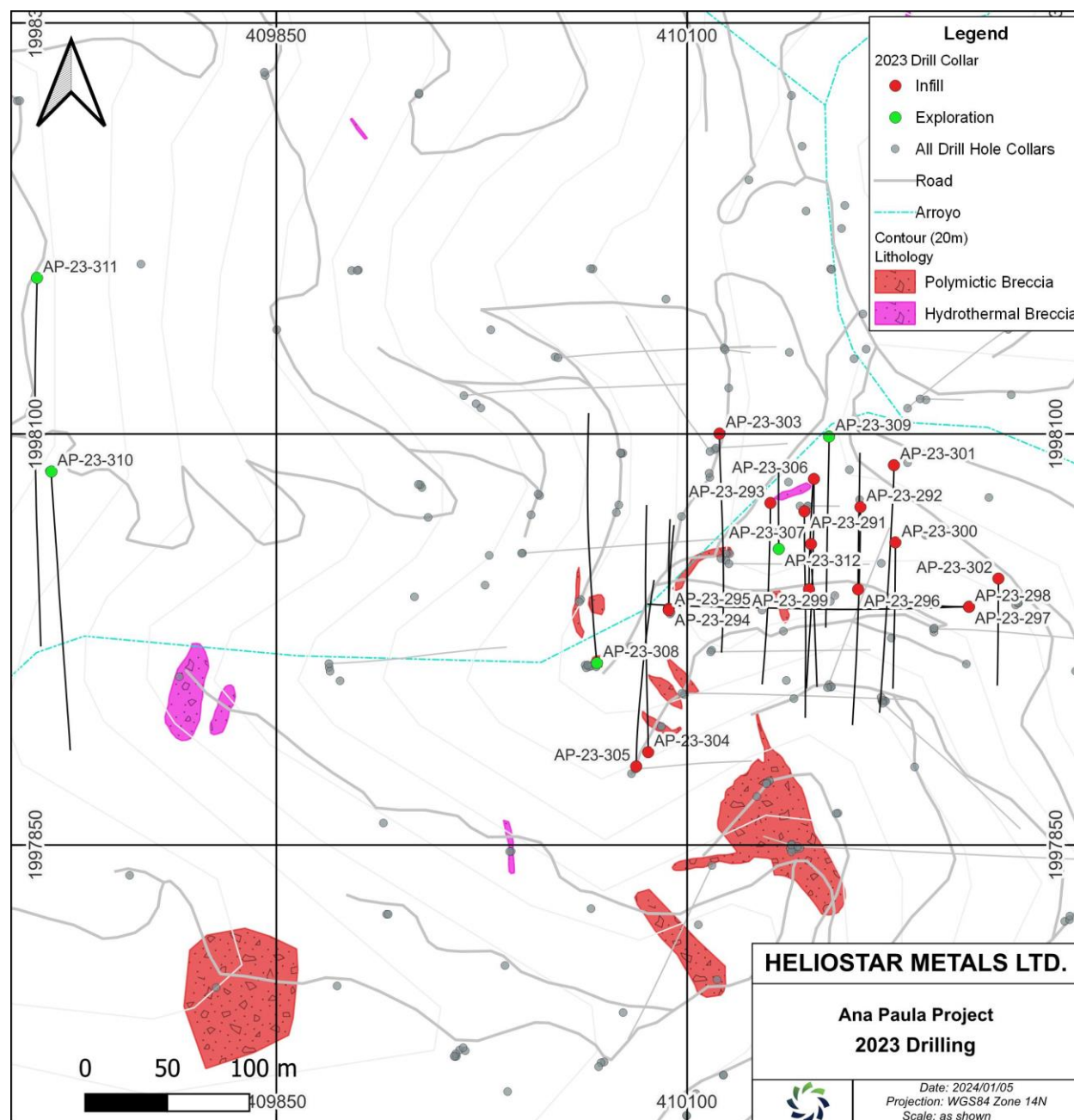
Figure 9-1: 2023 Drill Plan
