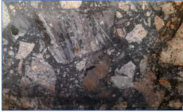
(a) (left): Polymictic Breccia illustrating higher amount of matrix (about 20% volume of breccia) with a strong black rock flour component. Note felsic clast in upper right quadrant with irregular borders indicative of juvenile material. From AP-12-162 at 135 m depth. (b) (right): Polymictic Breccia illustrating lesser amount of matrix (about 10% volume of breccia) with more igneous component. From AP-23-291 at 134 m depth.
