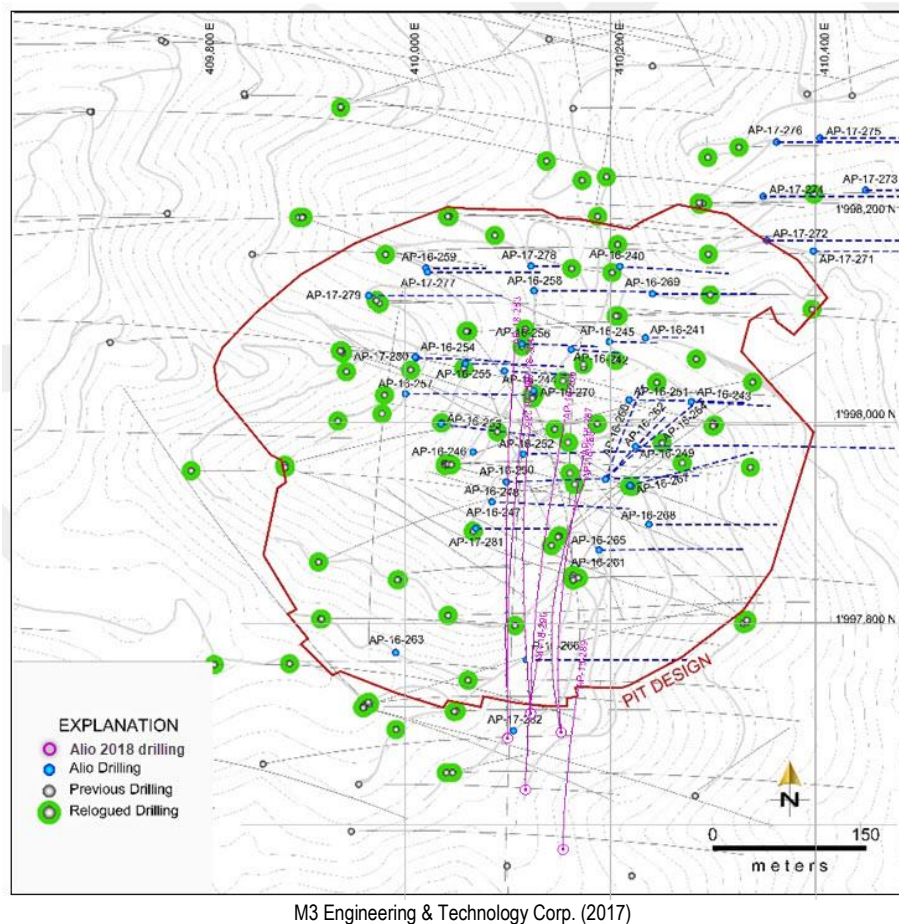
Figure 6-8: Map Showing the Re-Logged Drill holes at Pit Design Area
