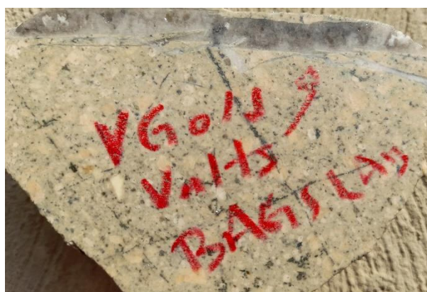
Figure 7-37: V5 Grey Quartz Veinlet (Photo 30)
