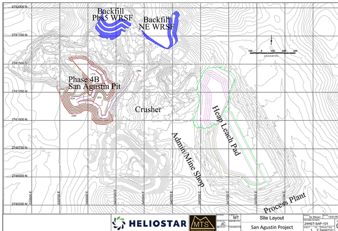
Figure 18-1: Infrastructure Layout Plan
