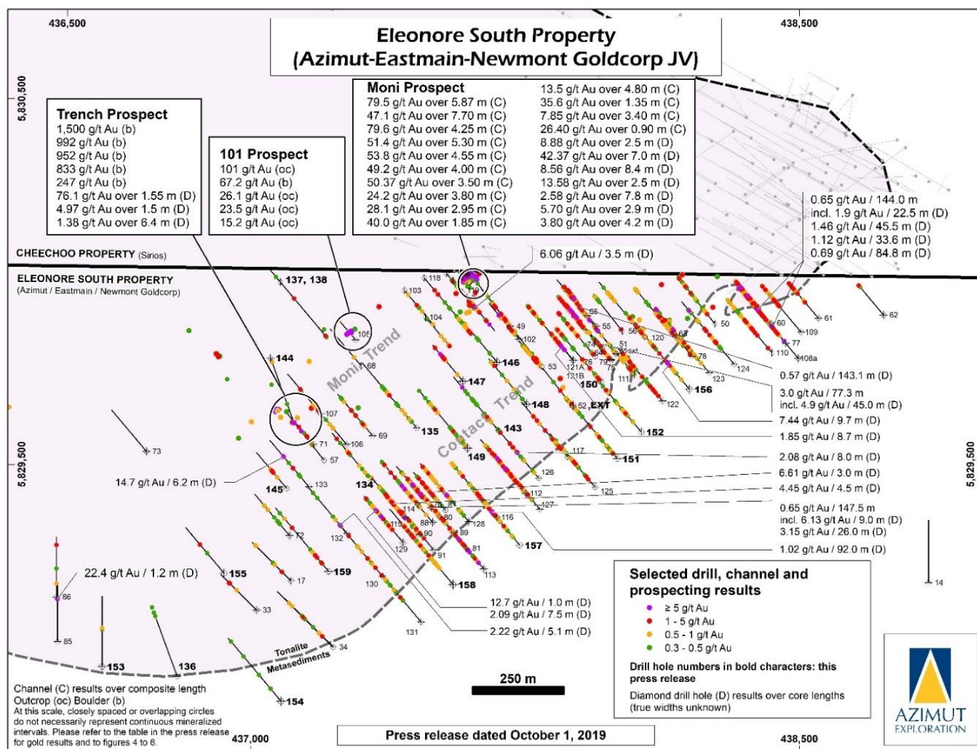
Figure 12: Details of the Moni and Contact trends along the tonalite-metasedimentary contact showing selected drill, channel and prospecting results.
