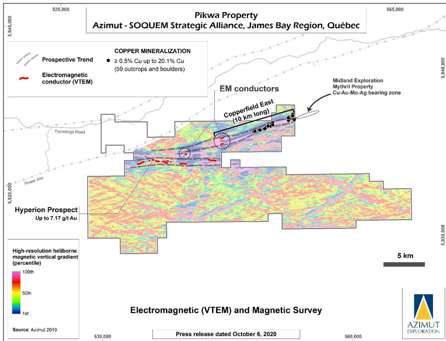
Figure 10: Geophysical signature of the Copperfield Trend on the Pikwa Property.
