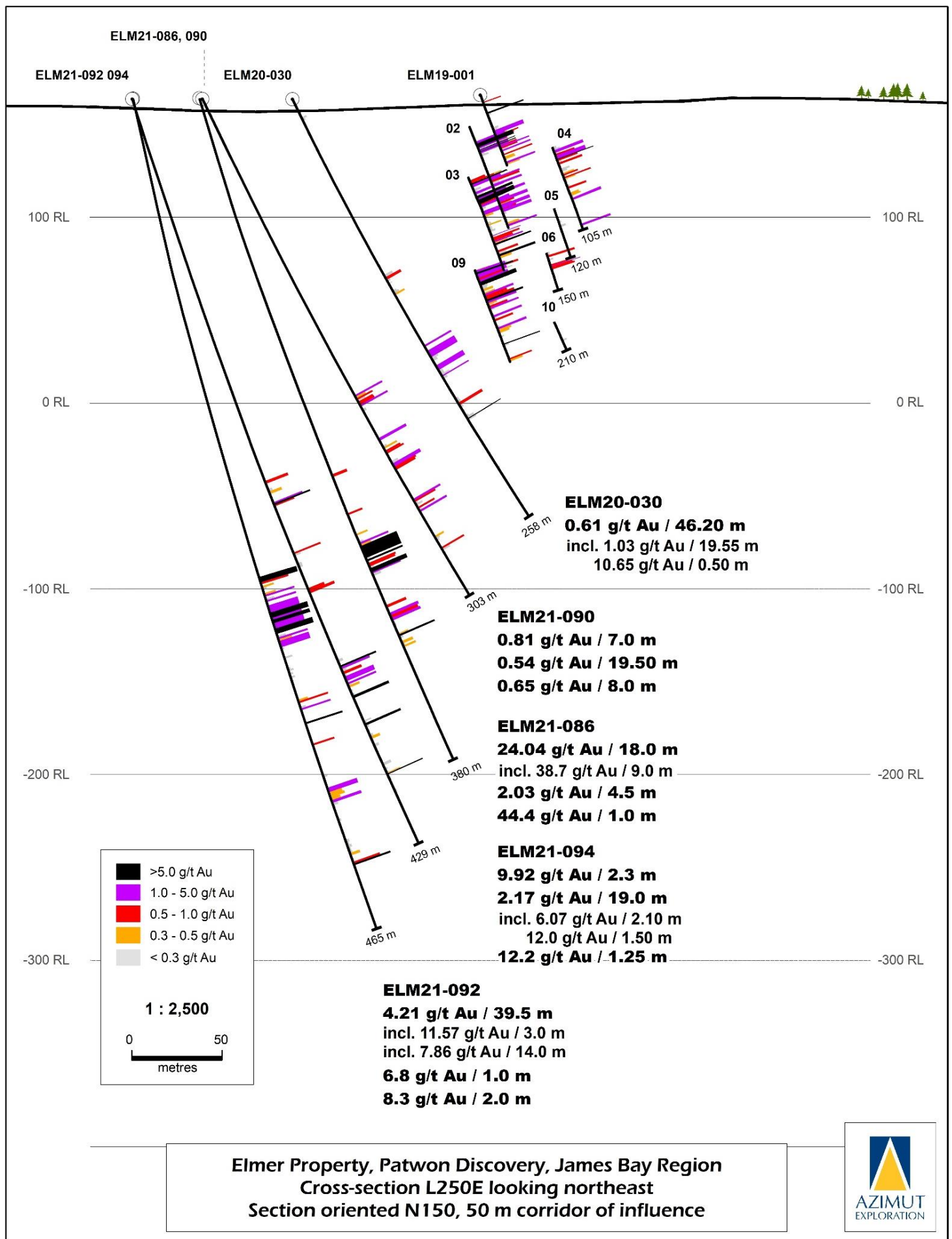
Figure 6: Cross section L250E through the Patwon Zone (looking NE).
