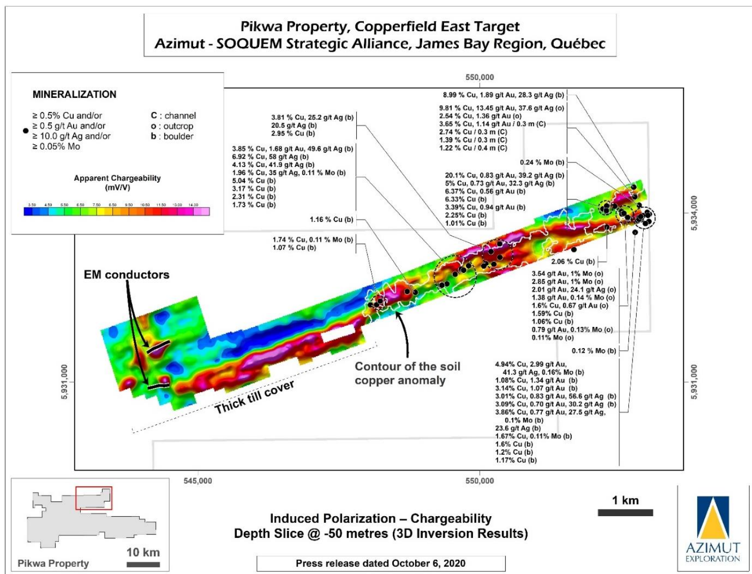
Figure 11: IP-chargeability footprint of the Copperfield East Target on the Pikwa Property.
