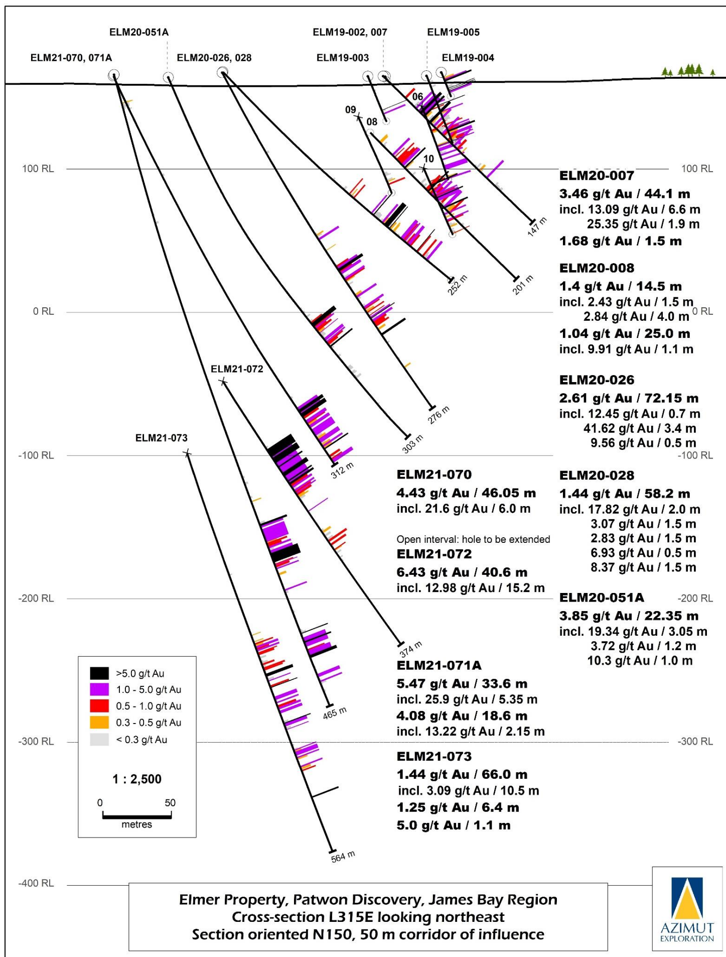
Figure 7: Cross section L315E through the Patwon Zone (looking NE).
