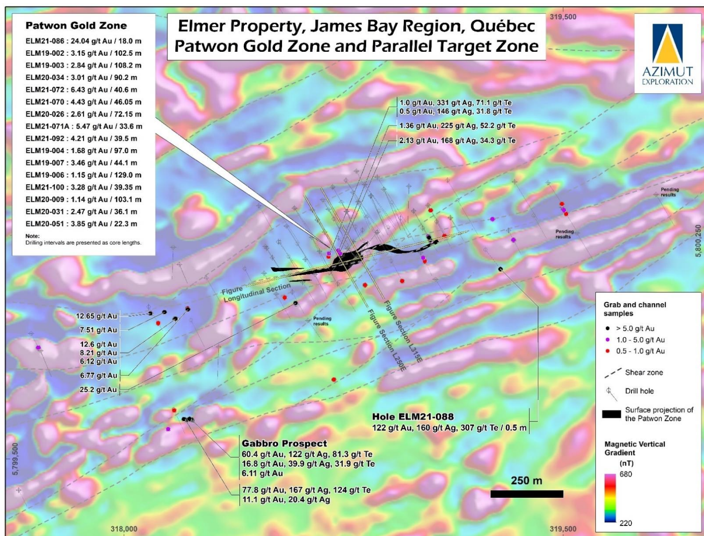
Figure 4: Close-up of the priority corridor on the Elmer Property showing drill hole traces, significant exploration results, the surface projection of the Patwon Zone, and the locations of the longitudinal section and cross-sections in the following figures.
