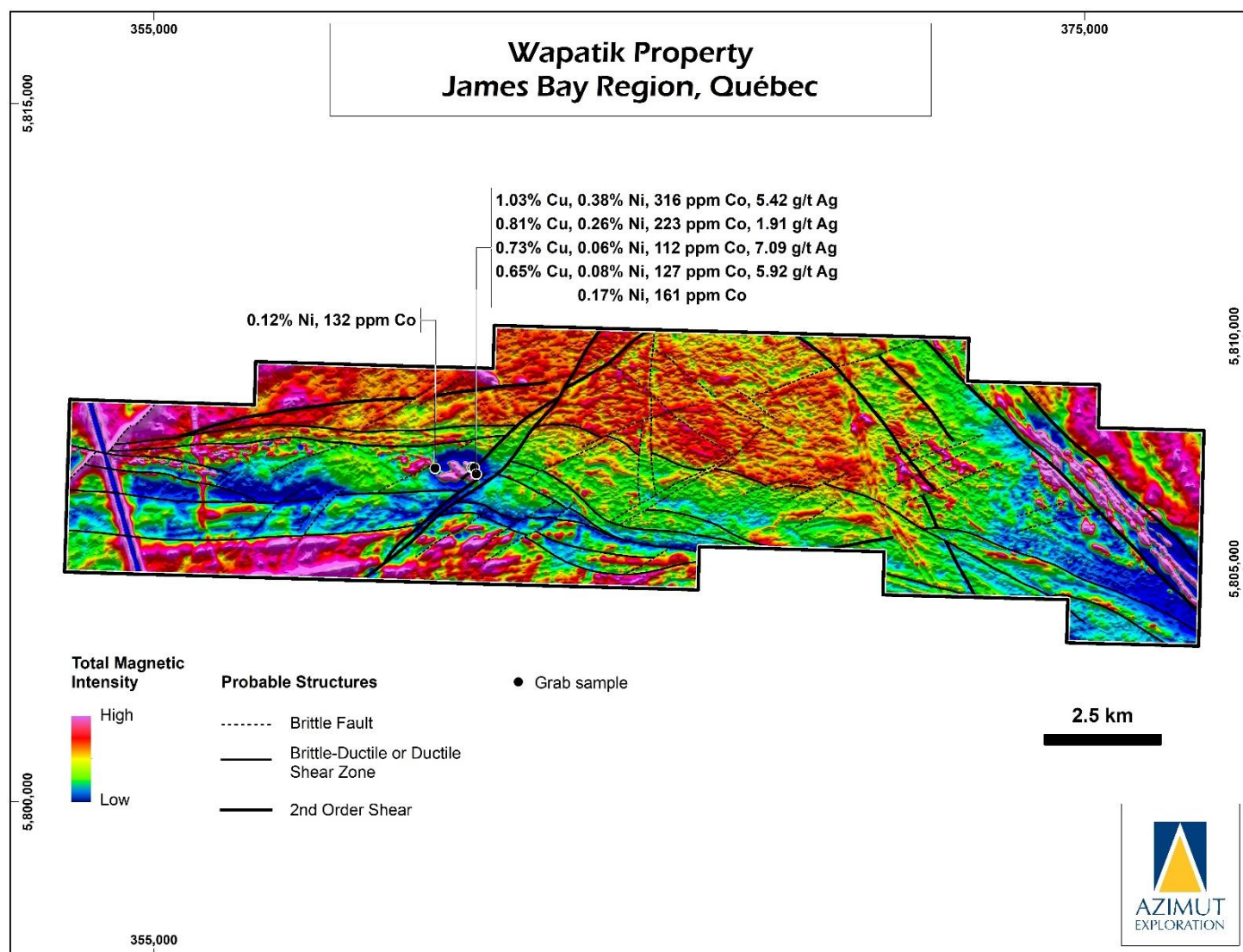
Figure 9: Magnetic map of the Wapatik Property showing structures and the locations of known mineralization.
