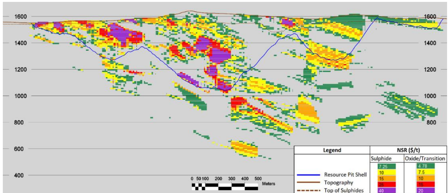
Figure 14-10: Long-Section A-A' through the Resource Block Model
