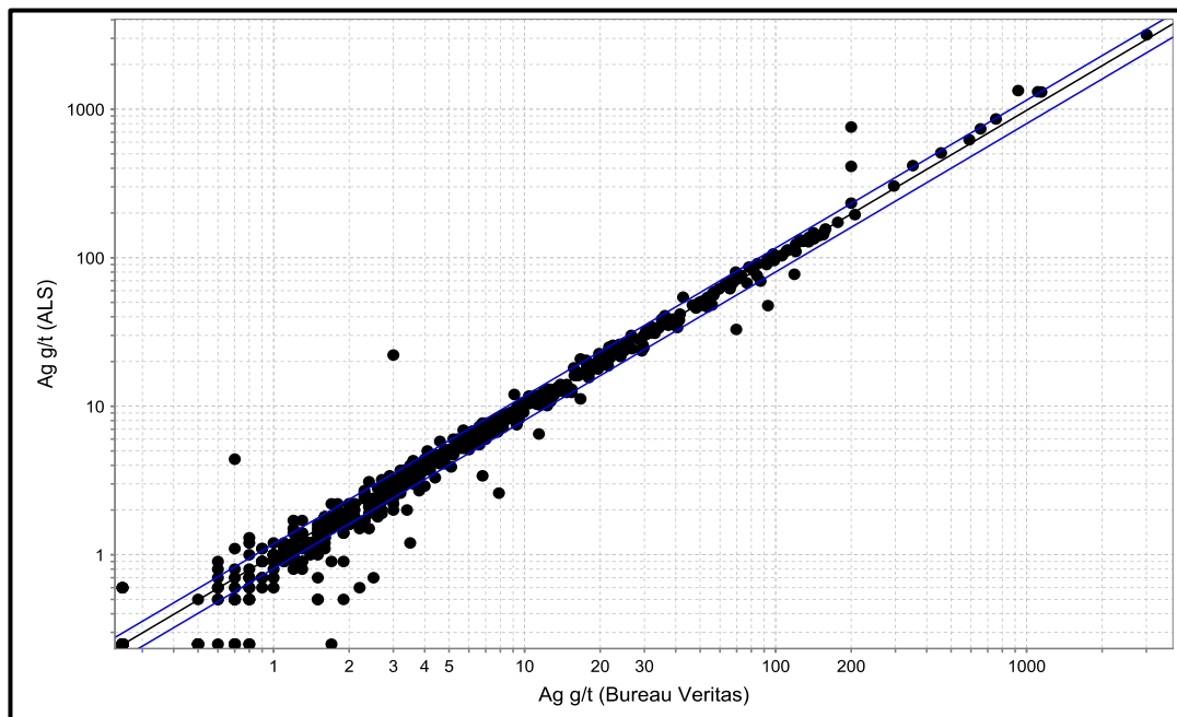
Figure 11-3: Comparison of Silver from Pulp Duplicate Check Assays
