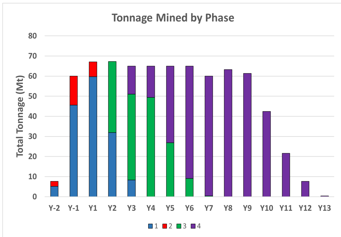
Figure 16-7: Tonnage Mined by Phase
