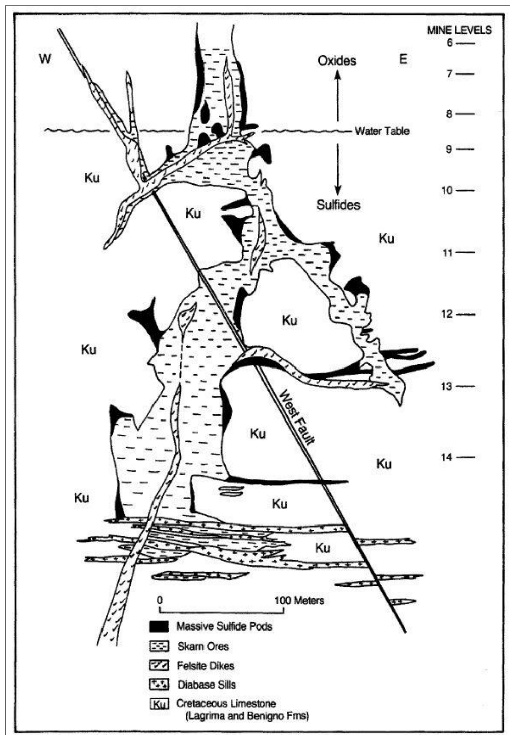
Figure 8-2: Cross-Section through the Carbonate-Hosted Replacement Deposit (Sulphide Manto/Chimney) at the San Antonio Mine in the Santa Eulalia Mining District
