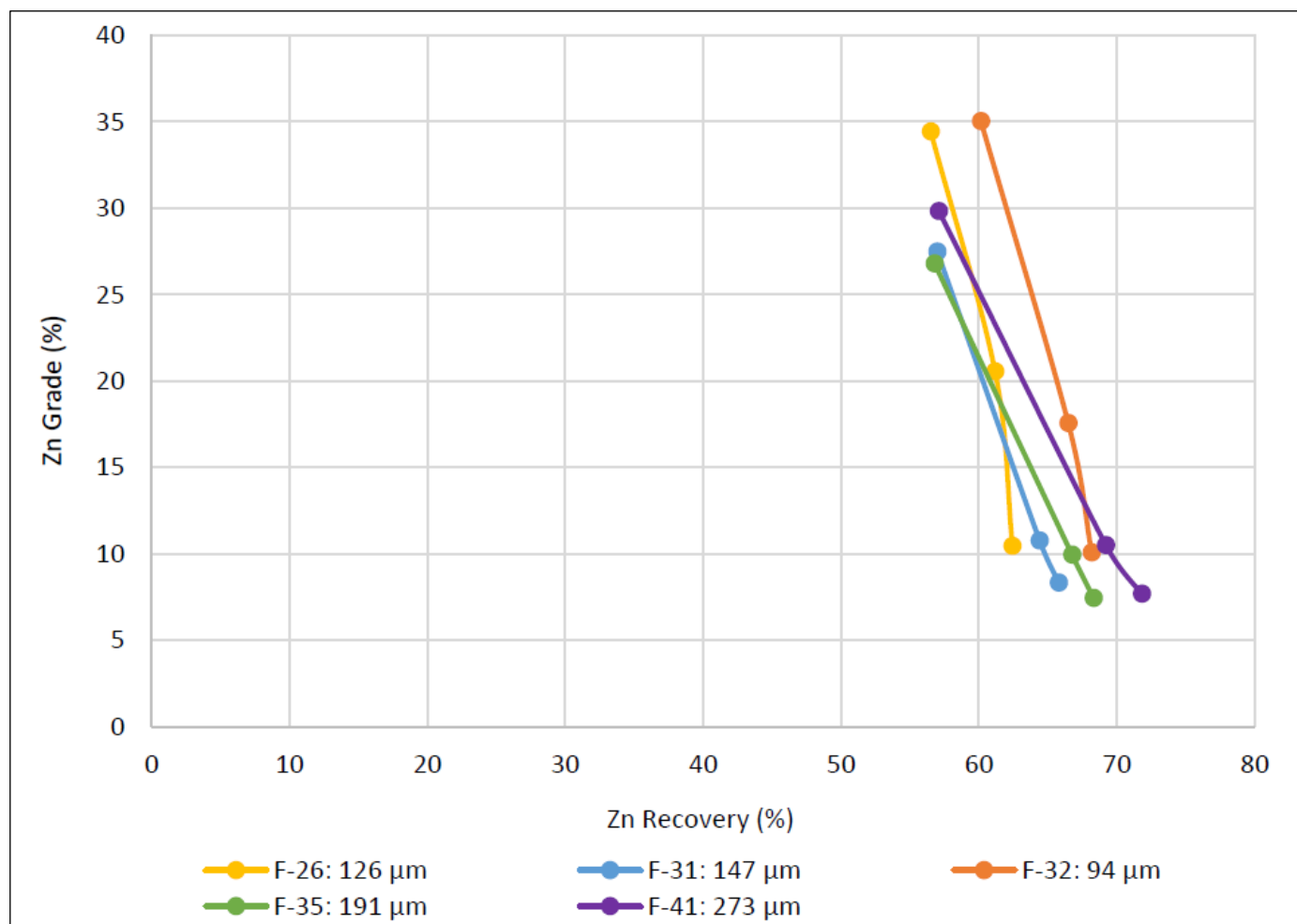
Figure 13-12: VOLC Master Composite Primary Grind vs. Recovery Sensitivity (Zinc Grade Recovery Curves)
