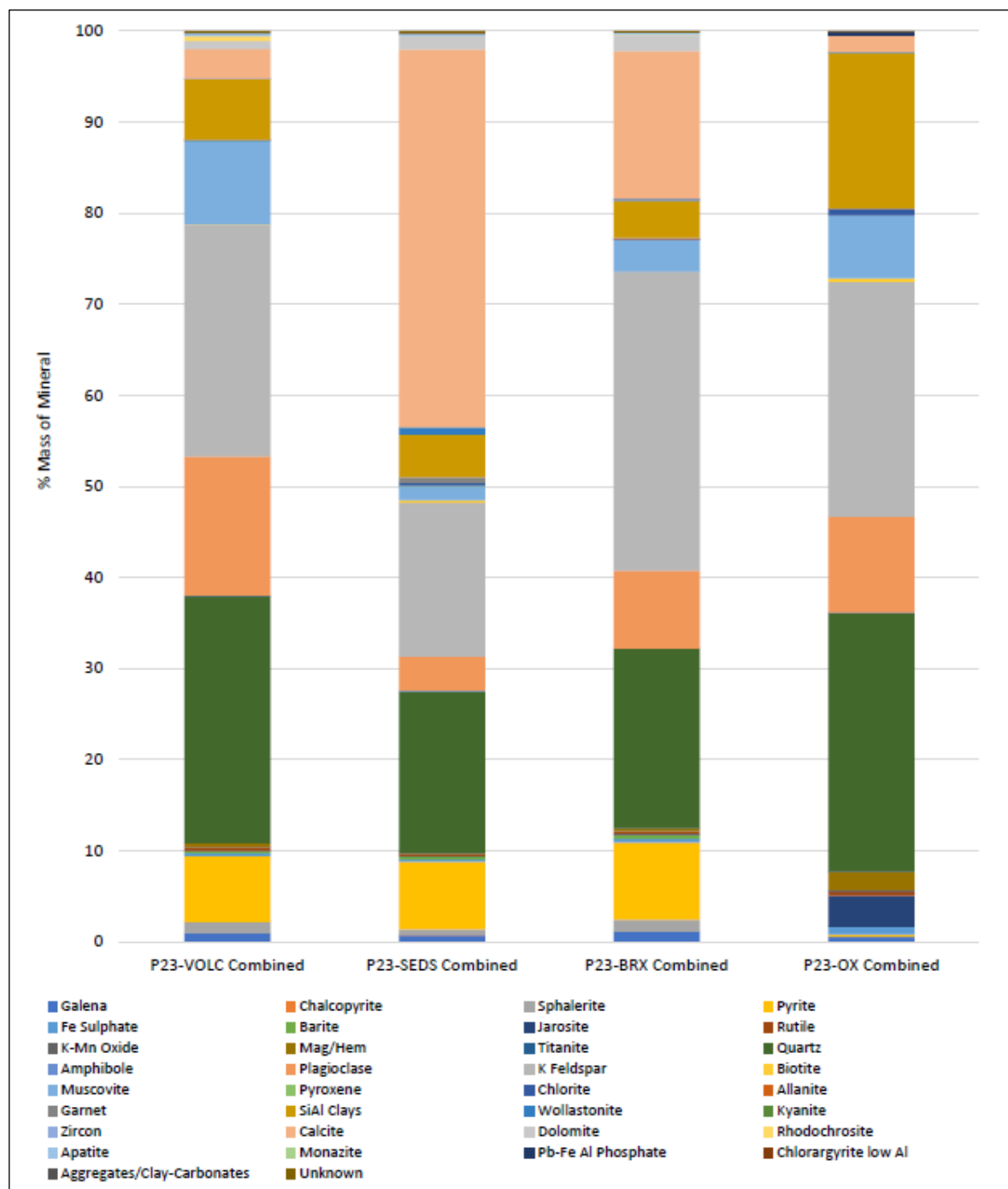
Figure 13-3: Pit 23 Lithology Composites Modal Mineralogy
