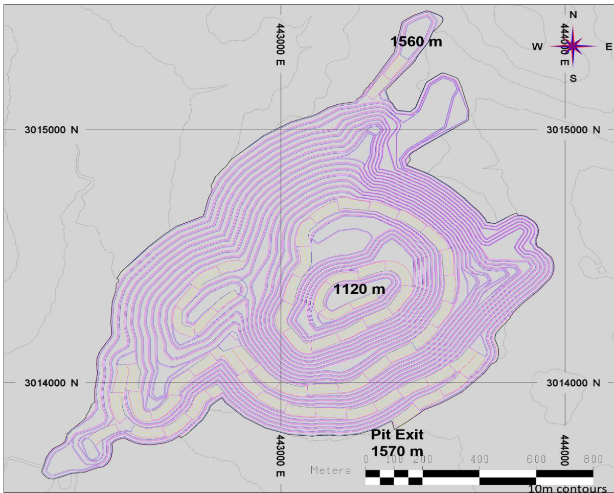
Figure 16-6: Phase 4 Layout
