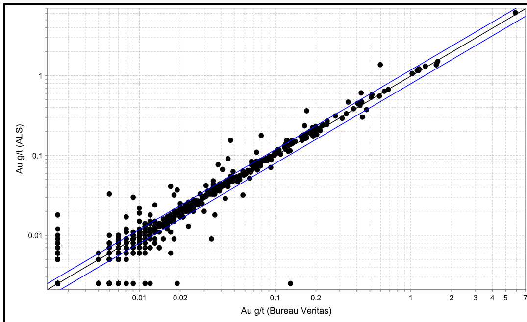
Figure 11-4: Comparison of Gold from Pulp Duplicate Check Assays
