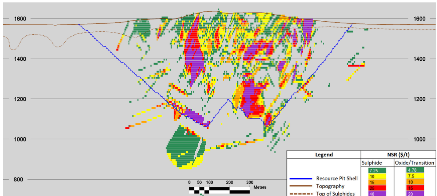
Figure 14-13: Cross-Section D-D' through the Resource Block Model
