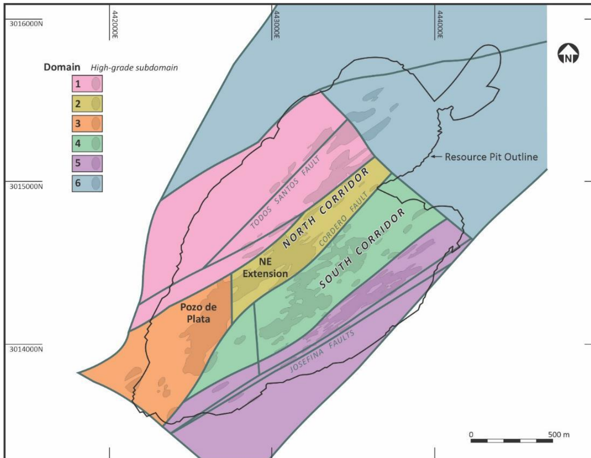
Figure 14-6: Estimation Domains in the Cordero Main Area Where Resources were Estimated
