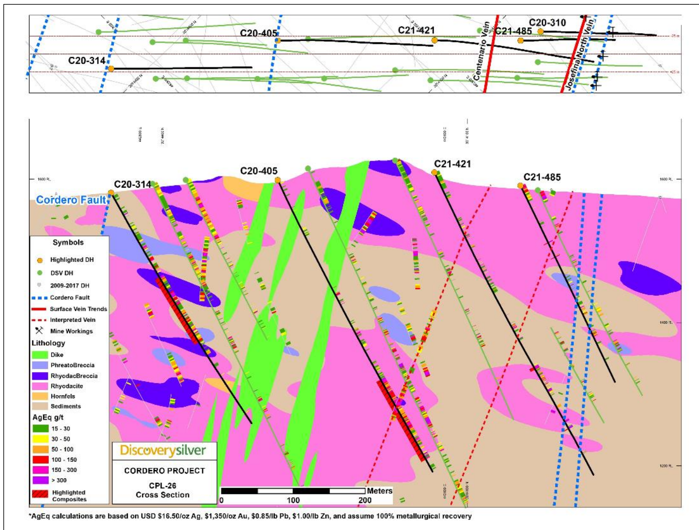
Figure 10-7: Cross-Section CPL-26 showing Geological Interpretation and Silver Equivalent Grades
