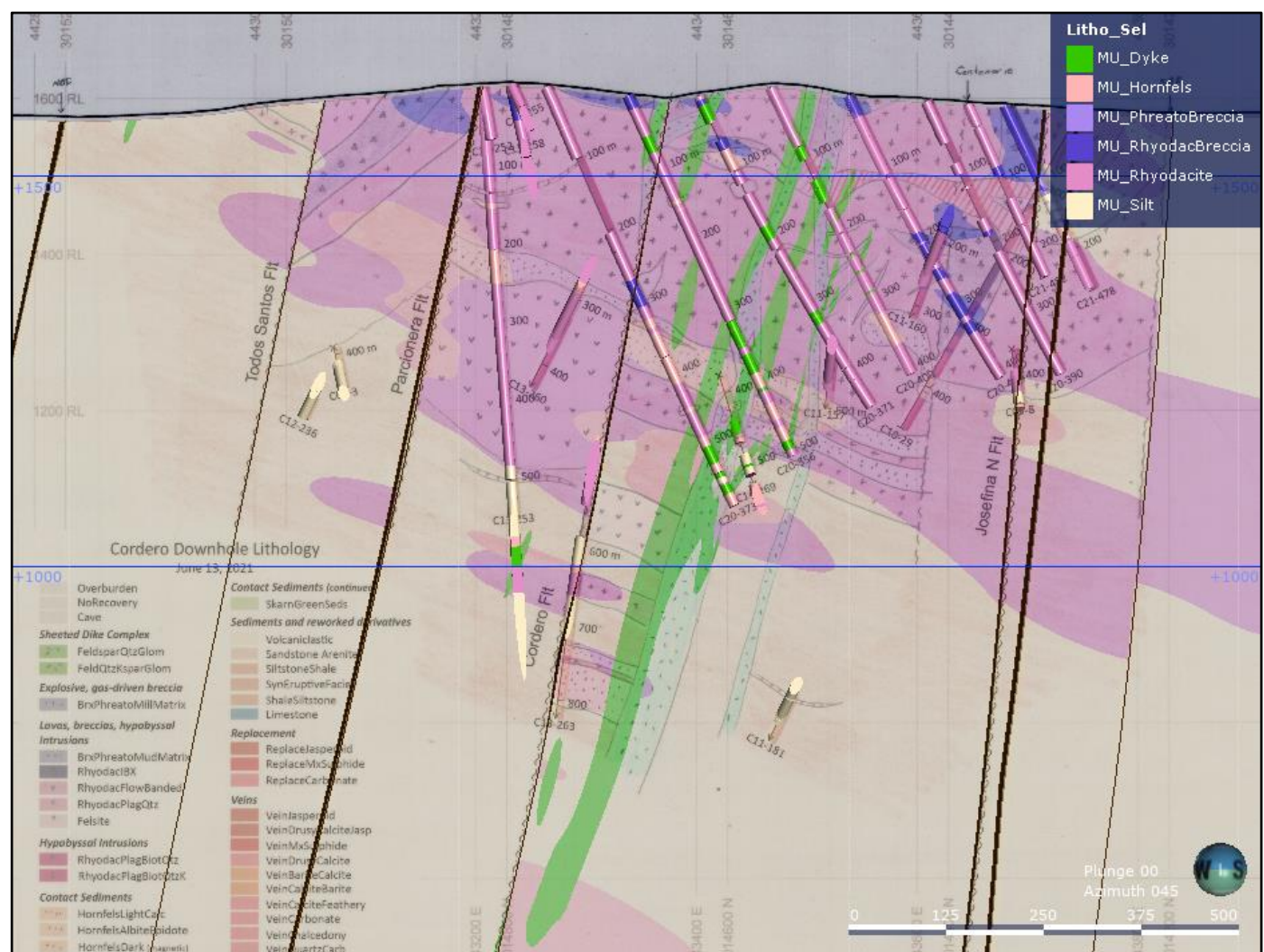
Figure 14-3: Example of a Northeast-Facing Lithology Cross-Section
