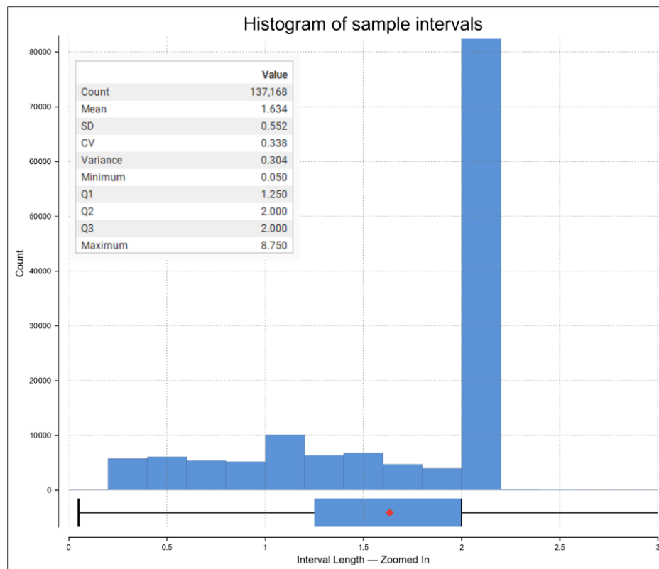
Figure 14-7: Histogram of Interval Length
