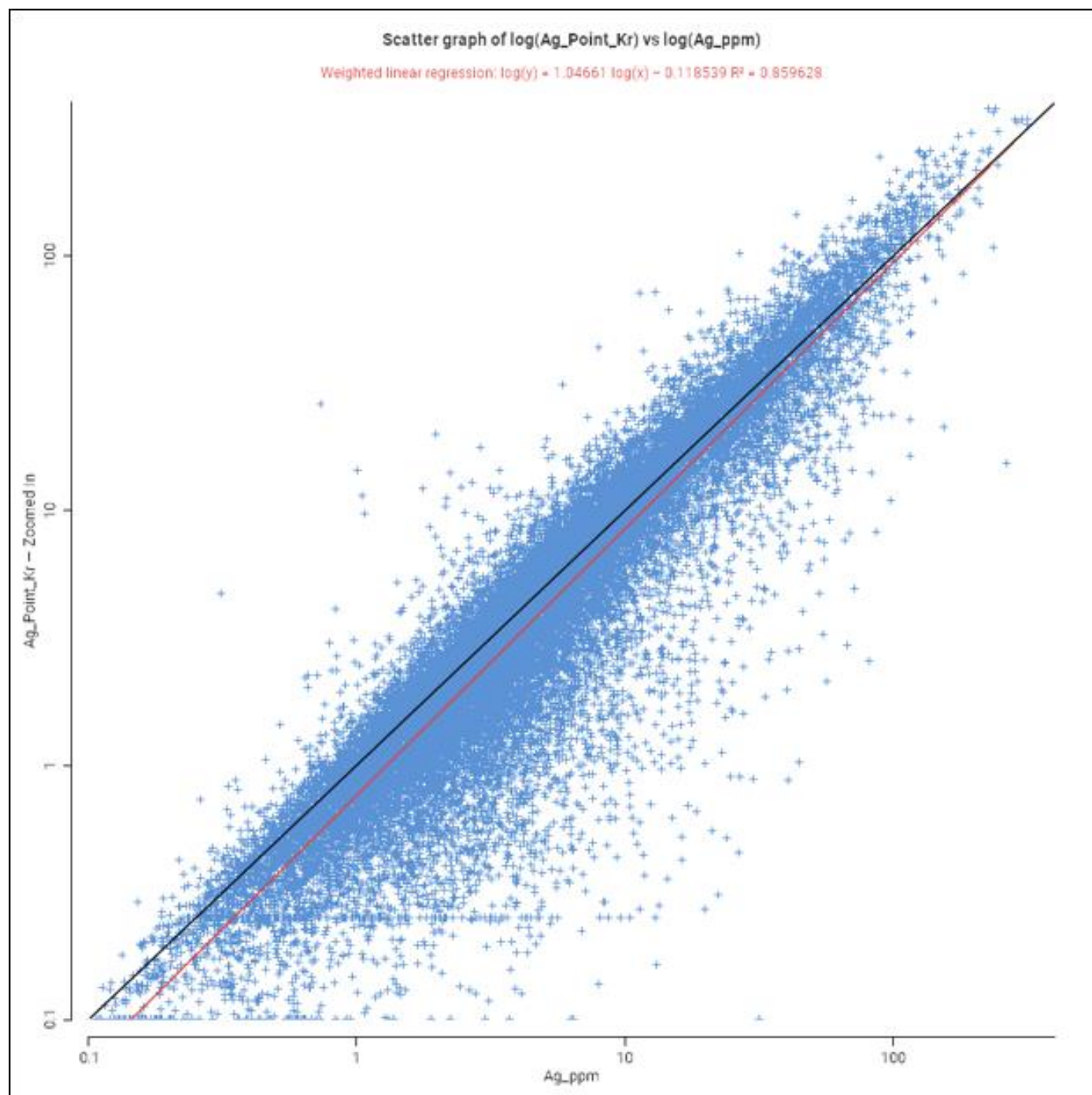
Figure 14-15: Scatterplot of Silver Composites vs. Silver Block Estimates
