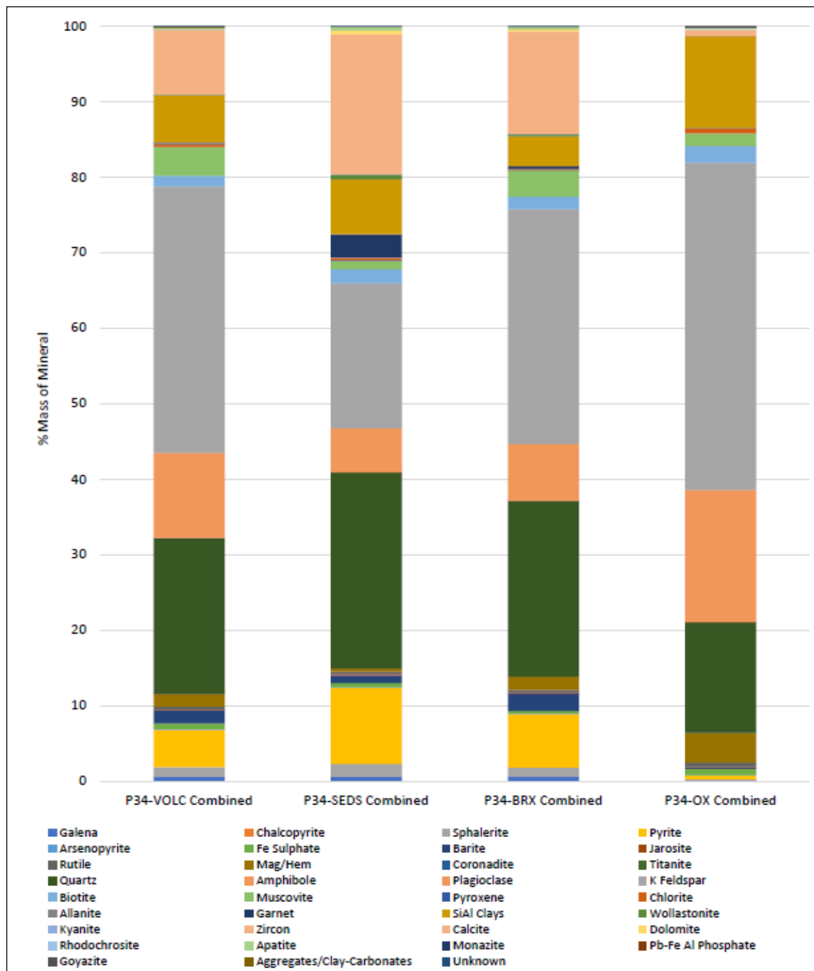
Figure 13-5: Pit 34 Lithology Composites Modal Mineralogy
