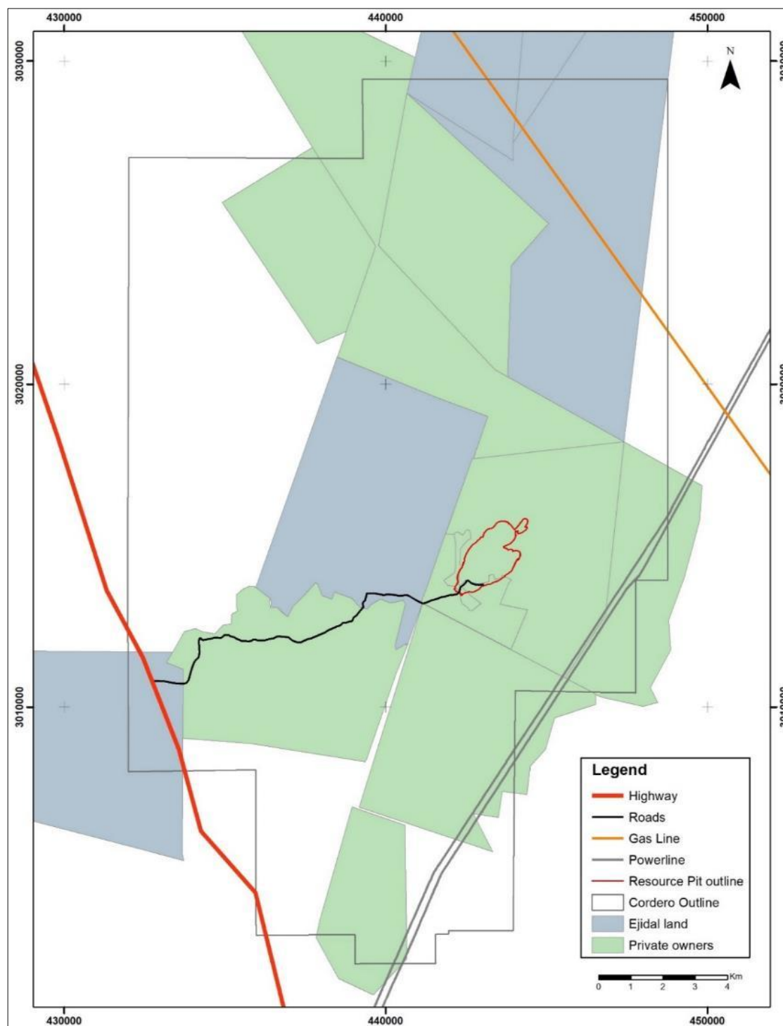
Figure 20-2: Property Rights at Cordero Project
