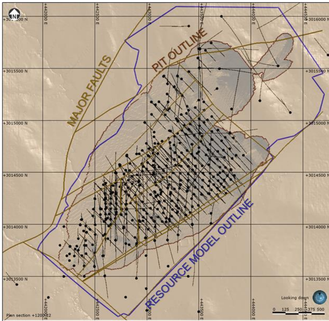
Figure 14-1: Drill Hole Locations
