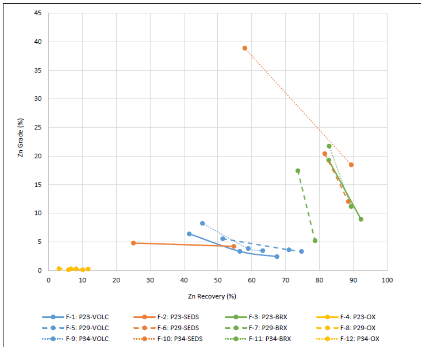
Figure 13-8: Lithology/Pit Composite Zinc Grade Versus Zinc Recovery
