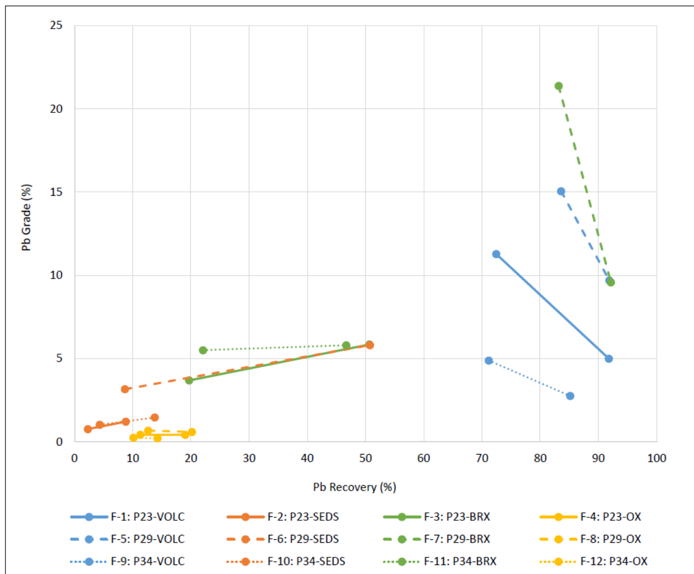
Figure 13-6: Lithology/Pit Composites Lead Grade Recovery Curves
