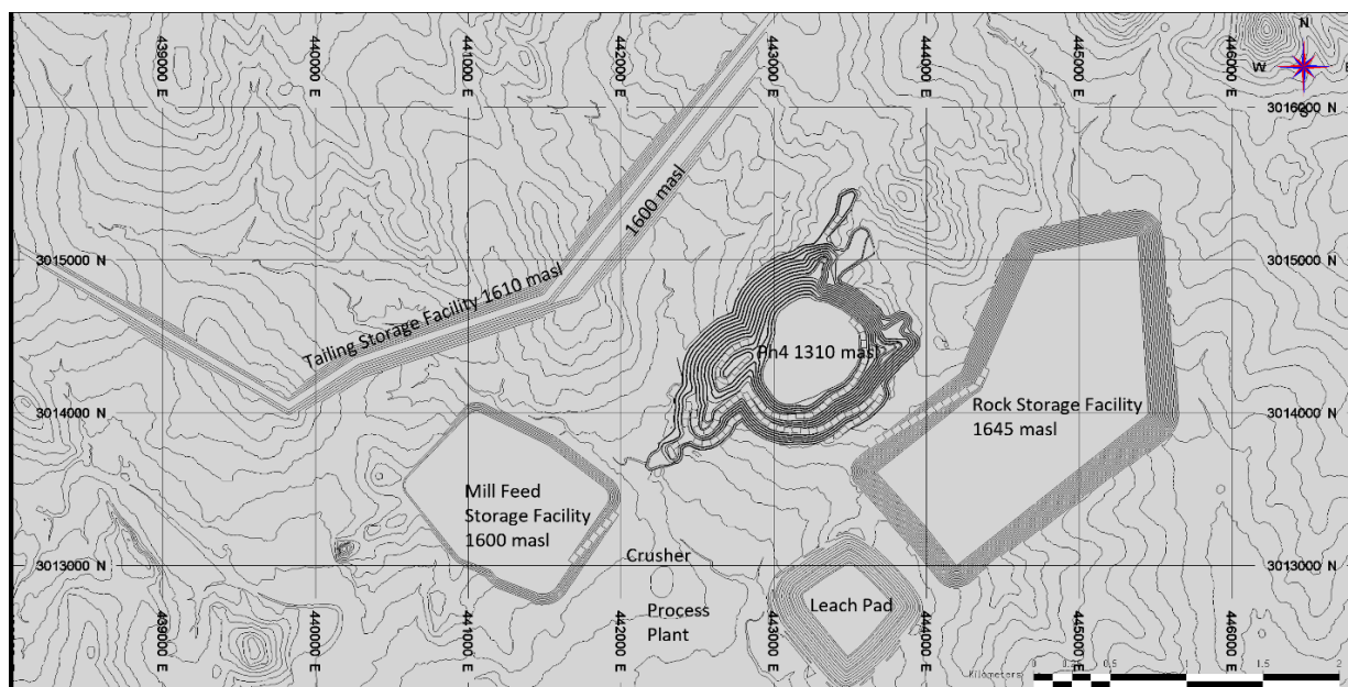
Figure 16-15: End of Year 9
