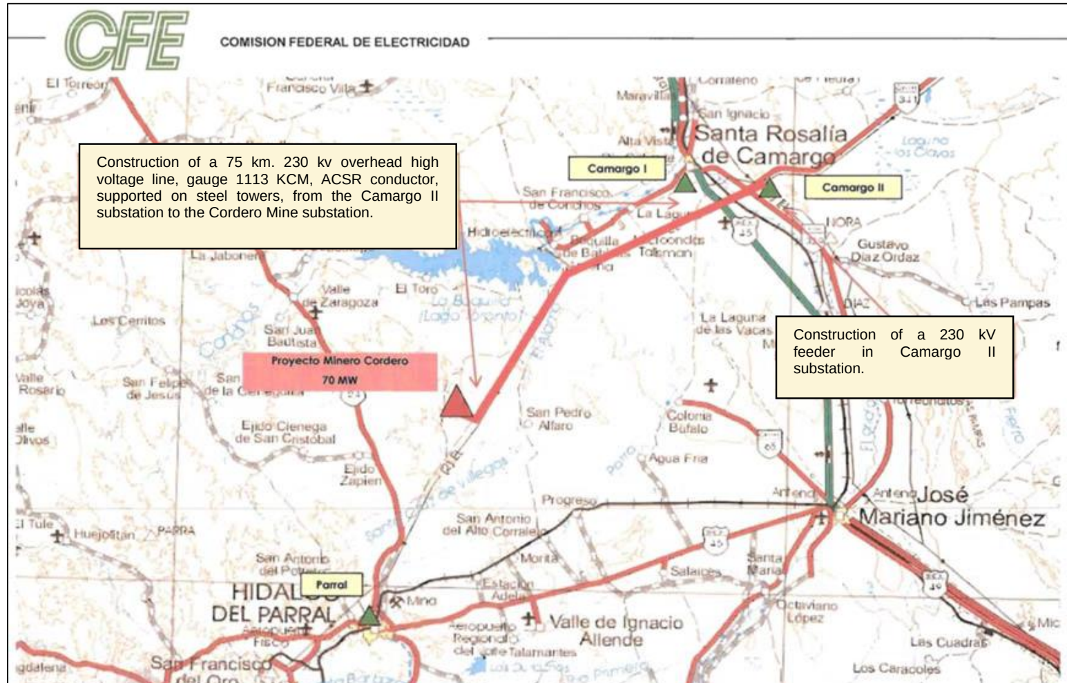
Figure 18-3: Proposed CFE 230 kV Transmission Line from Camargo II to Cordero Mine Site
