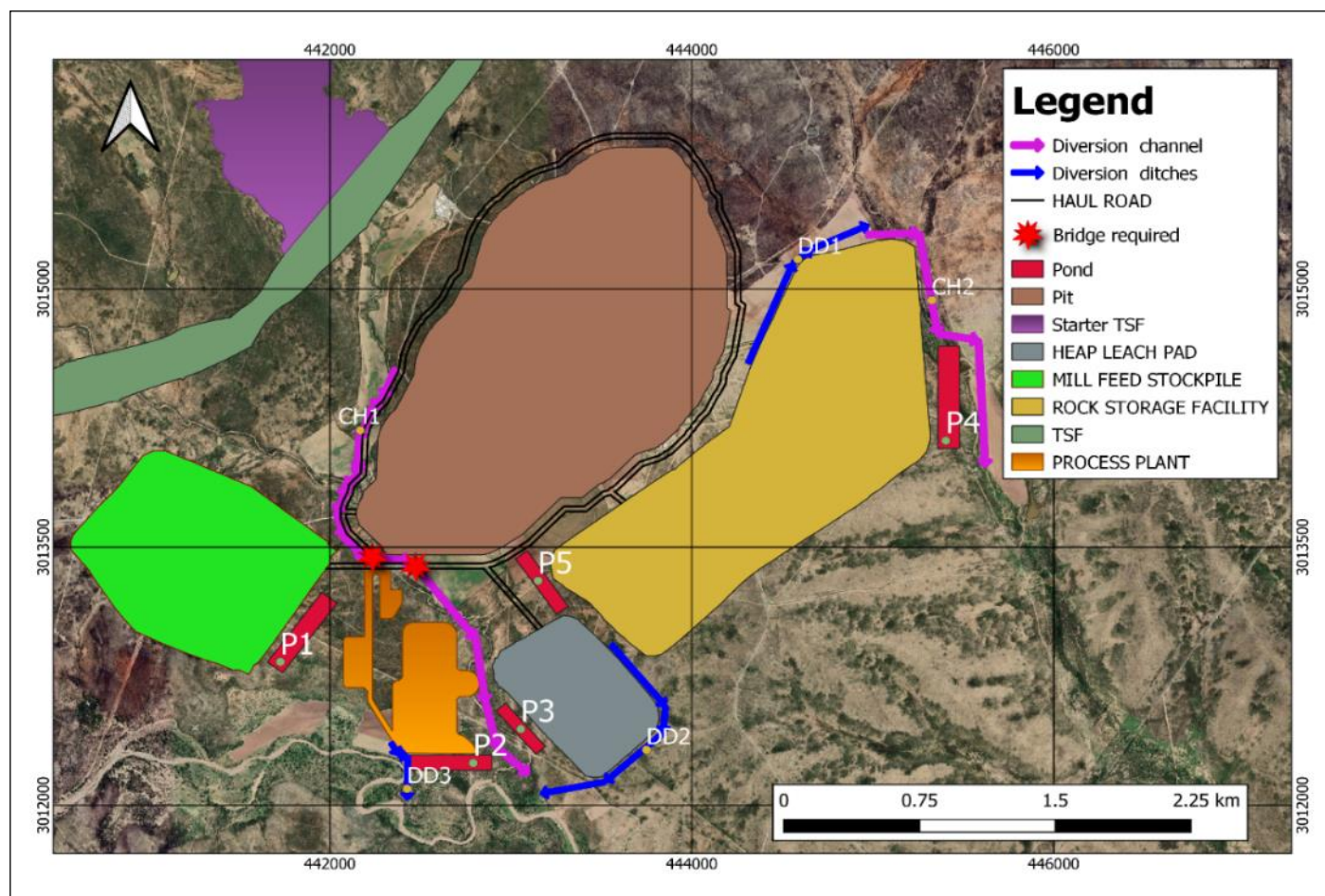
Figure 18-12: Diversion Channels, Ditches and Ponds
