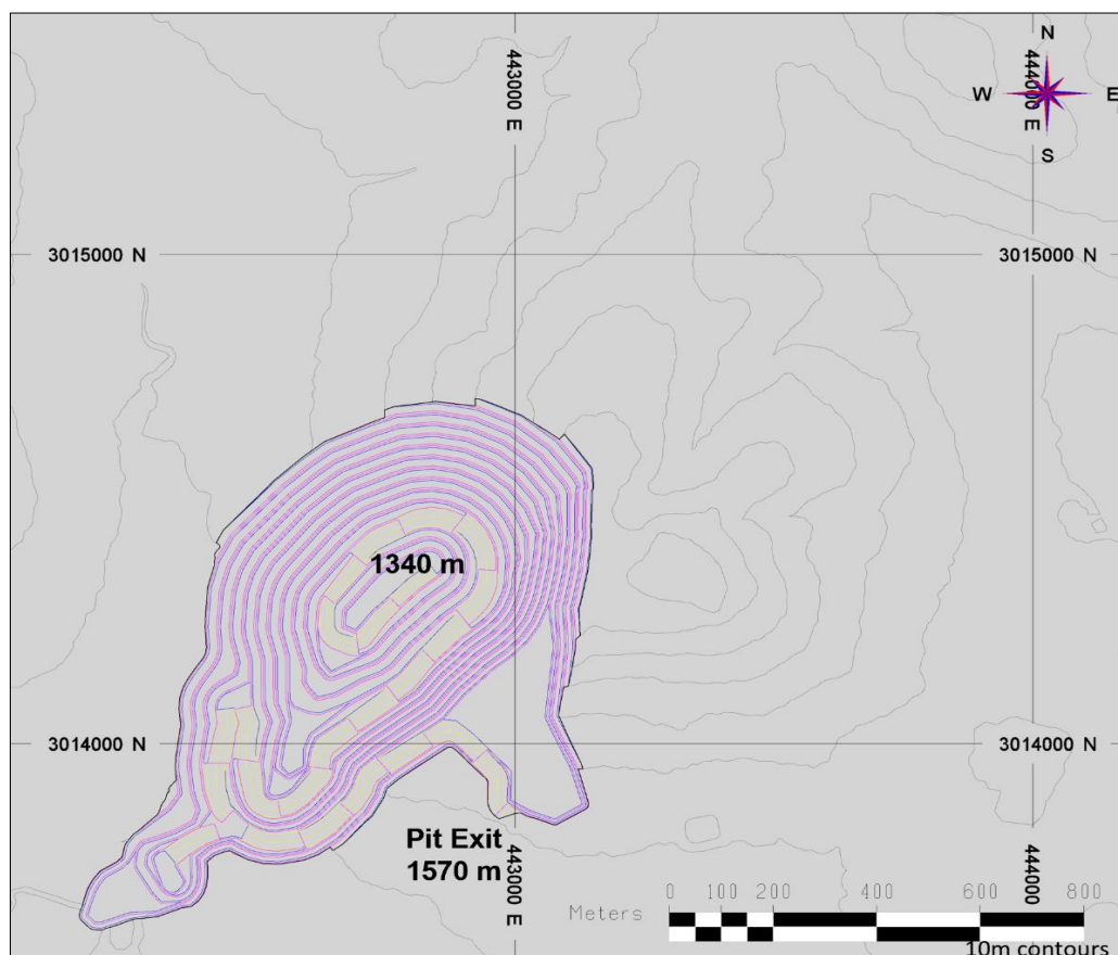
Figure 16-3: Phase 1 Layout
