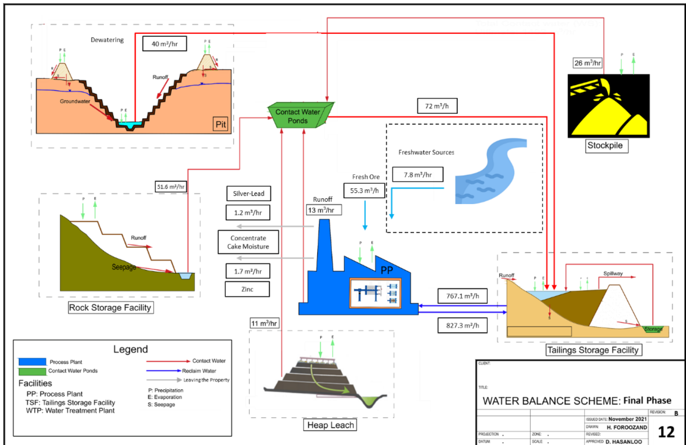
Figure 18-15: Schematic of Final Phase Site-Wide Water Balance
