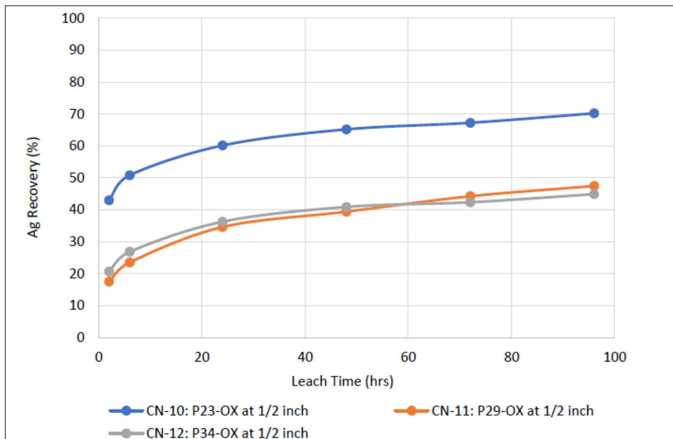
Figure 13-21: Lithology/Pit Composite ½" Bottle Roll Test Silver Kinetics Curves
