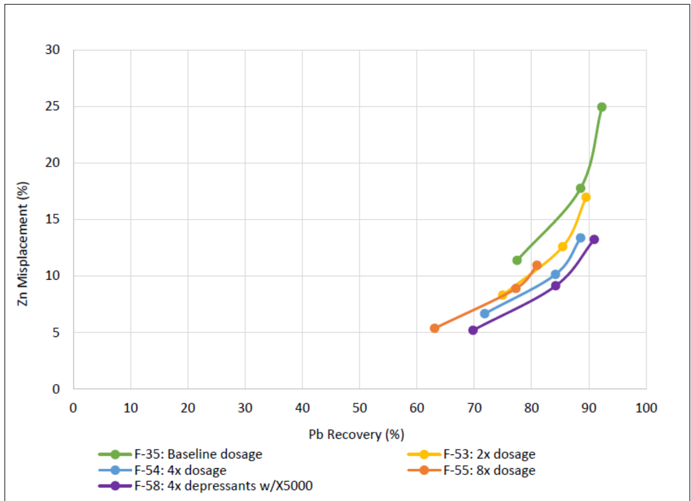
Figure 13-15: VOLC Master Composite Depressant Sensitivity (Lead-Zinc Selectivity Curves)
