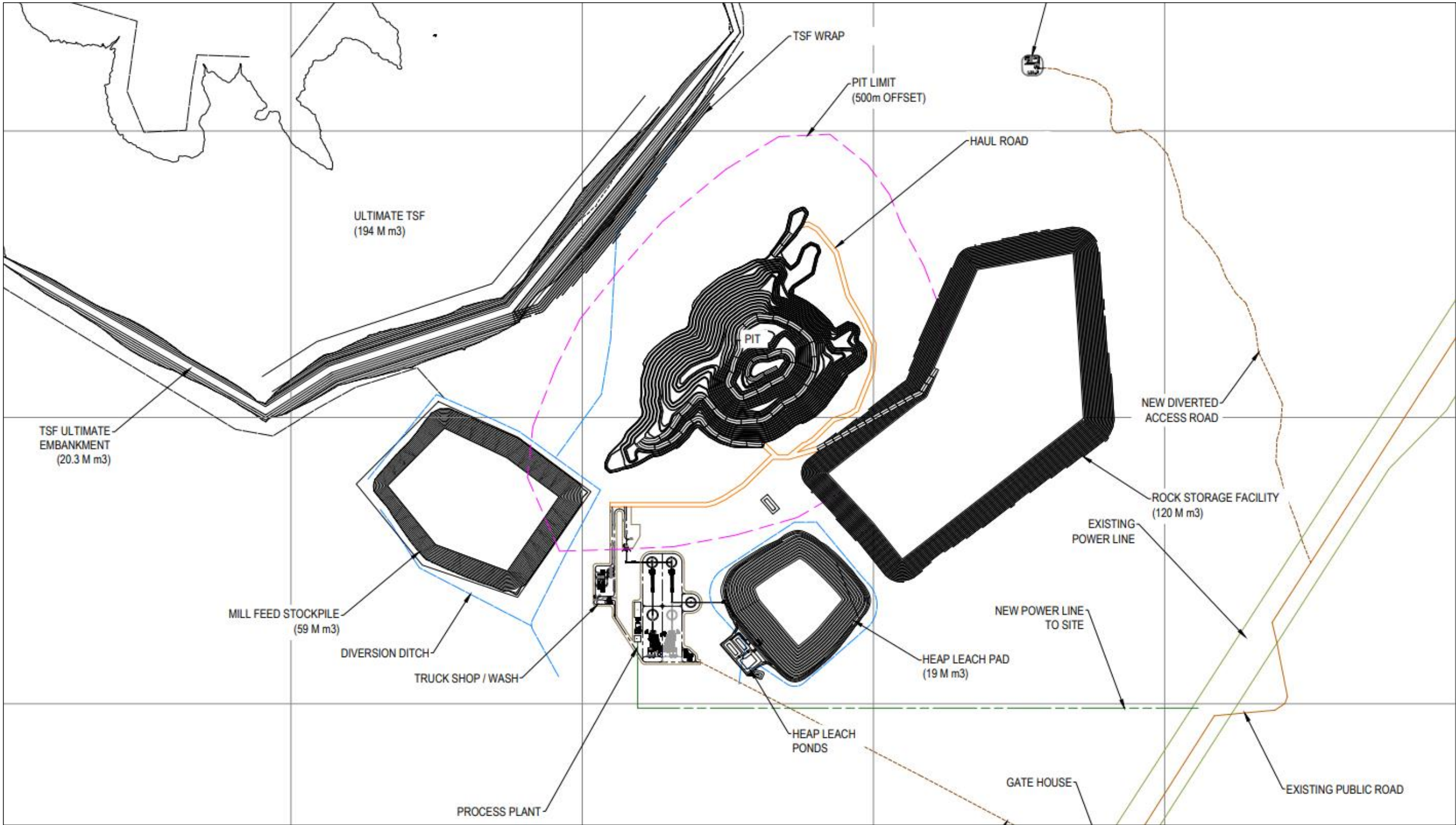
Figure 18-1: Overall Site Layout
