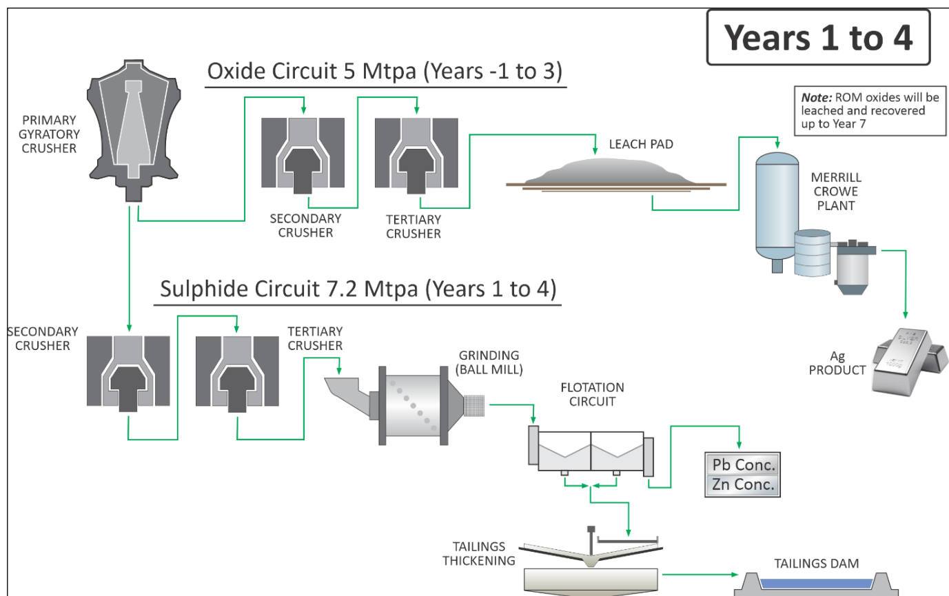
Figure 1-2: Simplified Process Flow Diagram
