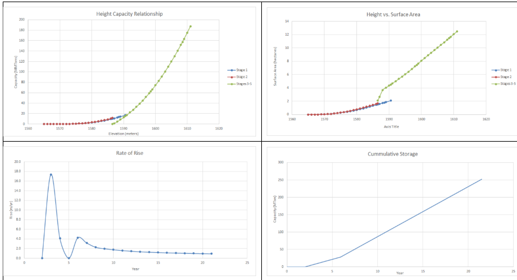
Figure 18-9: Tailings Storage Facility Height vs. Capacity and Rate of Tailings Rise
