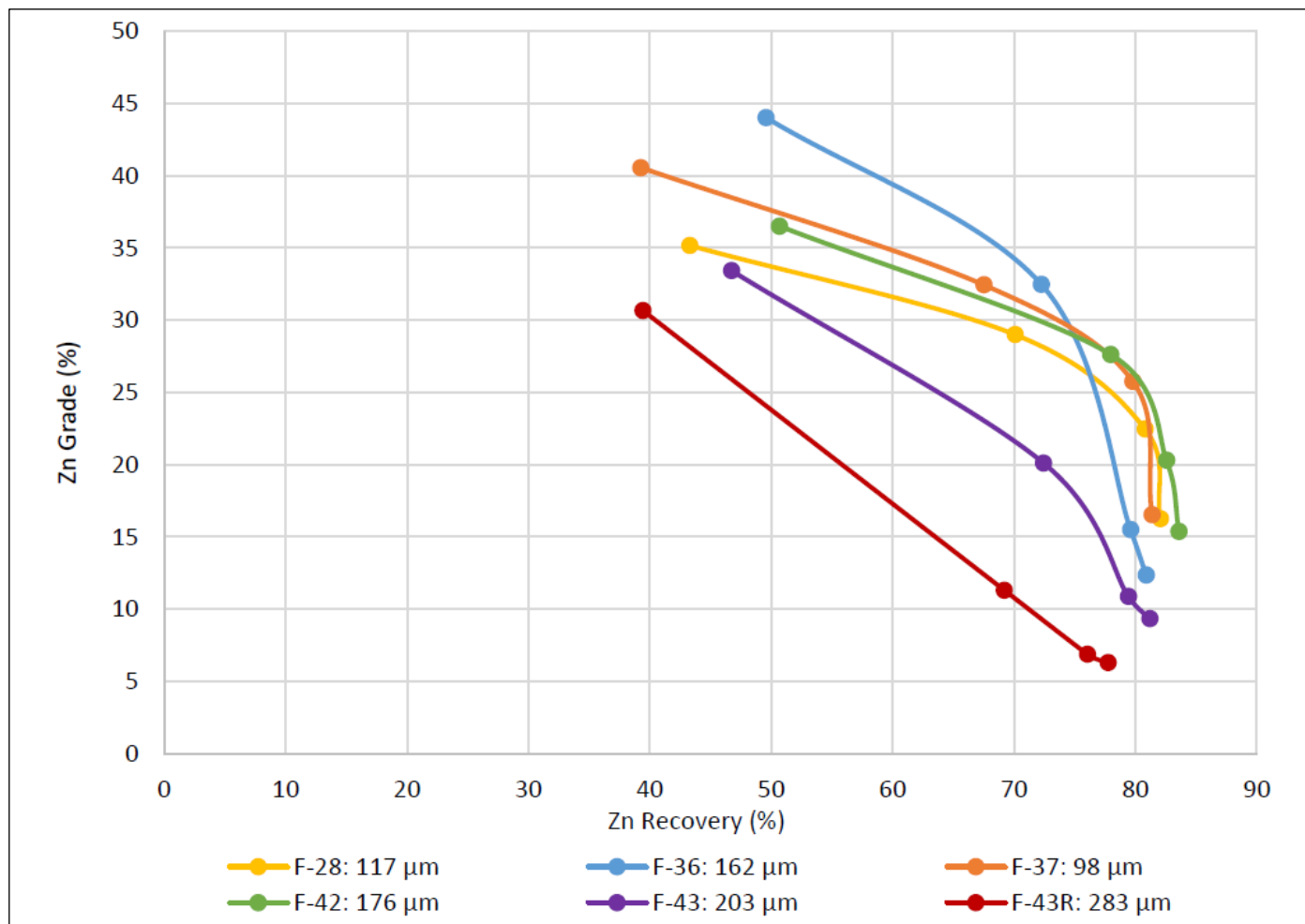
Figure 13-14: SEDS Master Composite Grind vs. Recovery Sensitivity (Zinc Grade vs. Recovery)
