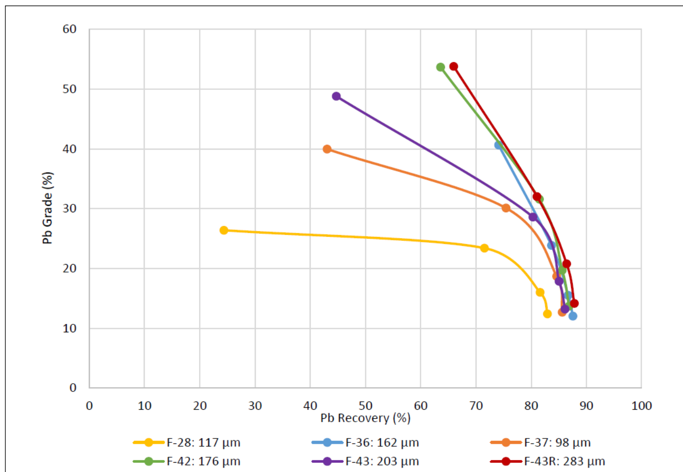
Figure 13-13: SEDS Master Composite Grind vs. Recovery Sensitivity (Lead Grade vs. Recovery)
