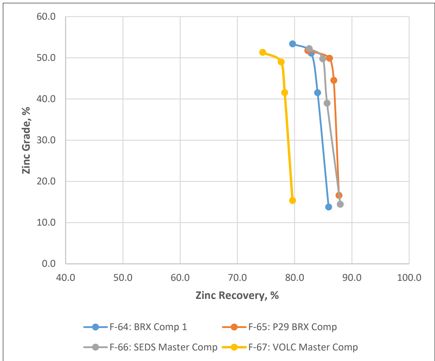
Figure 13-17: Cleaner Circuit Optimization Zinc Grade vs. Recovery Curves
