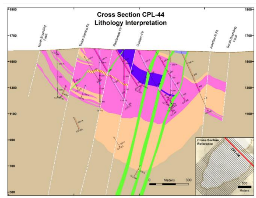
Figure 7-10: Cross-Section CPL-44
