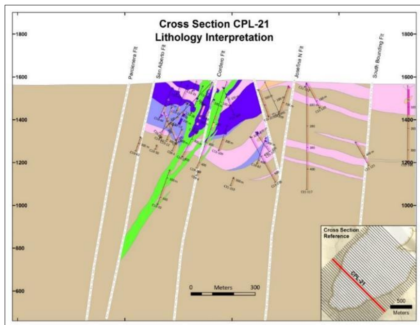
Figure 7-8: Cross-Section CPL-21
