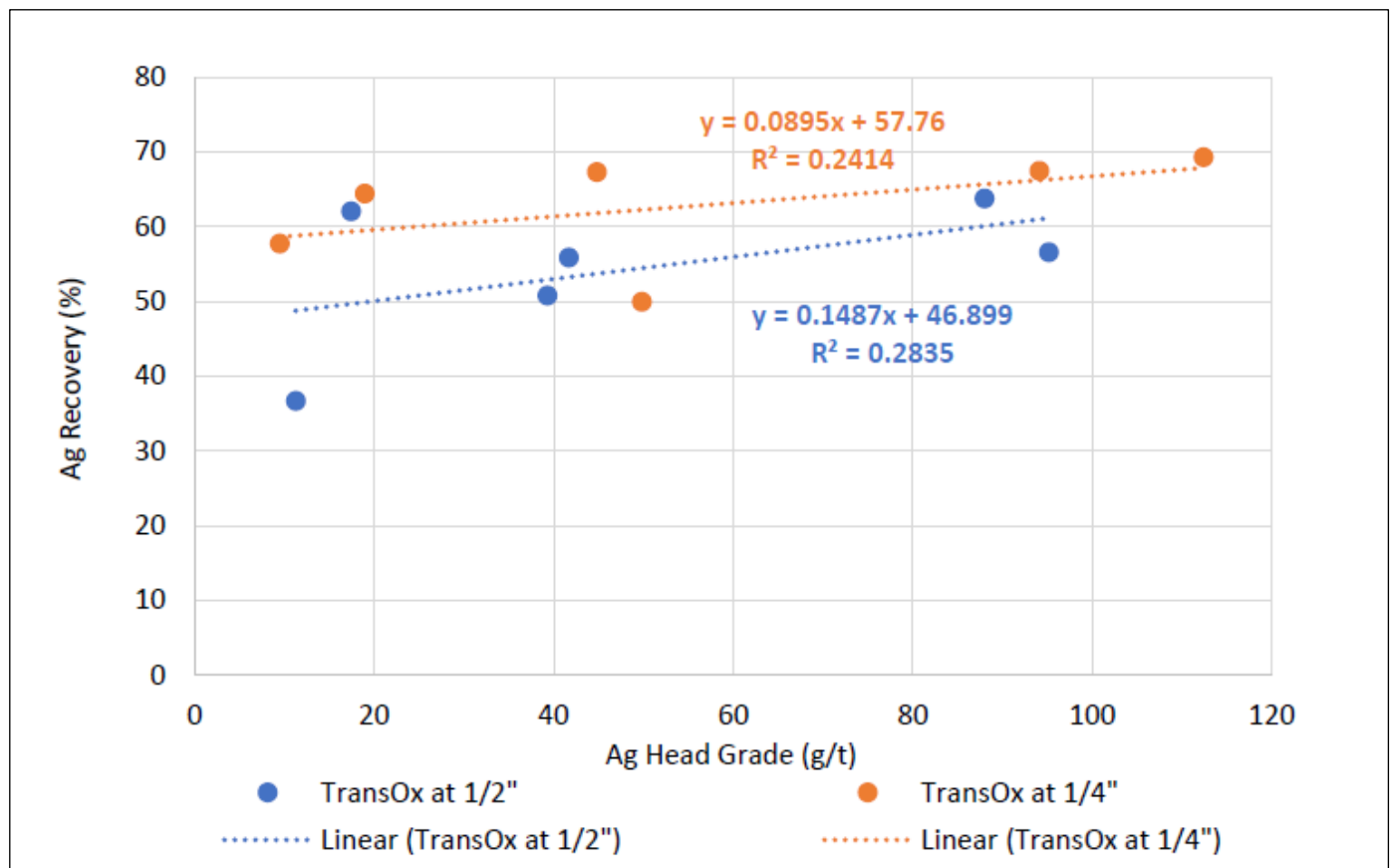
Figure 13-22: Additional Transition/Oxide Composite 96-hour, 0.5-inch Leach Test Results
