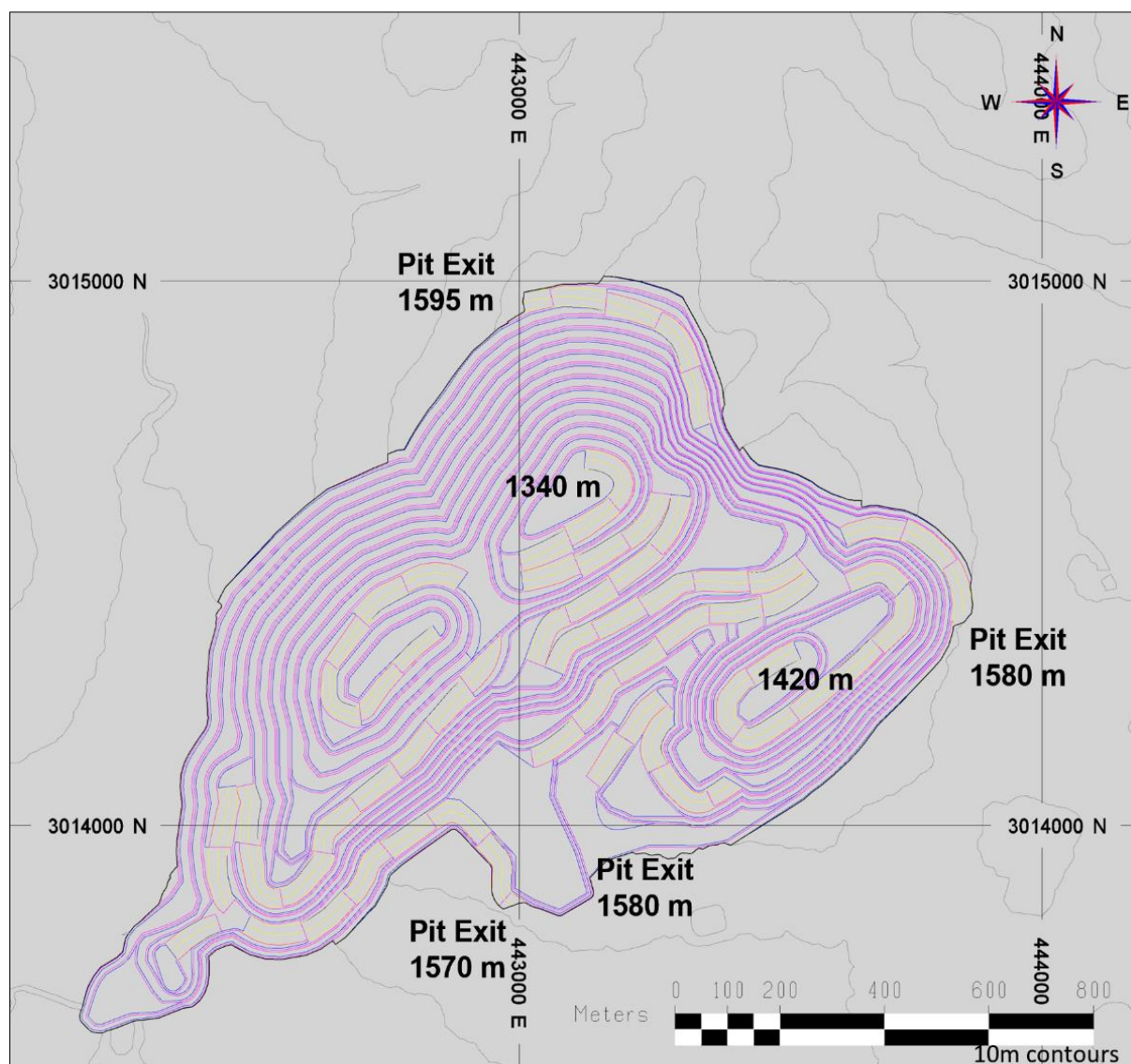
Figure 16-5: Phase 3 Layout
