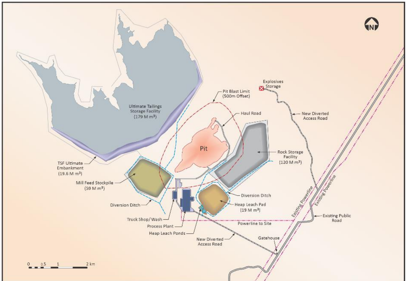
Figure 1-4: Overall Site Layout
