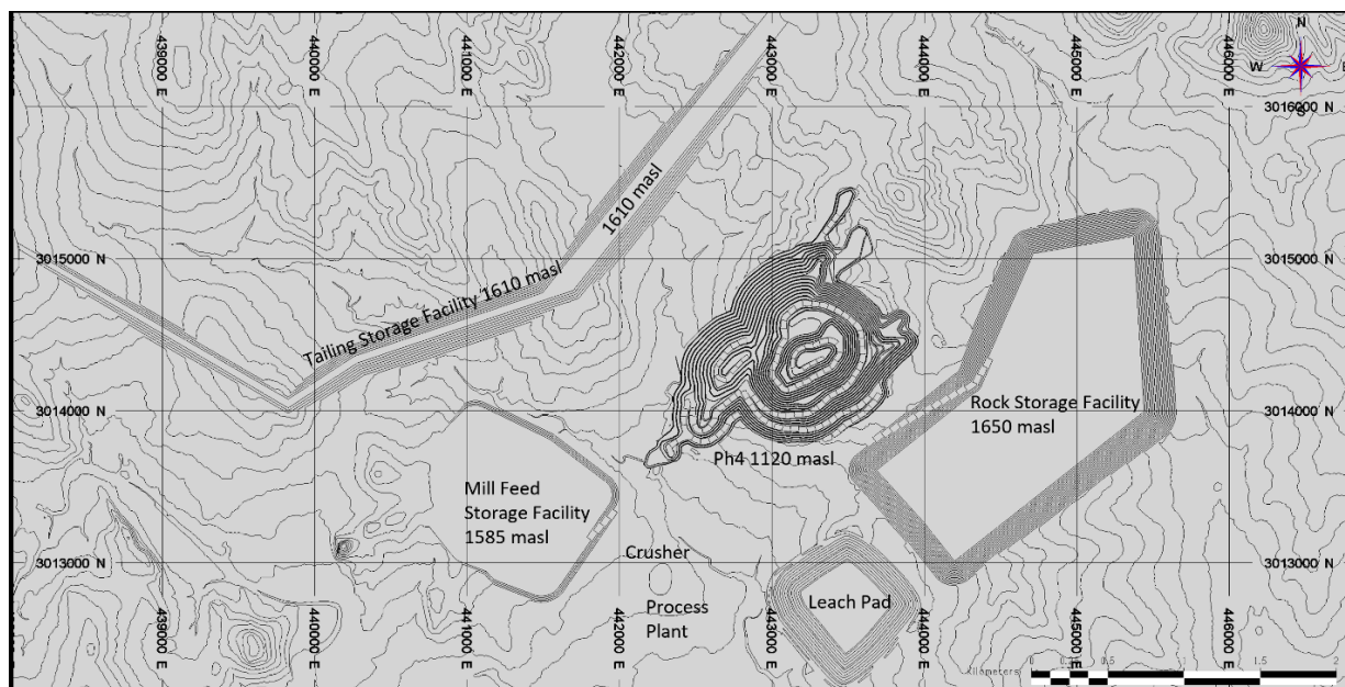
Figure 16-16: End of Year 13 (Mining Complete)
