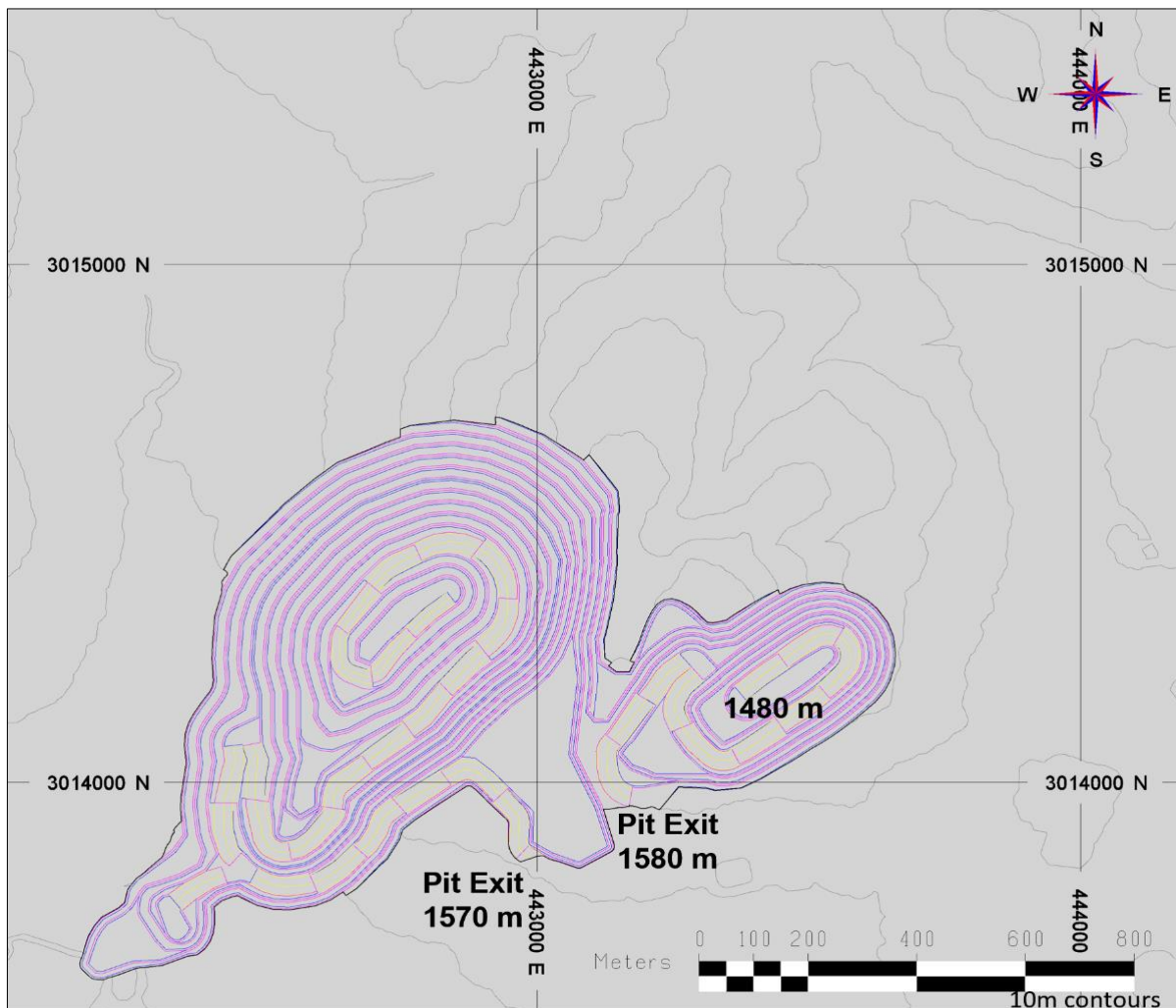
Figure 16-4: Phase 2 Layout
