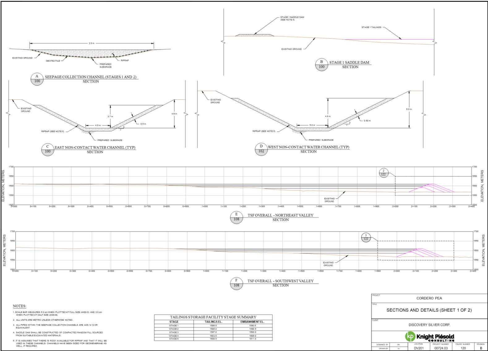
Figure 18-8: Tailings Storage Facility Sections and Details
