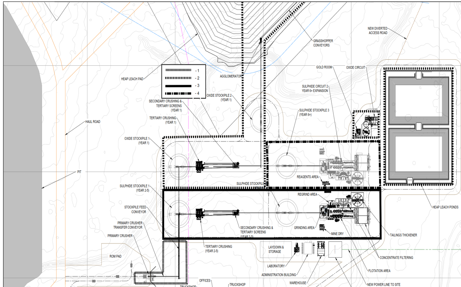
Figure 17-2: Overall Process Plant Layout
