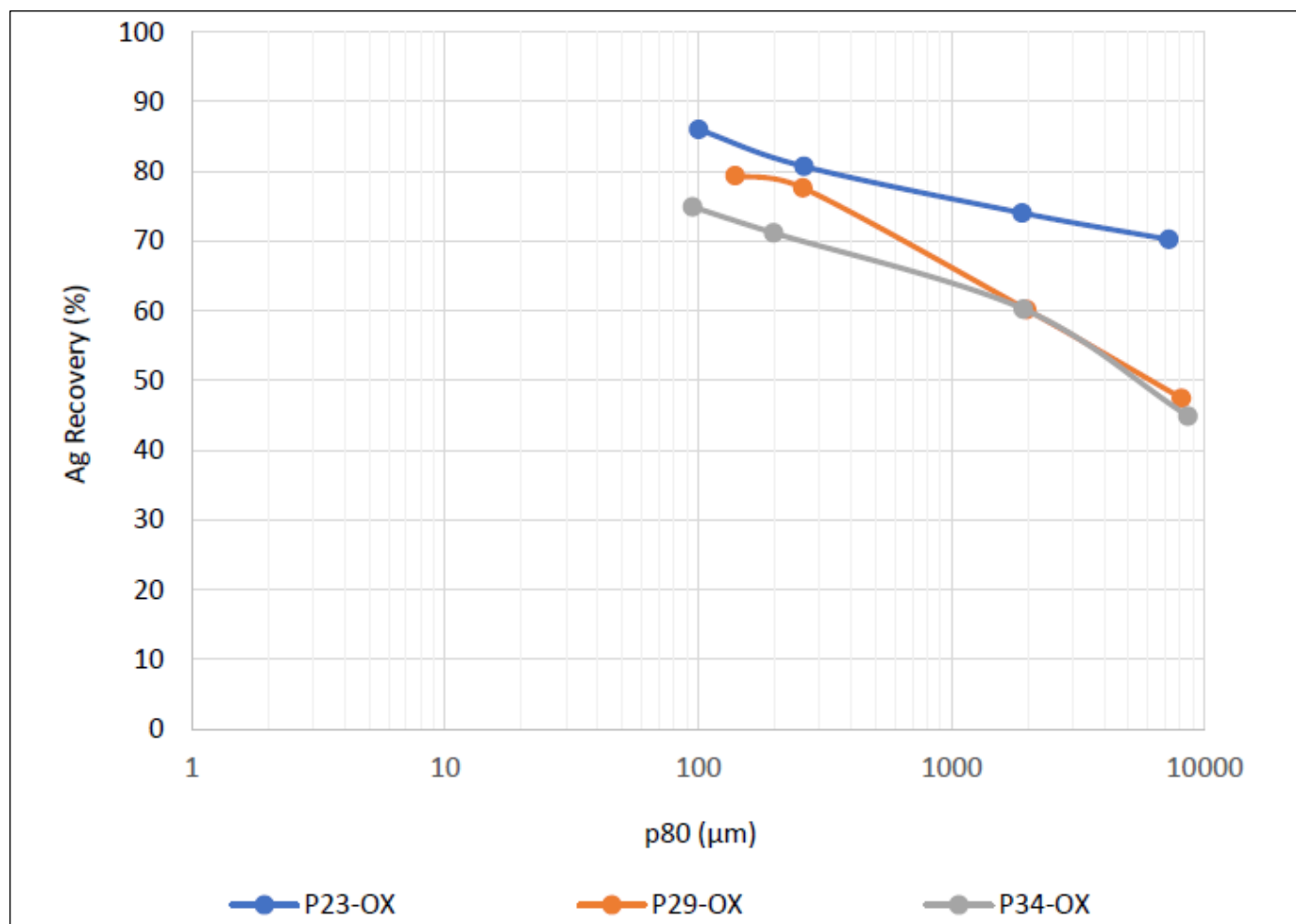
Figure 13-20: Lithology/Pit Composites Leach Response at Various Crush/Grind Sizes
