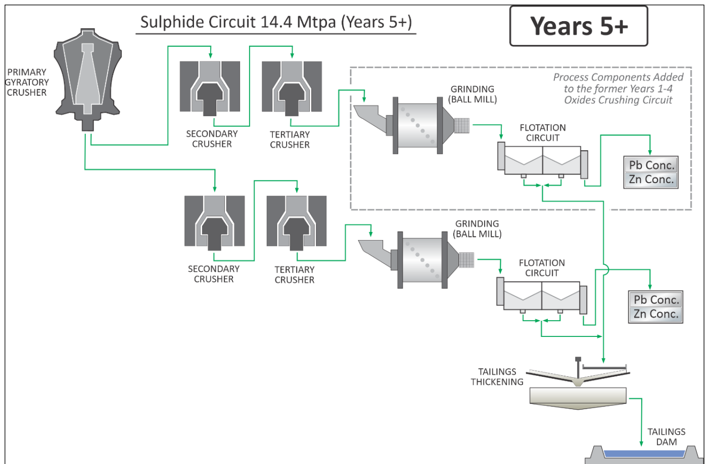
Figure 1-3: Overall Block Flow Diagram
