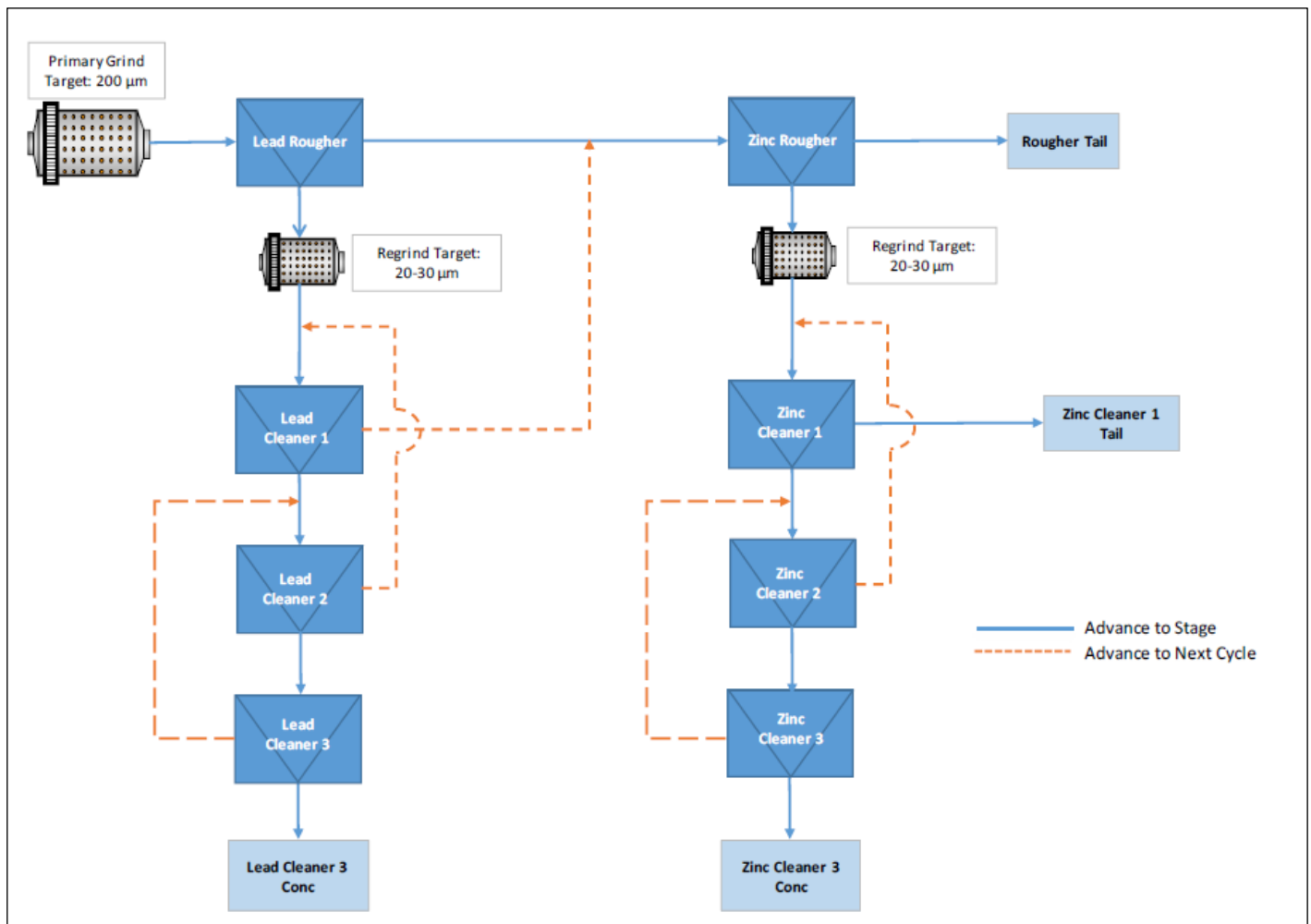
Figure 13-18: VOLC MC and Breccia-Volcanics LCT Flowsheet Configuration (No Carbon Pre-float)
