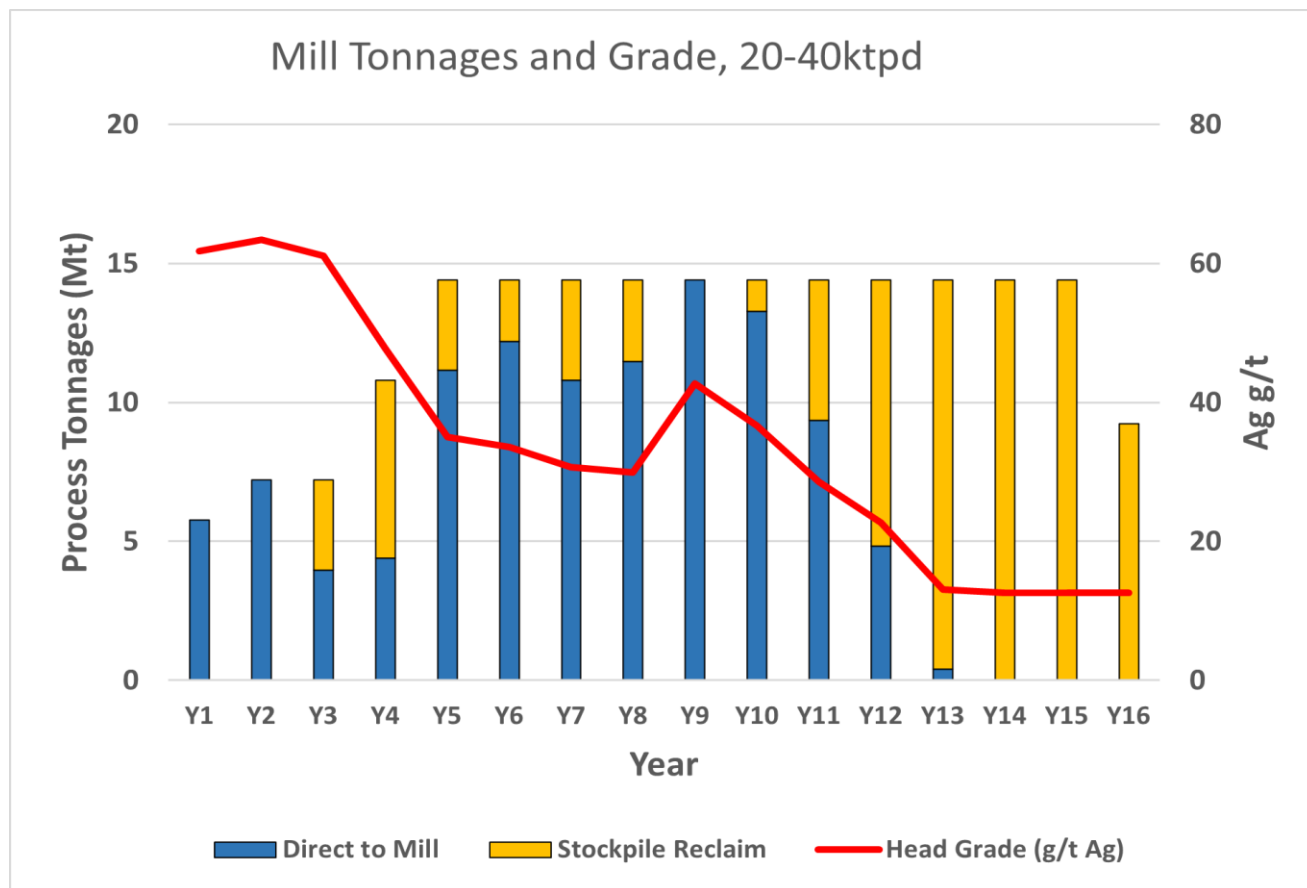
Figure 16-8: Mill Tonnes and Silver Grade
