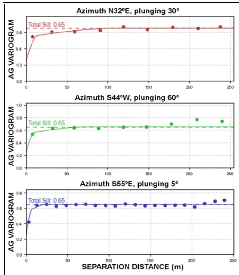
Figure 14-8: Example of Variogram Modelling
