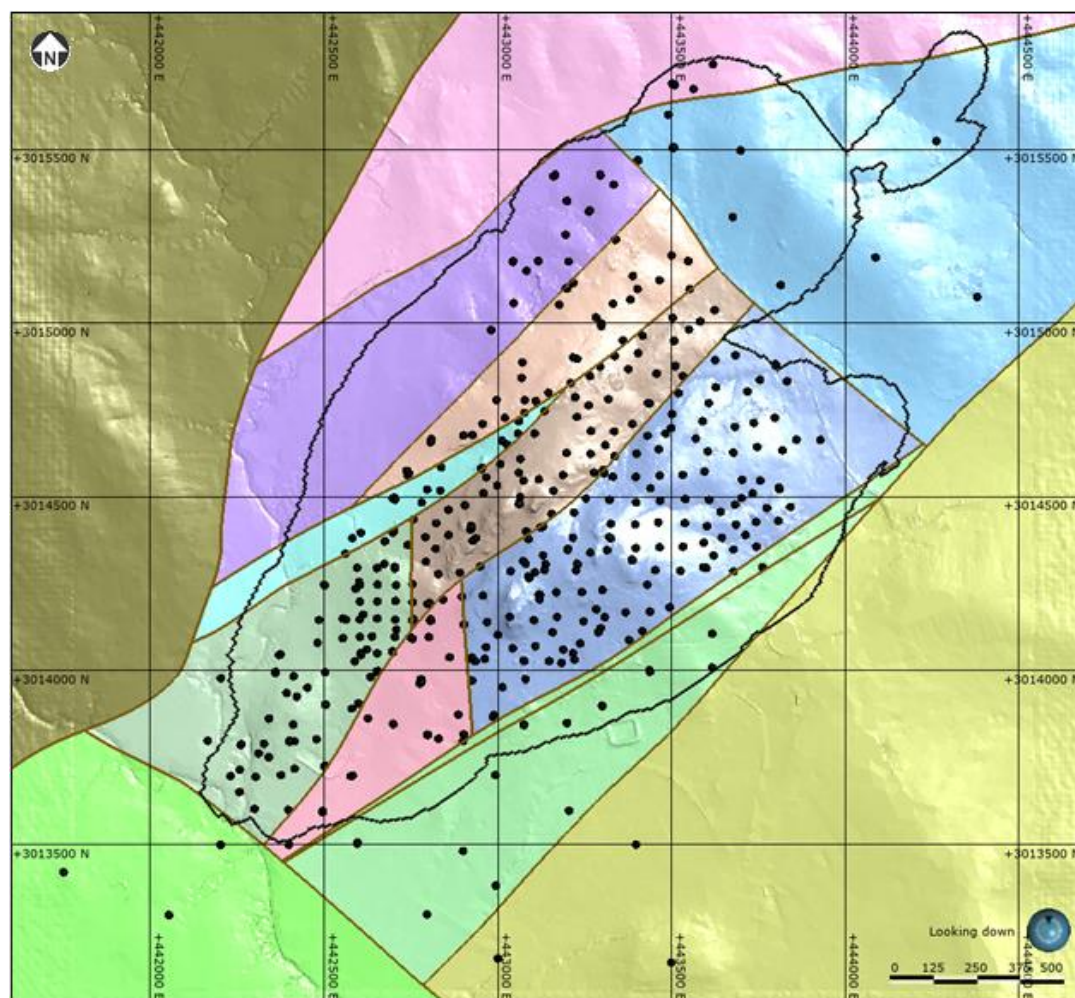
Figure 14-2: Fault Blocks in the Cordero Main Area Where Resources were Estimated
