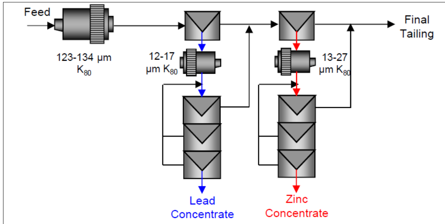
Figure 13-1: Locked Cycle Test Flowsheet Configuration
