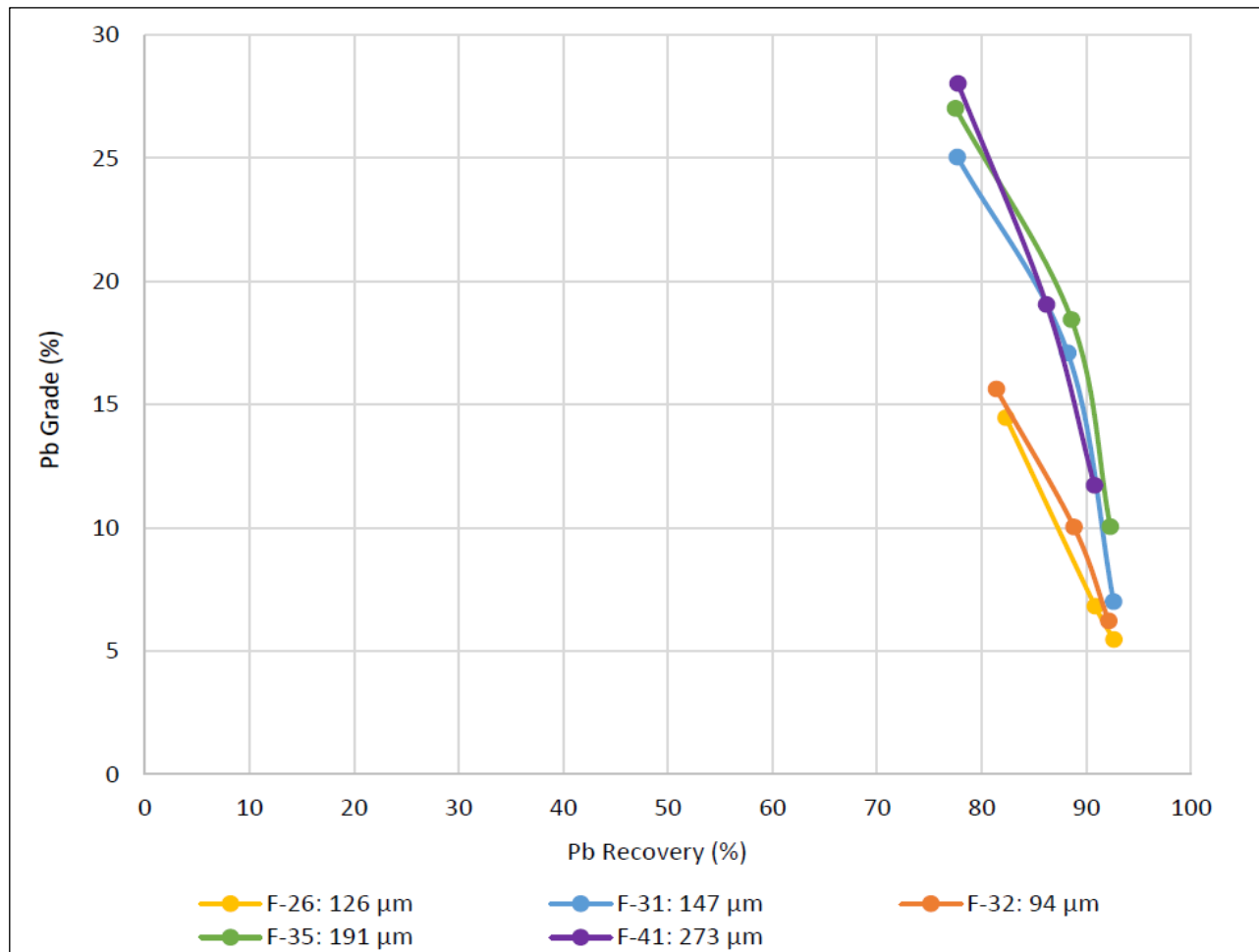
Figure 13-11: VOLC Master Composite Primary Grind vs. Recovery Sensitivity (Lead Grade Recovery Curves)
