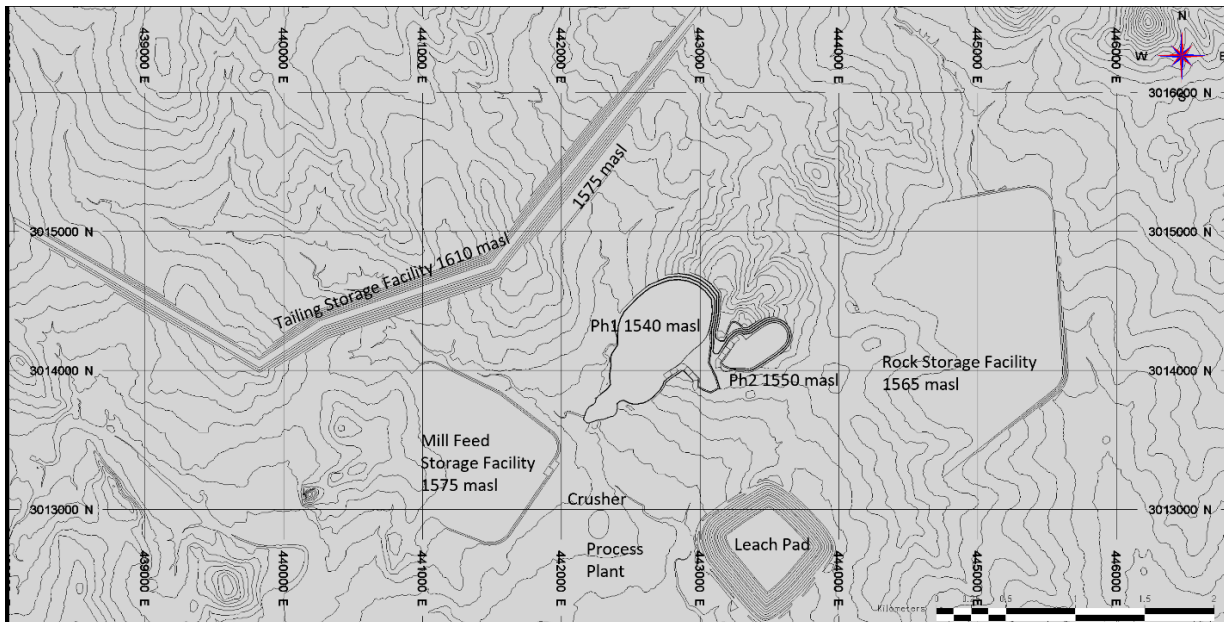
Figure 16-10: End of Year -1
