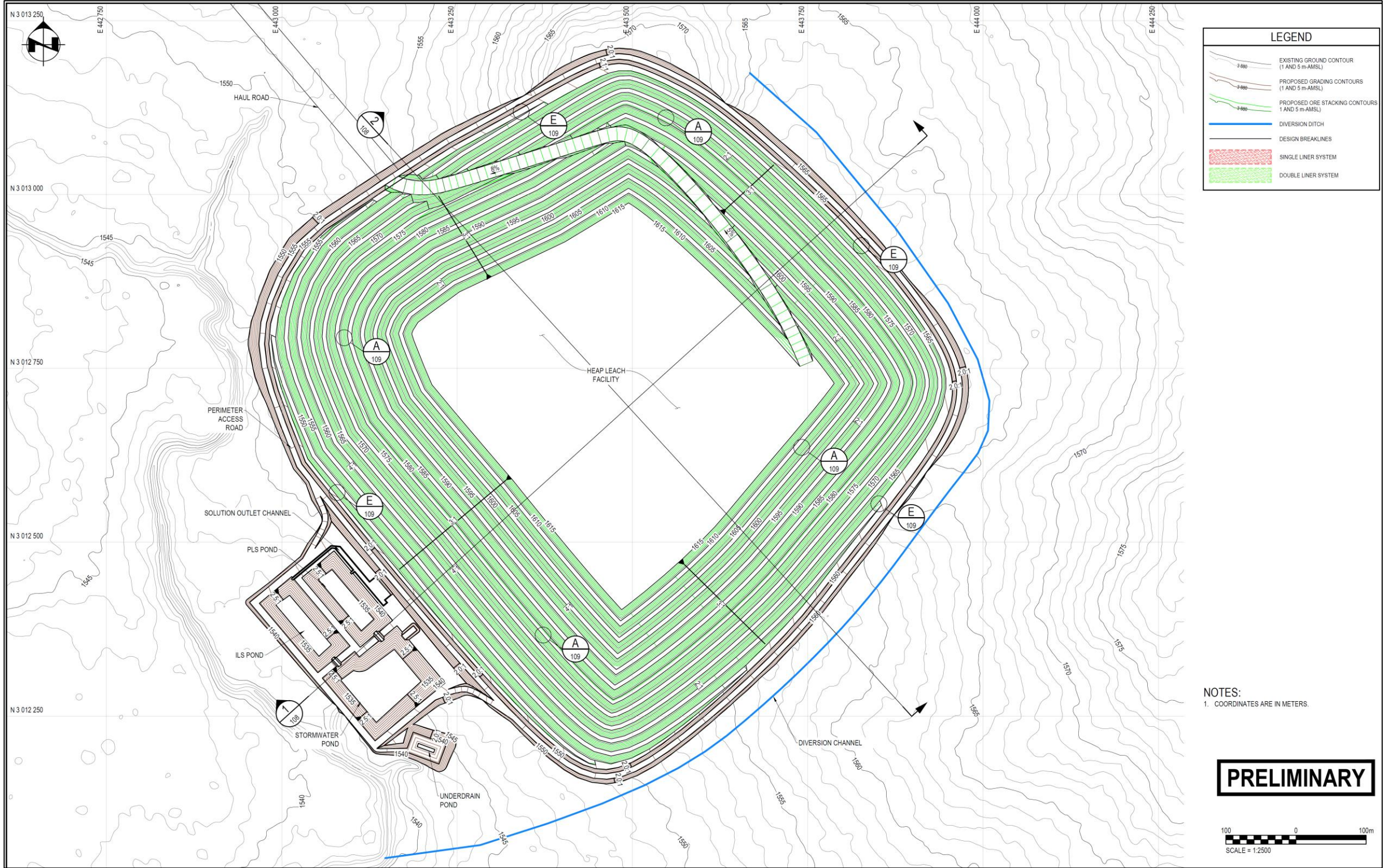
Figure 18-4: Heap Leach Facility
