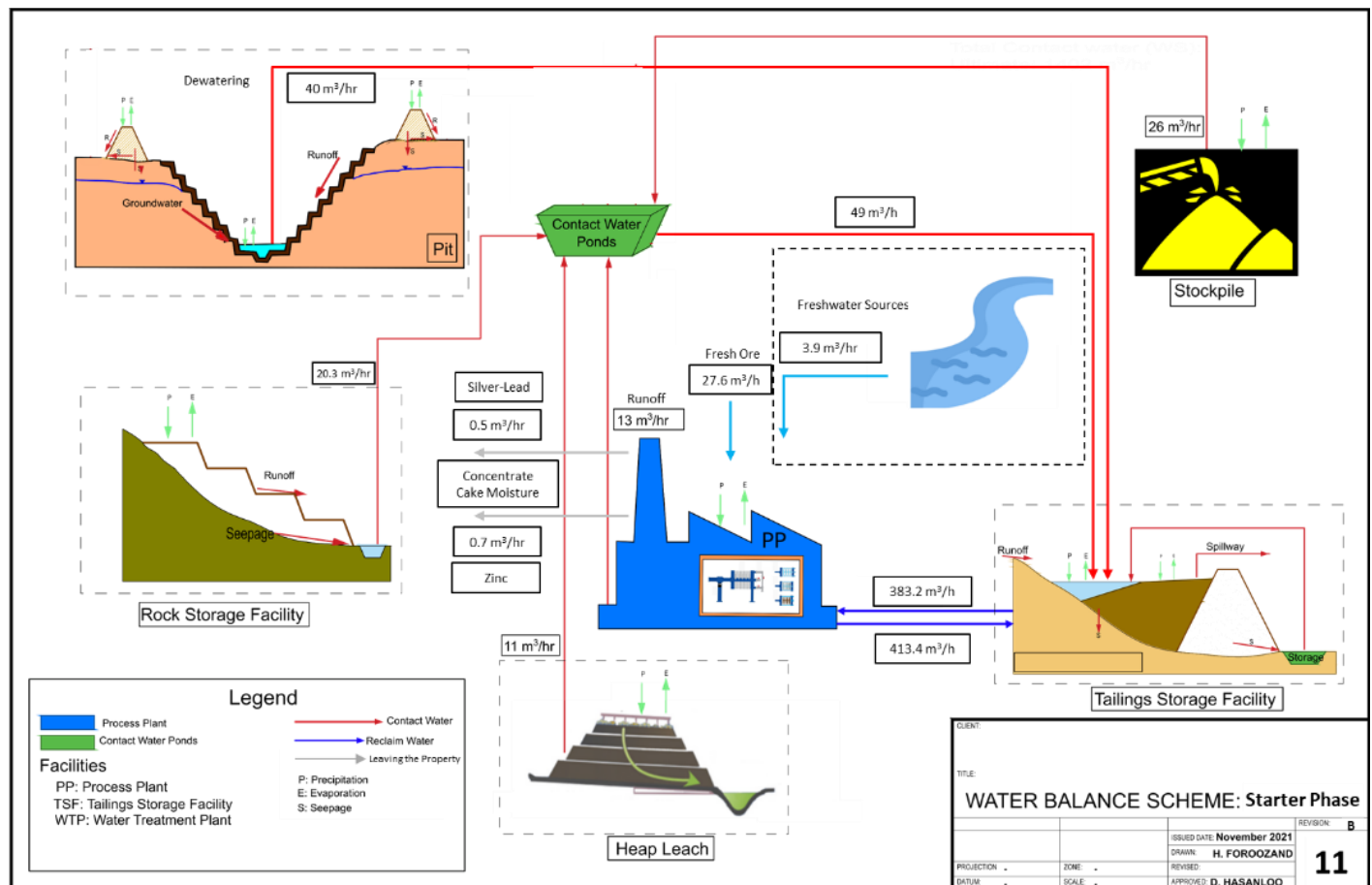
Figure 18-14: Schematic of Starter Phase Site-Wide Water Balance
