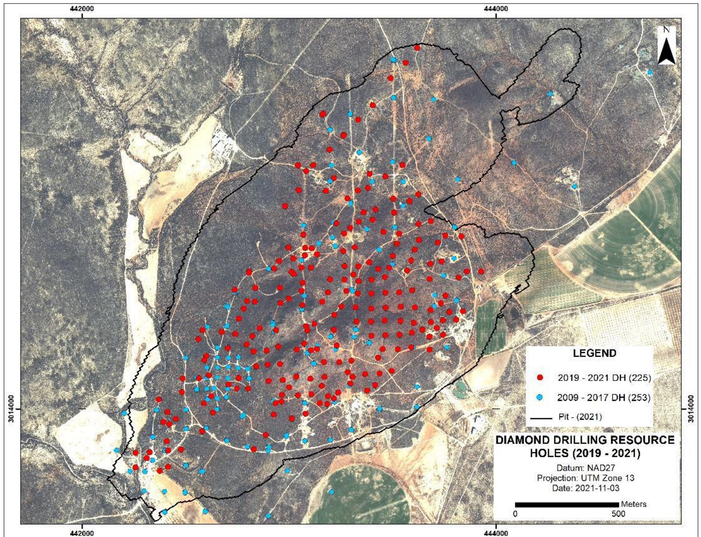
Figure 10-4: 225 Holes in the Resource Modelling Area that were used for the Mineral Resource Estimate
