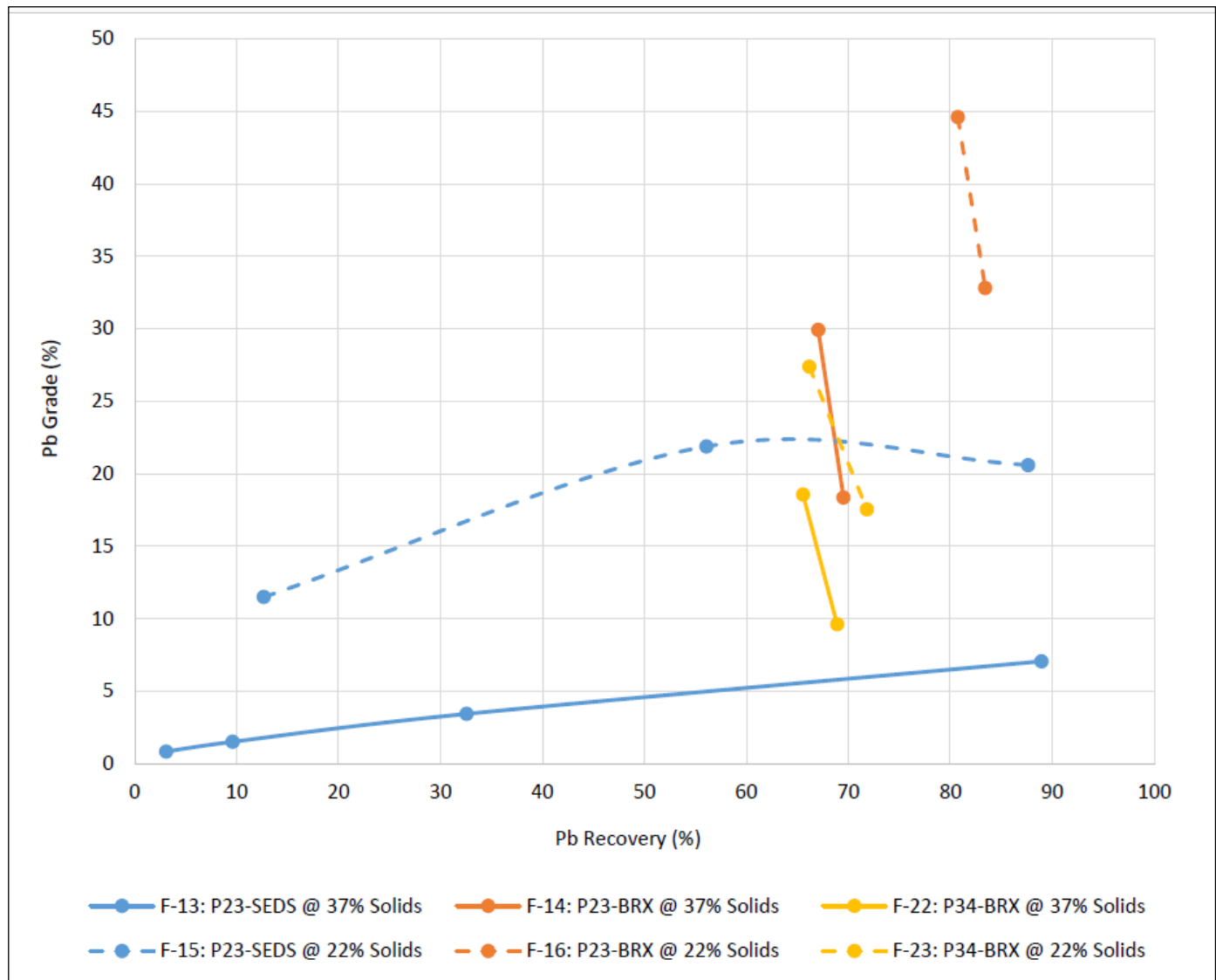
Figure 13-10: Pulp Density Sensitivity Tests Lead Grade vs. Recovery Curves (with Carbon Pre-float)
