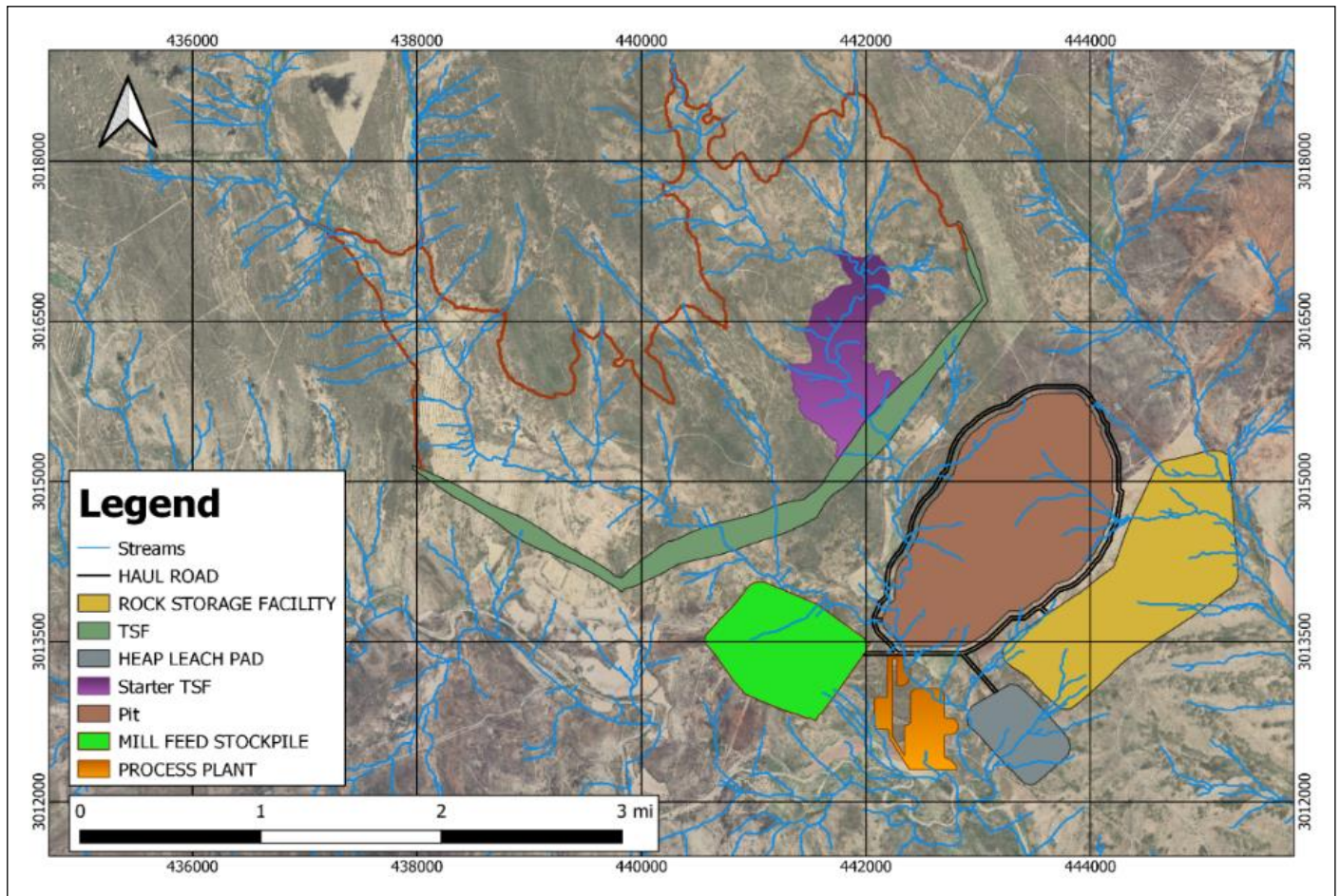
Figure 18-11: Cordero Site Facilities
