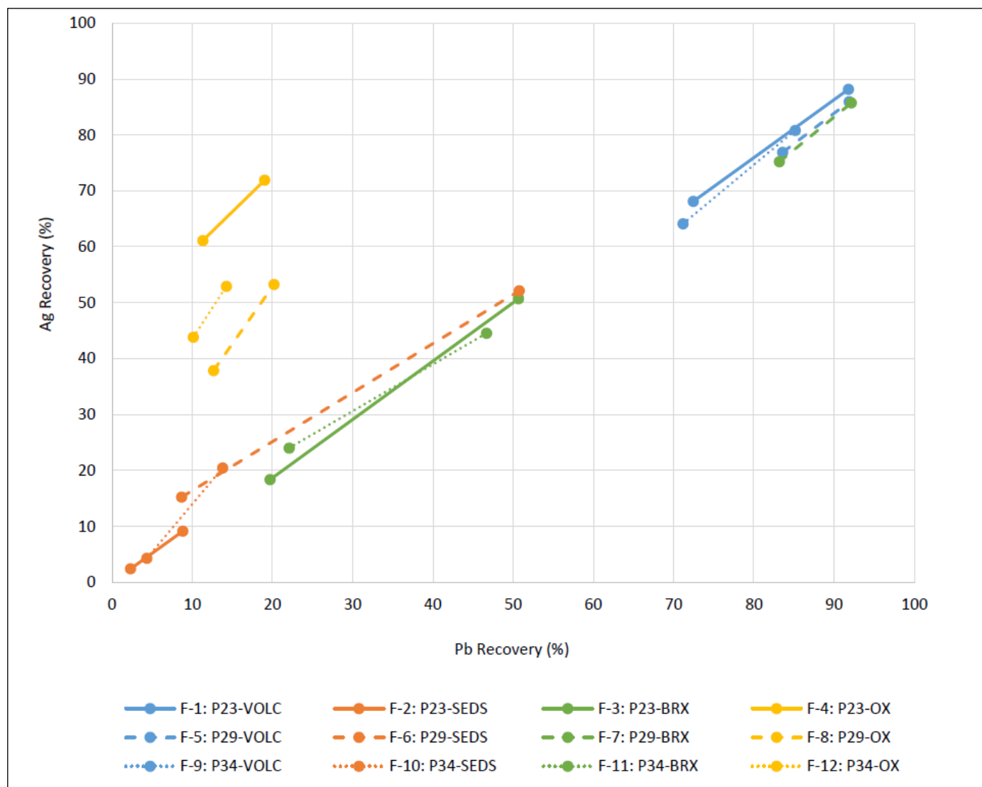
Figure 13-7: Lithology/Pit Composite Silver vs. Lead Recovery to the Lead Rougher
