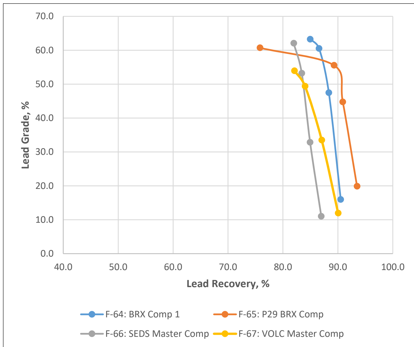
Figure 13-16: Cleaner Circuit Optimization Lead Grade vs. Recovery Curves
