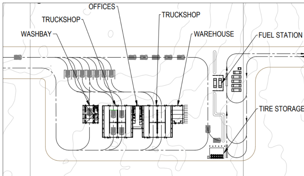
Figure 18-2: Truckshop, Washbay, Mine Warehouse, Tire Storage Area, Fuel Station, and Office
