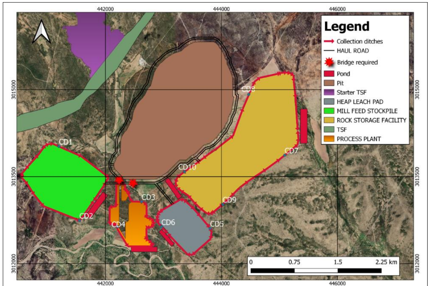
Figure 18-13: Collection Ditches
