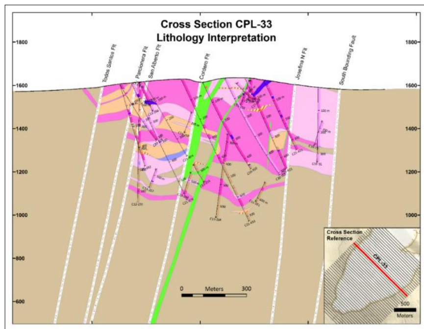
Figure 7-9: Cross-Section CPL-33
