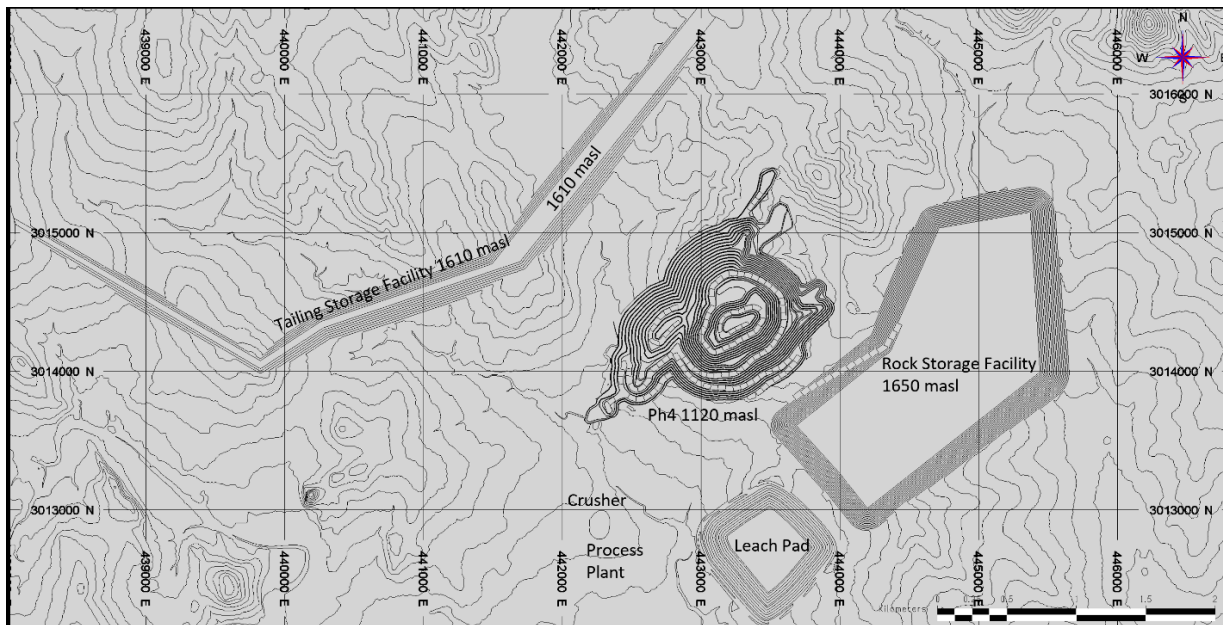
Figure 16-17: End of Year 16 (Processing Complete)
