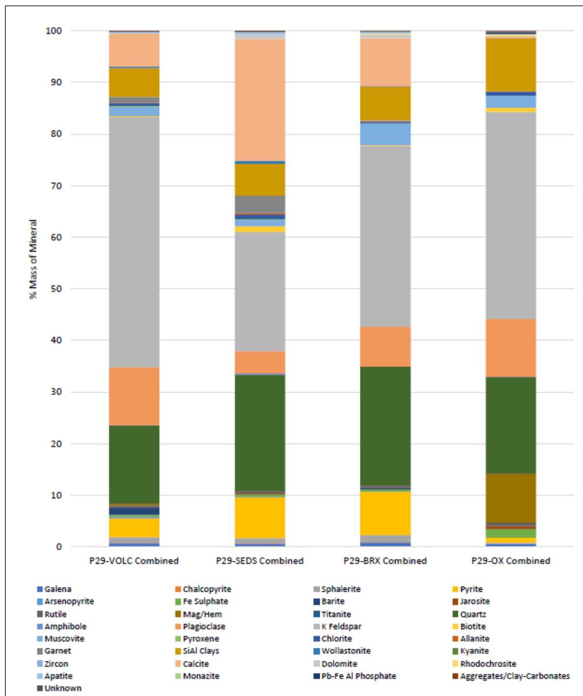
Figure 13-4: Pit 29 Lithology Composites Modal Mineralogy
