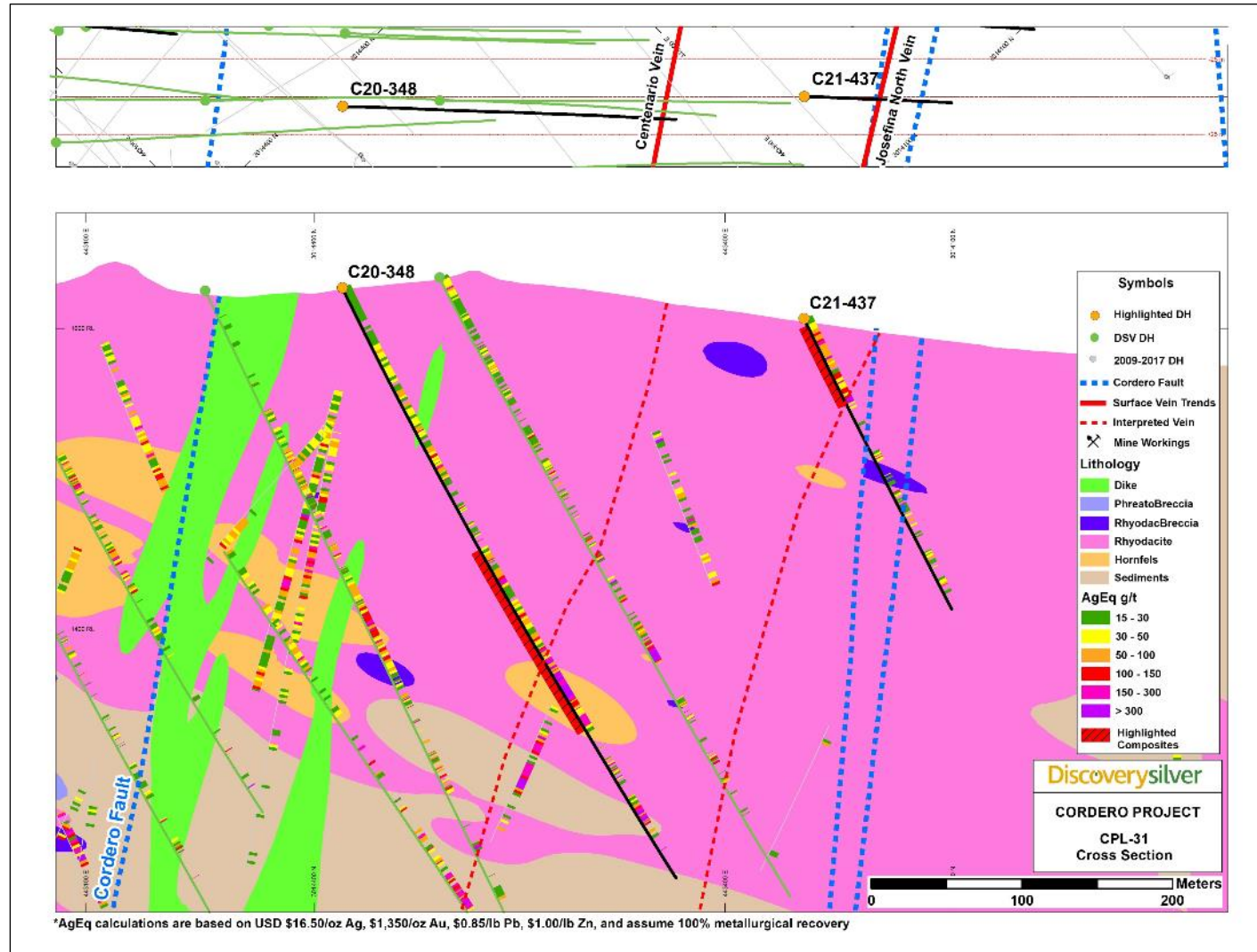
Figure 10-8: Cross-Section CPL-31 showing Geological Interpretation and Silver Equivalent Grades
