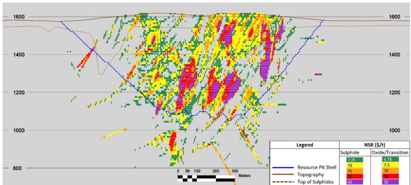
Figure 14-14: Cross-Section E-E' through the Resource Block Model
