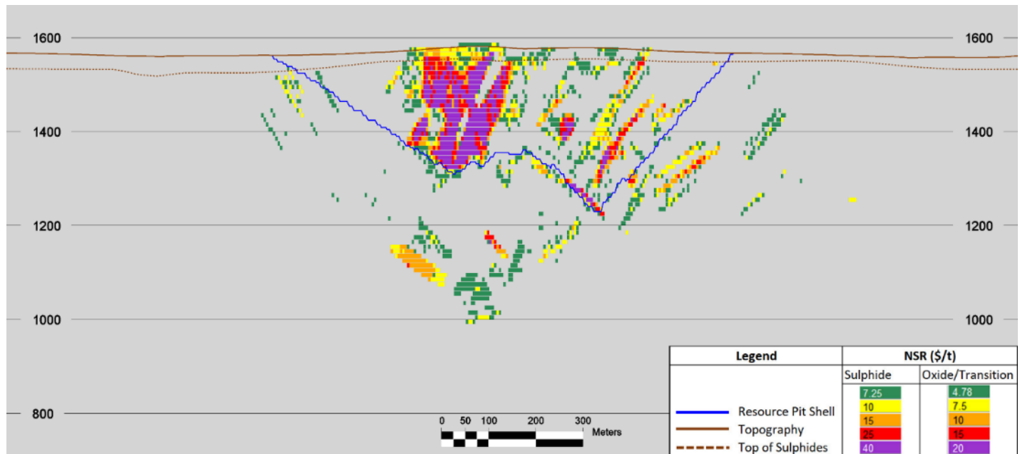
Figure 14-12: Cross-Section C-C' through the Resource Block Model
