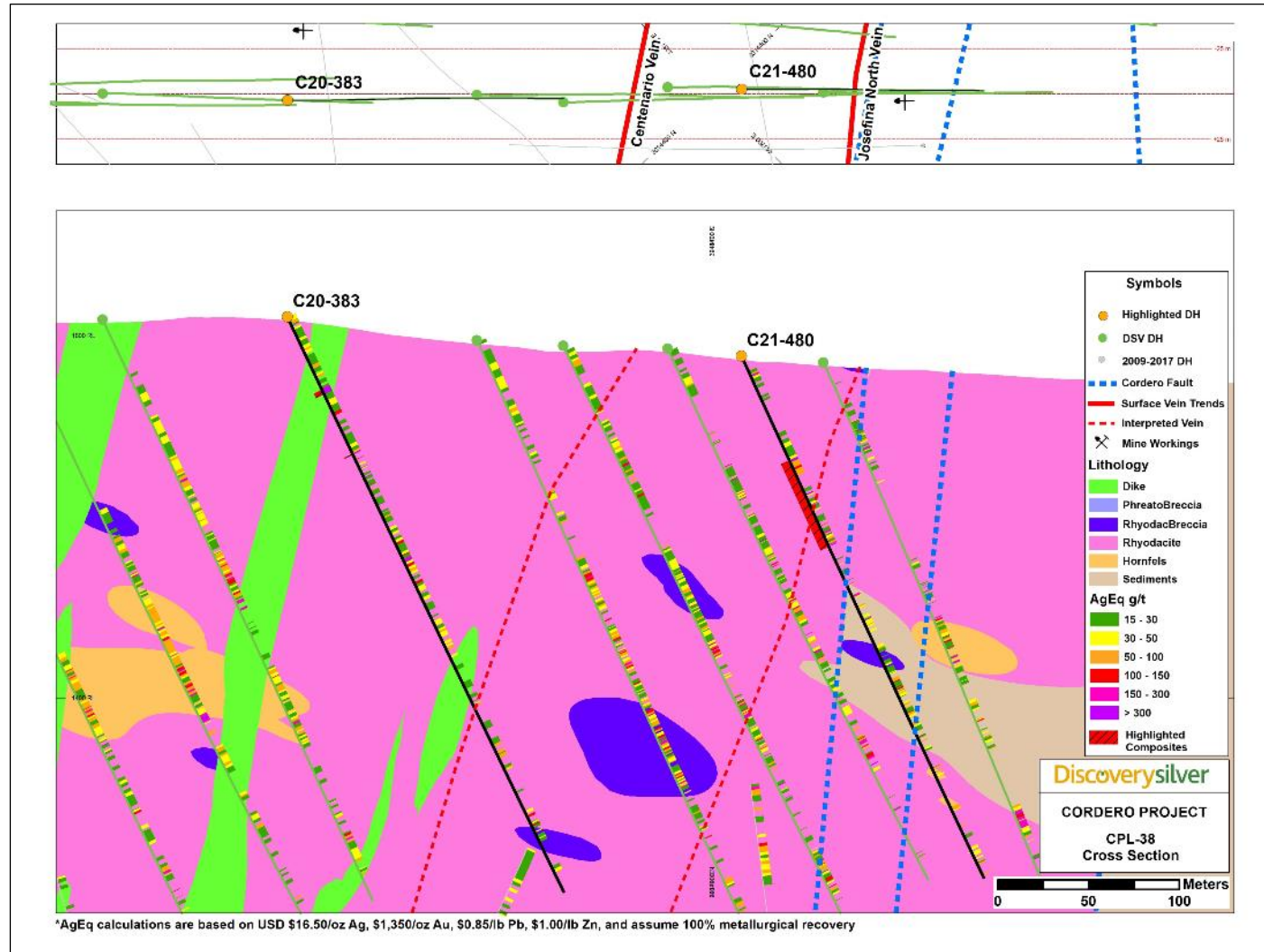
Figure 10-12: Cross-Section CPL-38 showing Geological Interpretation and Silver Equivalent Grades
