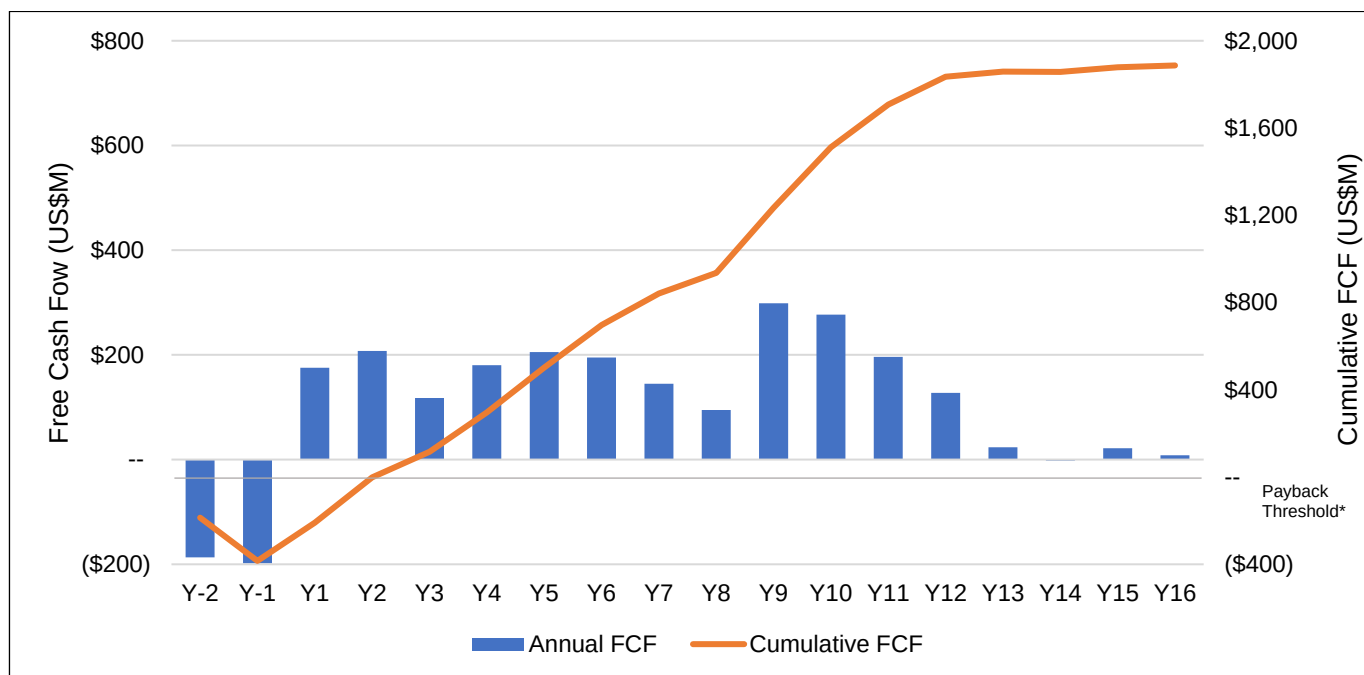
Figure 22-1: Post-Tax Project Economics
