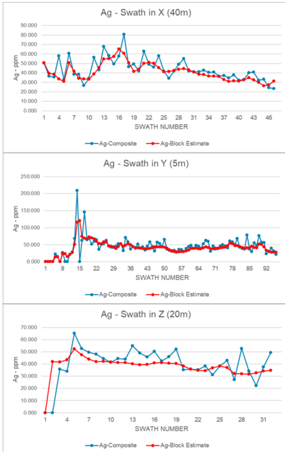
Figure 14-16: Swath Plots Comparing Silver Estimates to Drill Hole Data
