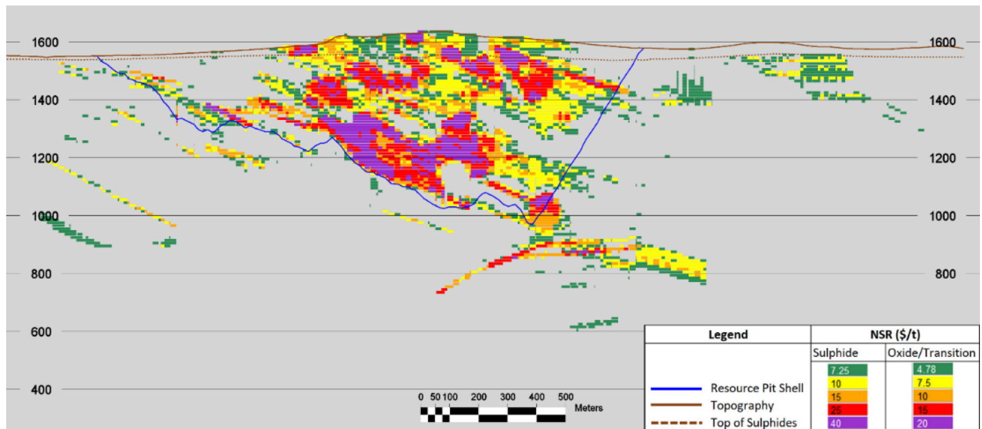
Figure 14-11: Long-Section B-B' through the Resource Block Model
