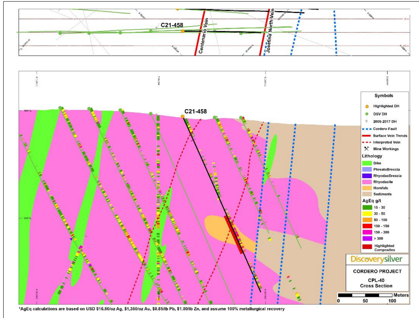
Figure 10-13: Cross-Section CPL-40 showing Geological Interpretation and Silver Equivalent Grades
