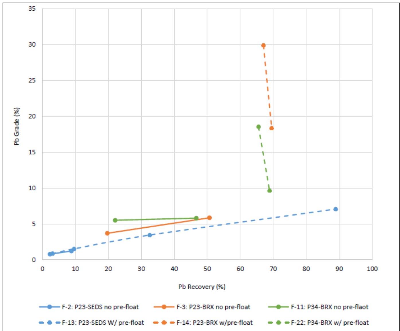
Figure 13-9: Pre-flotation Test Series Lead Recovery Versus Grade Curves
