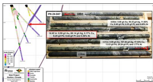
Figure 2: Core picture of hole PN-24-047 showing the strongly mineralized intervals and its location on a vertical cross-section view looking ENE along holes PN-24-047 and PN-24-051. (CNW Group/Power Nickel Inc.)
