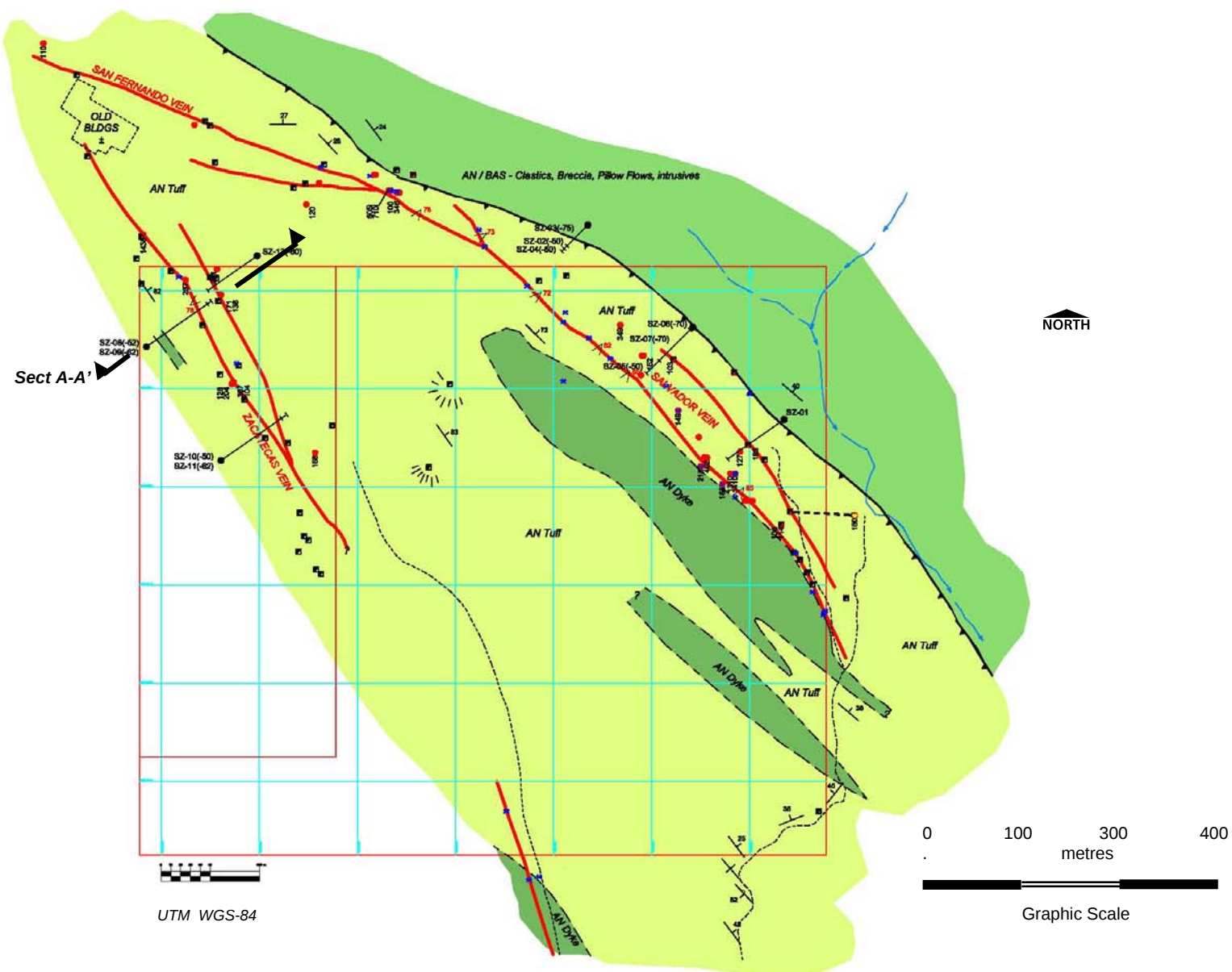
Figure 5 Property Geology – Salvador - Zacatecas
