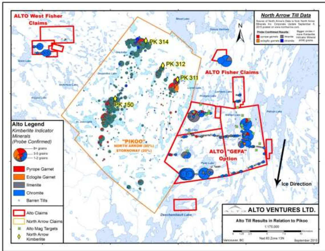
Figure 1 Alto Ventures claims are outlined in red with KIM trains and aeromagnetic anomalies shown from Alto's 2014 and 2015 programs. North Arrow Minerals claims are outlined in orange with diamondiferous kimberlites discovered to date by drilling highlighted in yellow. Note PK346 was discovered in 2016 and is located near PK314.
