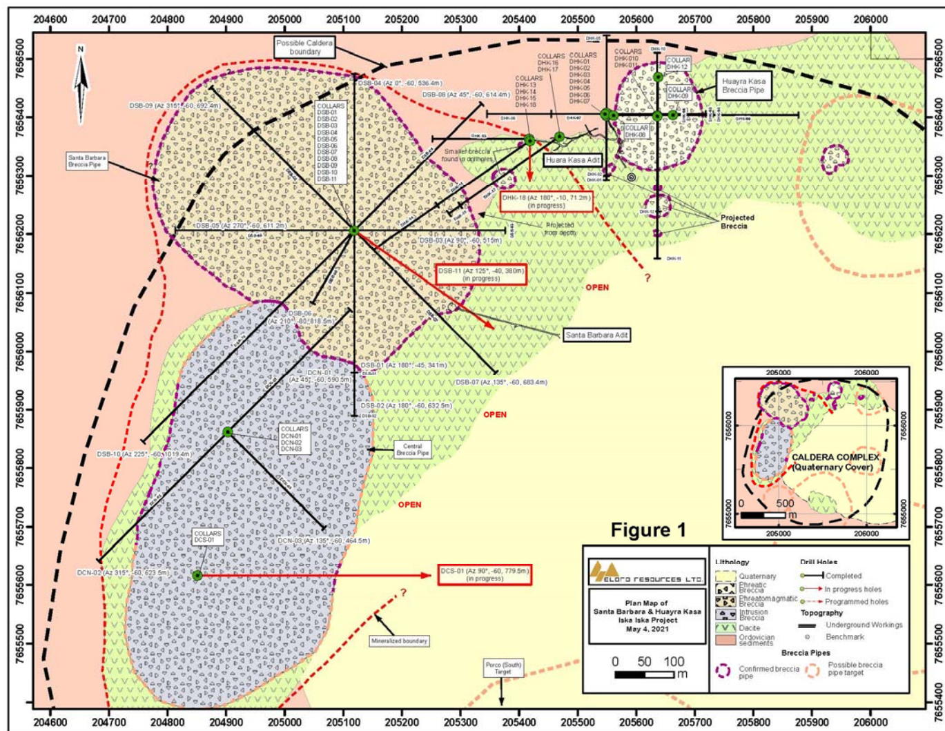
Figure 1: Geological Plan Map of the Santa Barbara and Central Breccia Pipe areas
