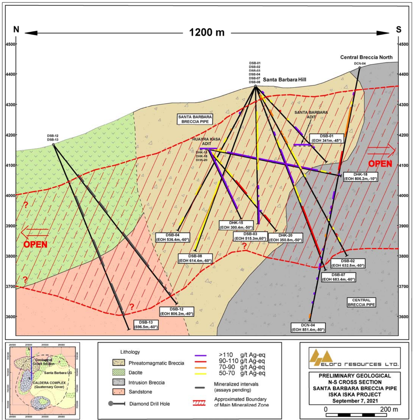
Figure 2: North-South Geological Cross Section, Santa Barbara Breccia Pipe showing Major Extension in Holes DSB-12 and DSB-13
