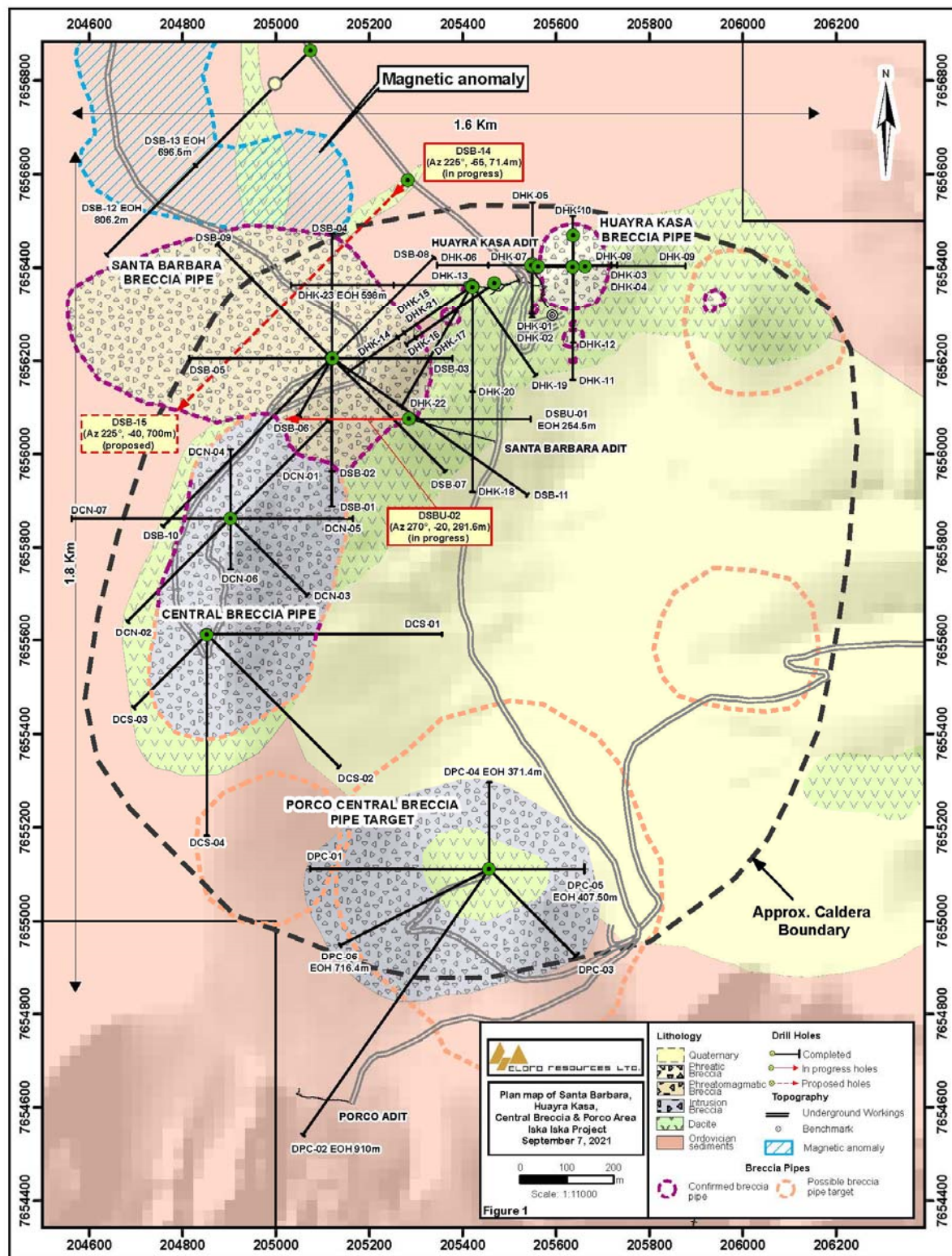
Figure 1: Geology of the Iska Iska Caldera Complex showing locations of Major Breccia Pipe targets including the magnetic anomaly northwest of the Santa Barbara Breccia Pipe and diamond drill holes completed and in progress.
