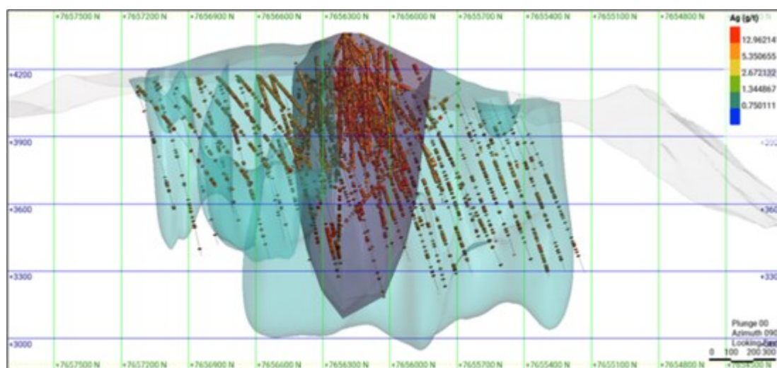
Figure 2: Iska Iska Deposit Wireframes in 3D Perspective
