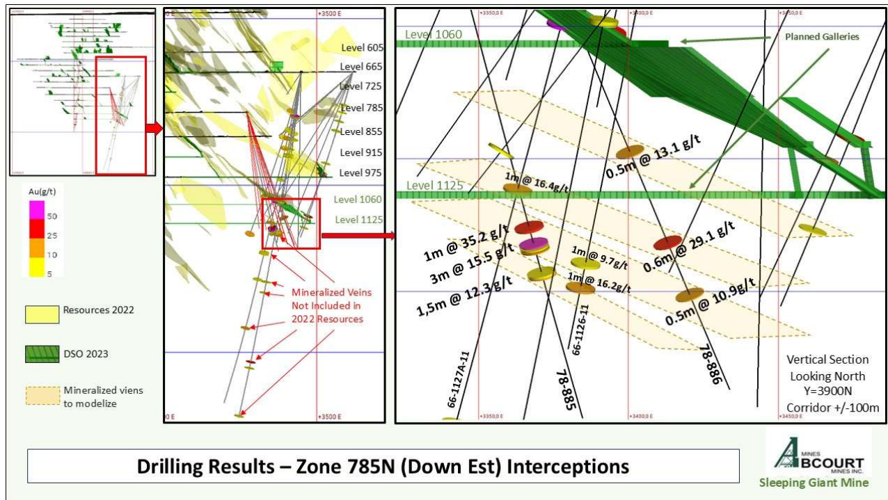
Figure 3: Main Results - Interceptions at the bottom of Zone 785N (eastern part)
