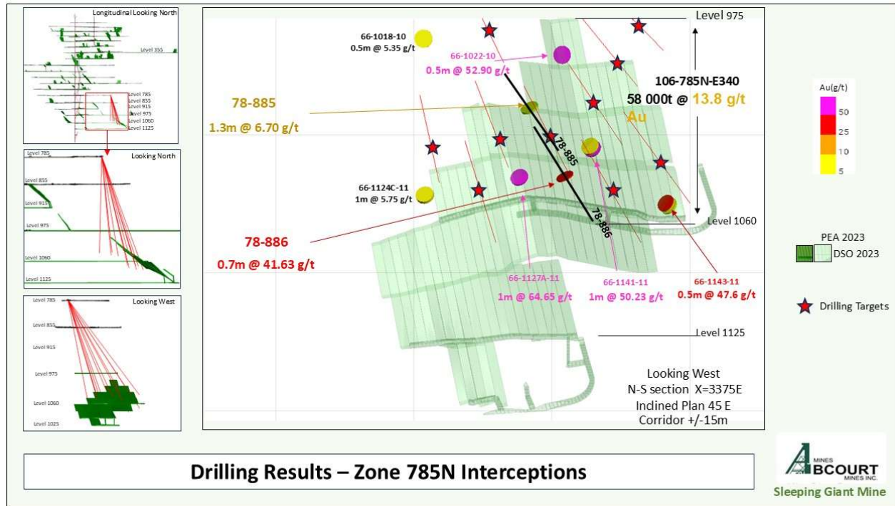
Figure 1: Main Drilling Results – Interception of 785N Zone.
