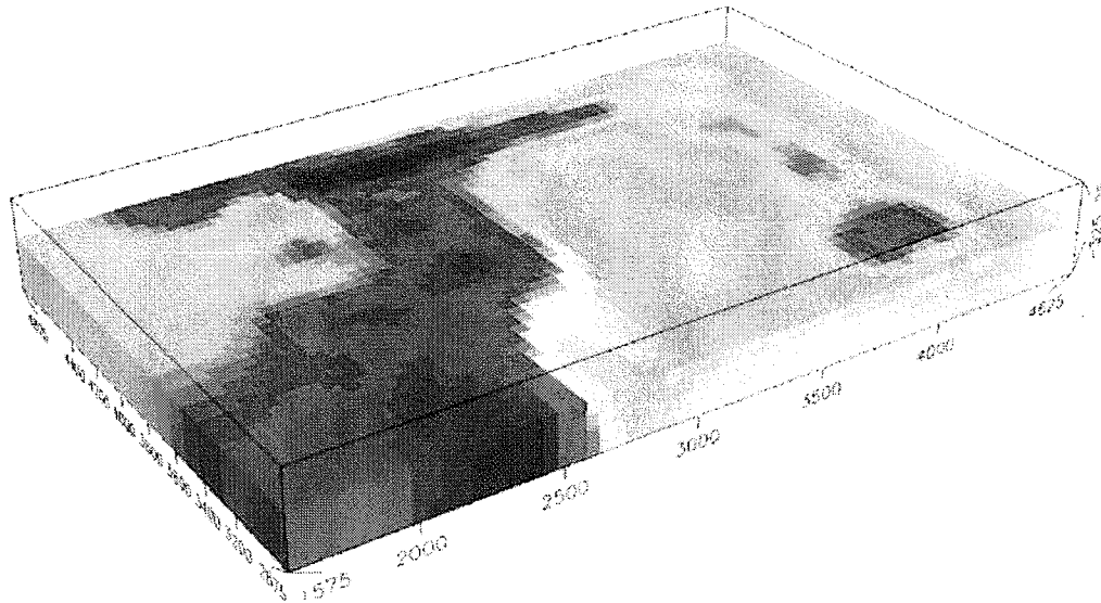
3D MODELLED RESISTIVITY DEPTH 125 Meters
