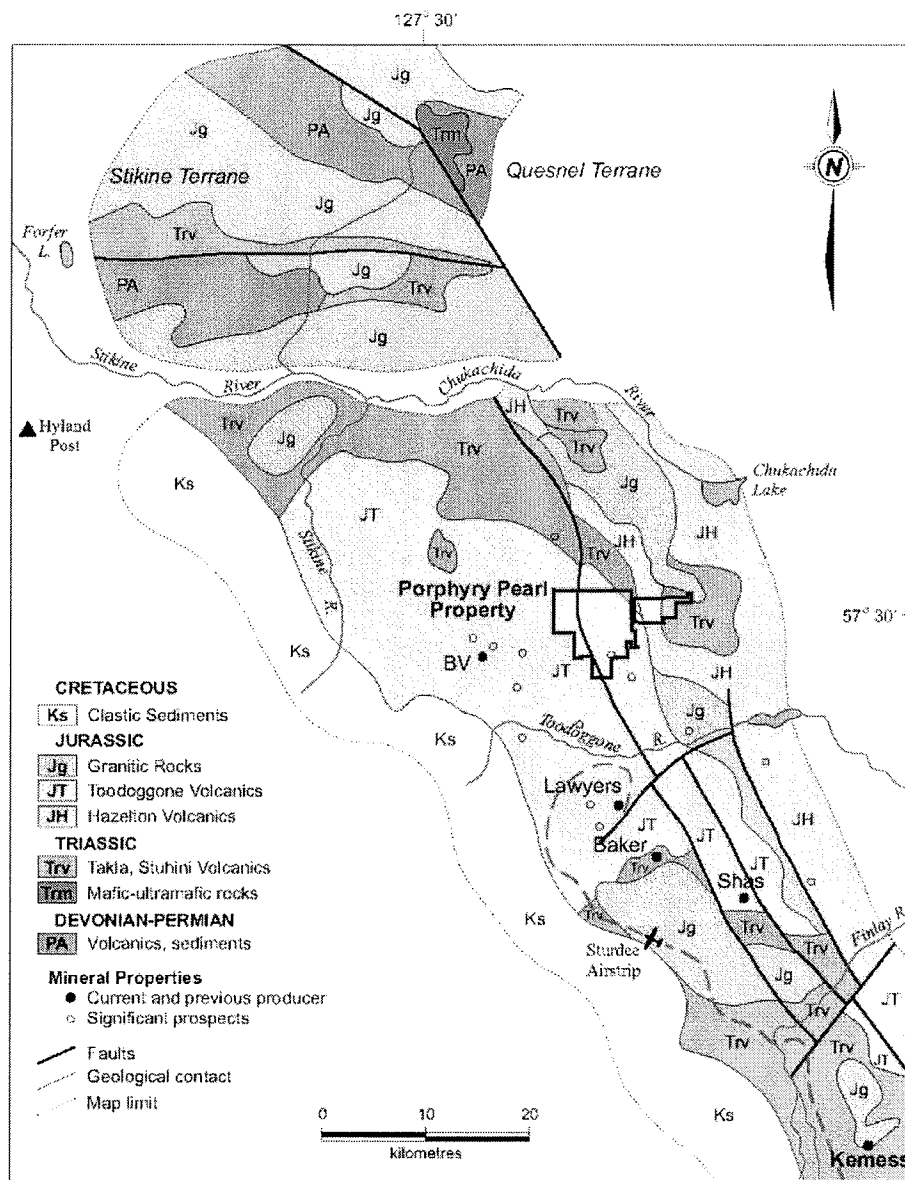
Figure 4: Porphyry Pearl Property - Regional Geological Setting
