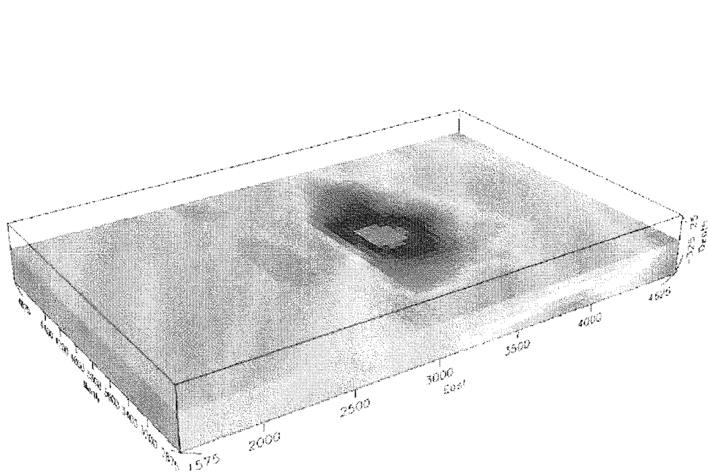
3D MODELLED CHARGEABILITY DEPTH 125 Meters
