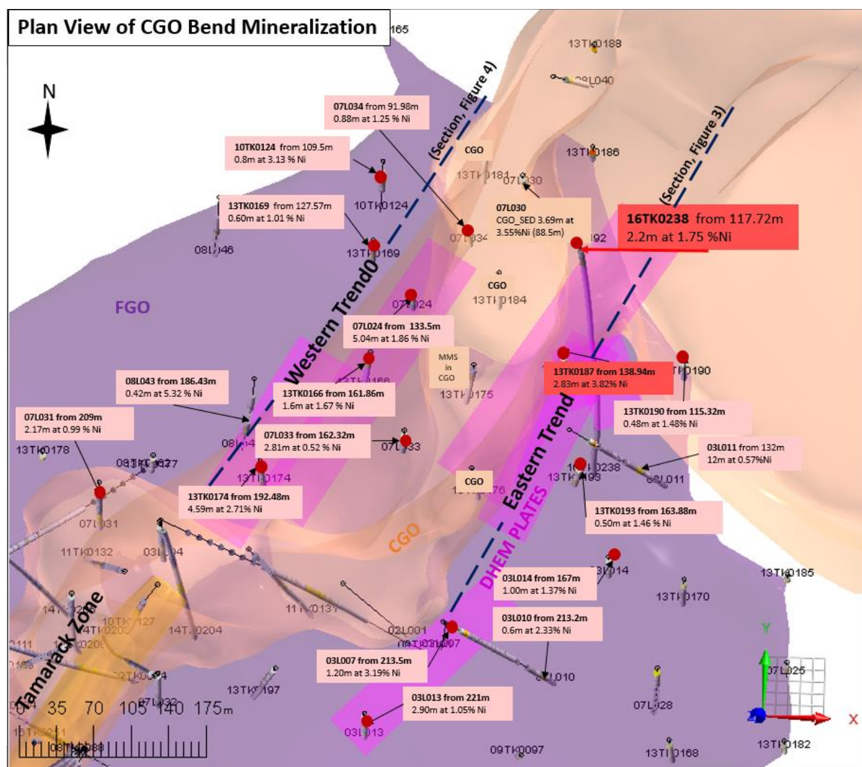
Figure 2: Plan view showing the CGO Bend up-dip of the Tamarack Zone with locality of drill hole 16TK0238 towards the north of the eastern trend of the CGO bend. Also shown are other historical drill hole intercepts and interpreted DHEM conductors which support the potential for continuity of mineralisation at the base of the FGO both to the east and west of the CGO (see sections in Figure 3 and 4 and Table 3 for table of historical intercepts).
