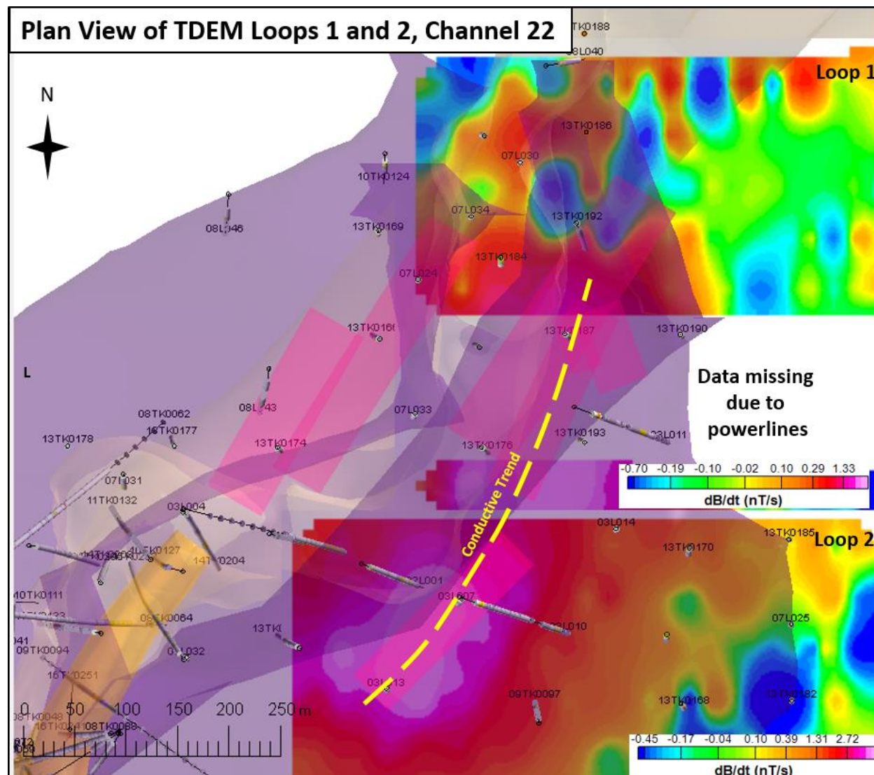
Figure 5: Plan of the CGO Bend with the recently completed TDEM survey covering the eastern trend, with conductors corresponding the interpreted DHEM conductors at the base of the FGO.
