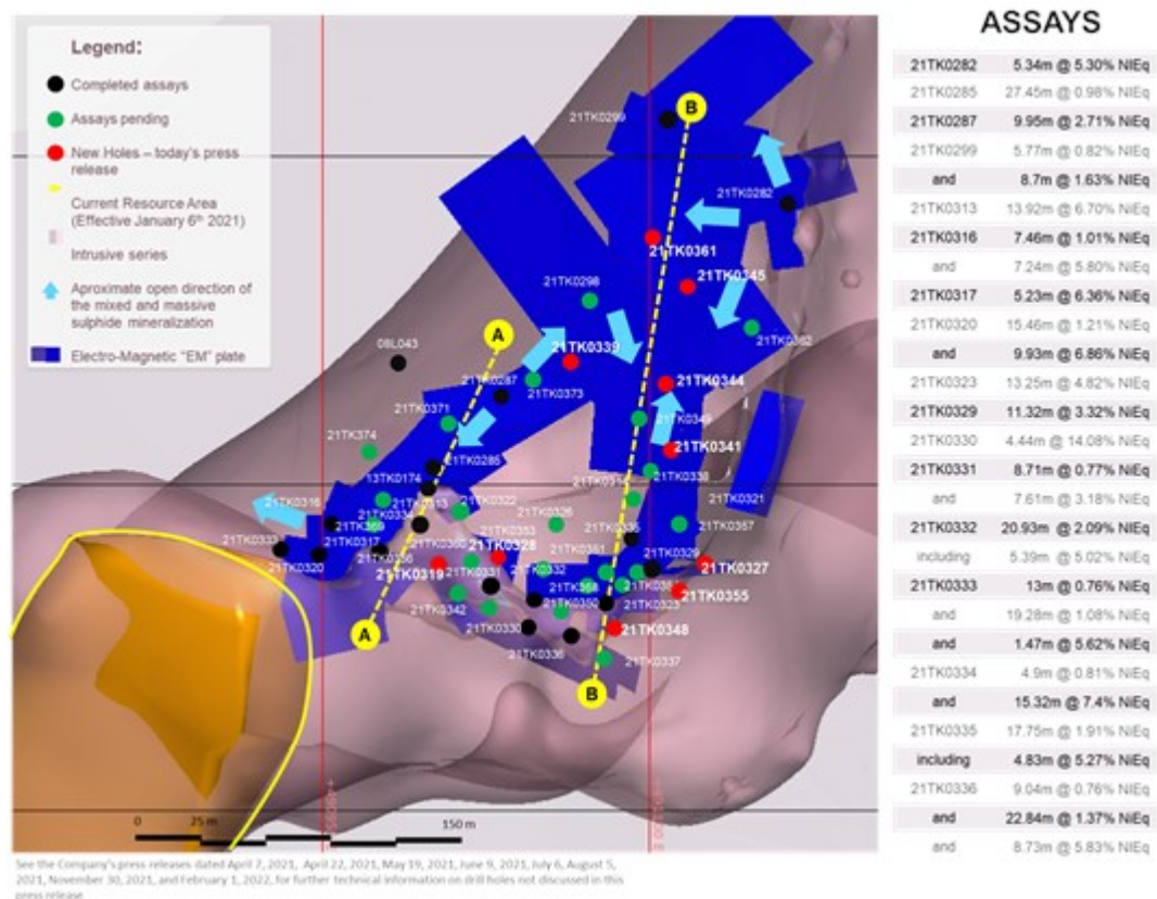
Figure 2. Plan view geological map of the northern portion of the Tamarack Nickel Project (CGO West area) showing the new drill holes in red
