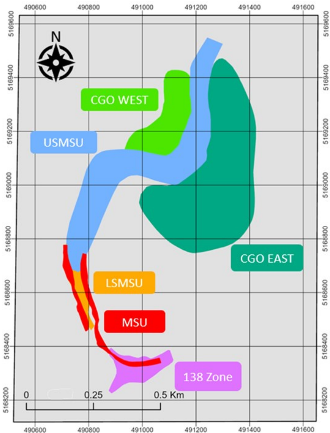
Figure 1. Plan view of the expanded mineral resource area at the Tamarack Nickel Project. Coordinate system UTM-NAD 83
