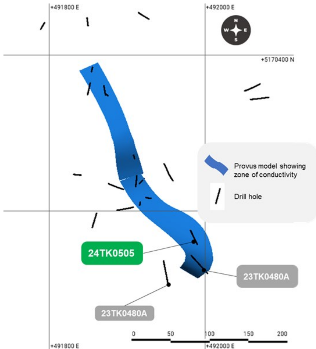
Figure 4: Talon uses various software to assist the Company to identify "conductive" zones, which leads to finding additional areas of nickel-copper mineralization. Novaminex's Provus EM modelling software is one example of software that has been successfully used by Talon, in this case to drill 24TK0505 in the Raptor Zone.
