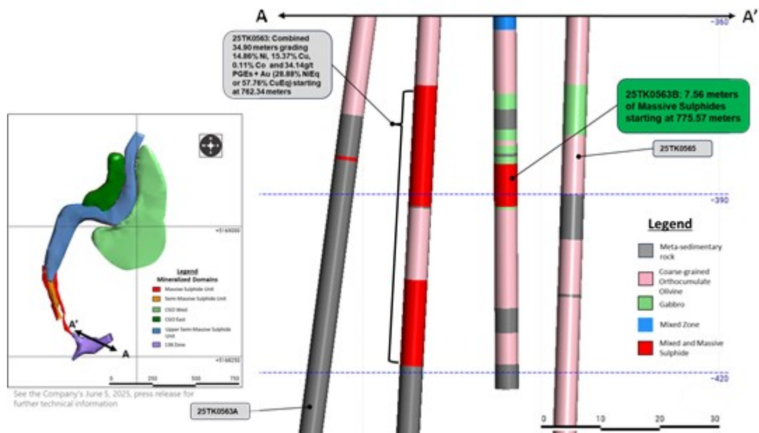
Figure 3: Cross section looking southwest of the Vault Zone showing the spatial relationship between discovery drill hole 25TK0563 and the new approximate 16m step out drill hole 25TK0563B
