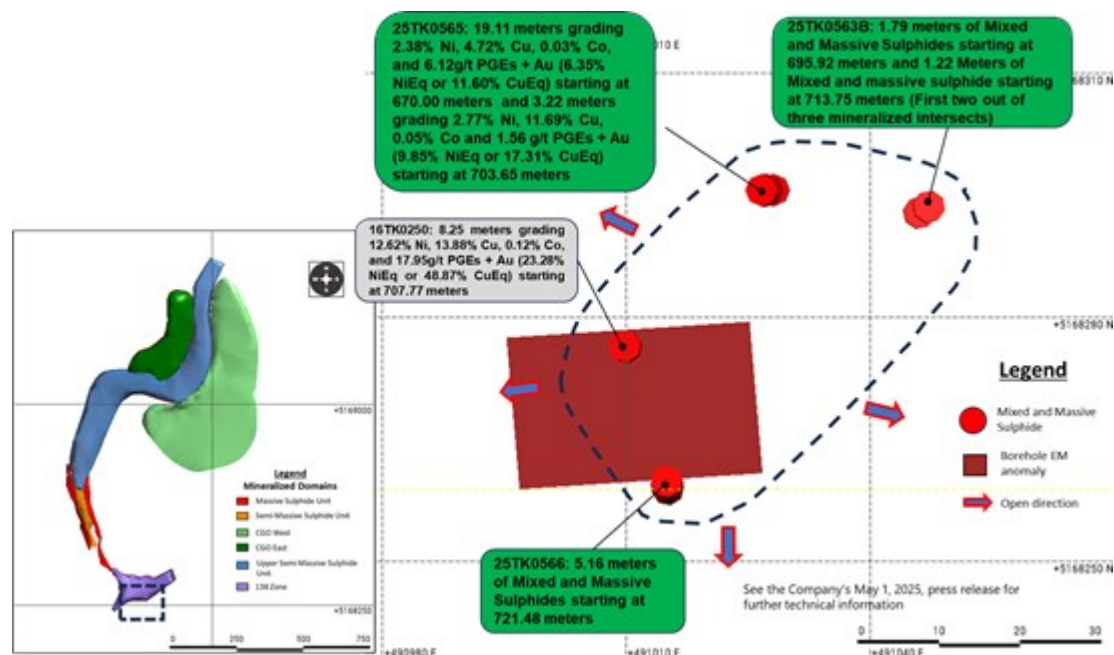
Figure 5: Plan view map of the Vault Zone at approximately 700m depth, showing the new assay results from drill hole 25TK0565 and new MMS in drill holes 25TK0566 and 25TK0563B at the same depth elevation as discovery drill hole 16TK0250
