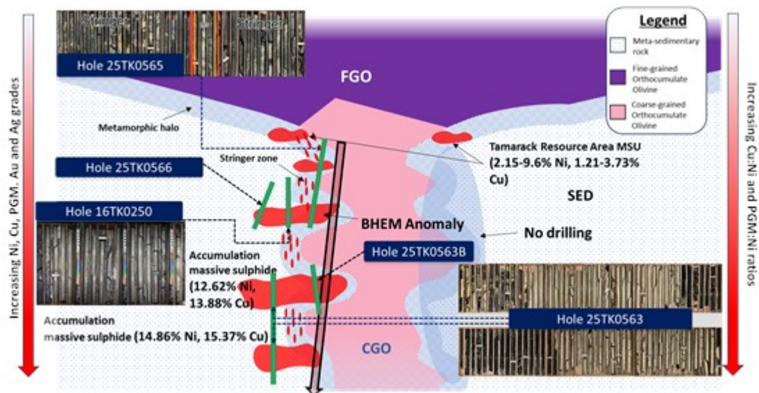
Figure 6: Conceptual cross-section through the Vault Zone showing the stack of previously intercepted high-grade nickel-copper-PGE mineralization
