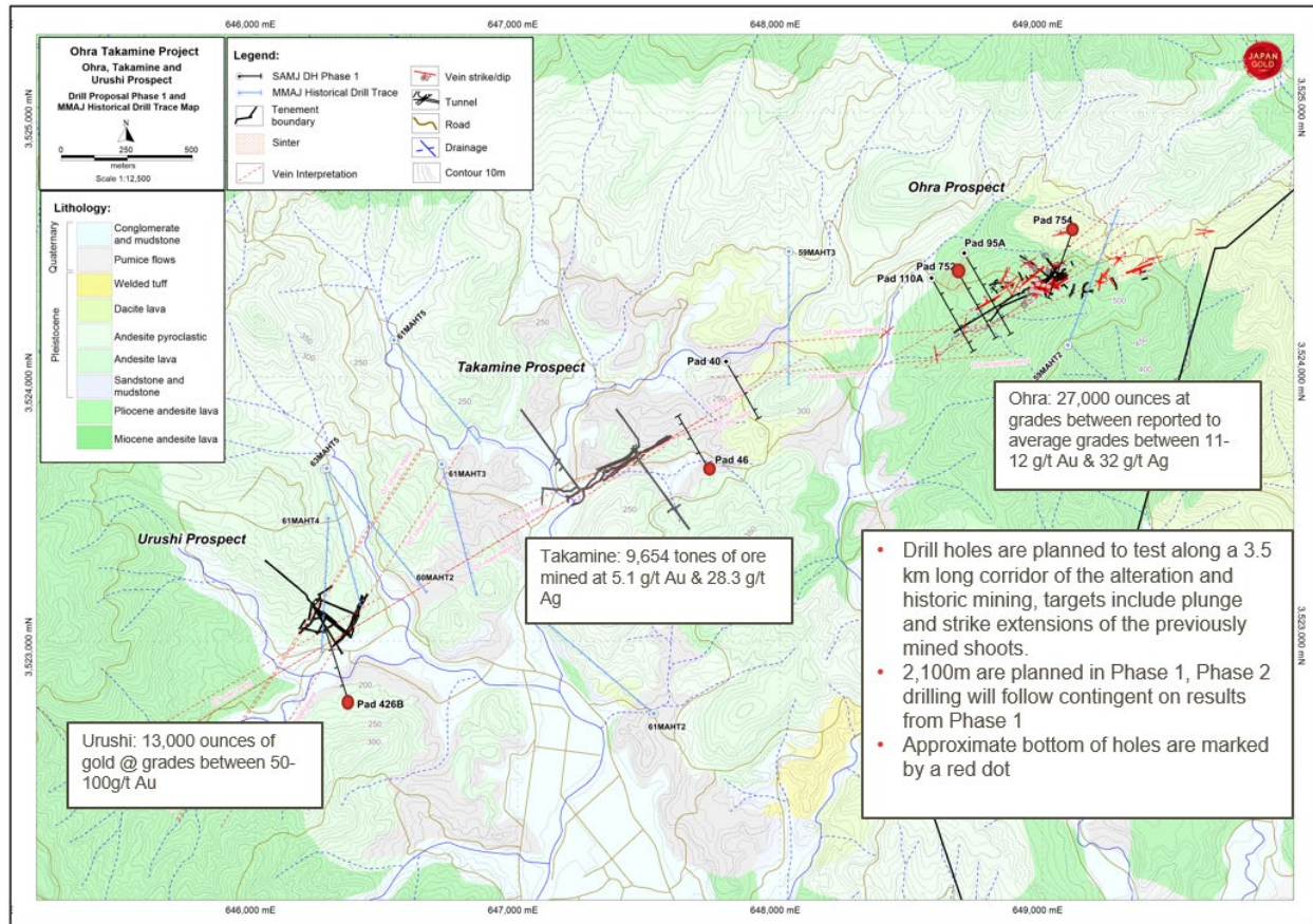
Figure 1: Ohra-Takamine Project, Phase 1 Drill Proposal Plan
