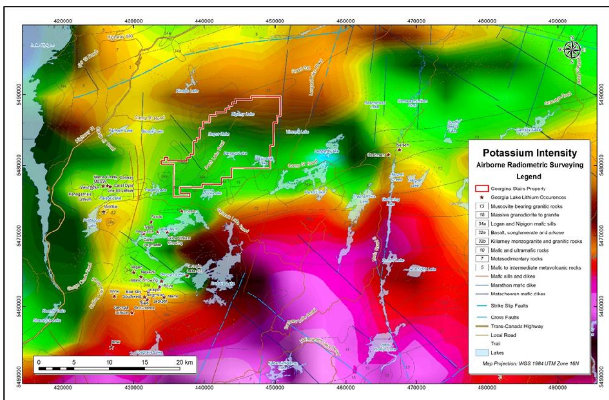
Figure 2: Regional potassium intensity from an airborne radiometric survey for Georgia Lake, Northwestern Ontario.
