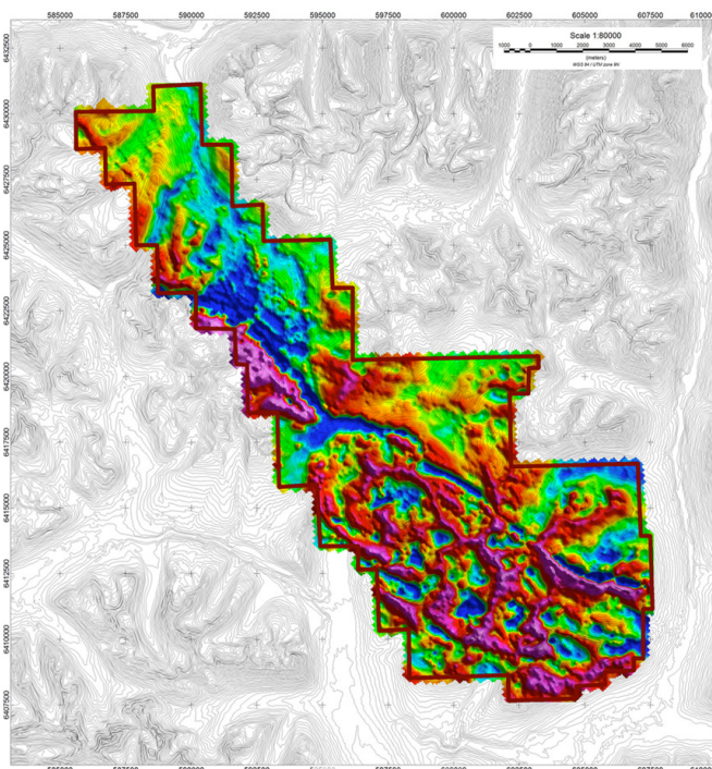
Lunar survey block calculated vertical gradient of the total magnetic intensity
